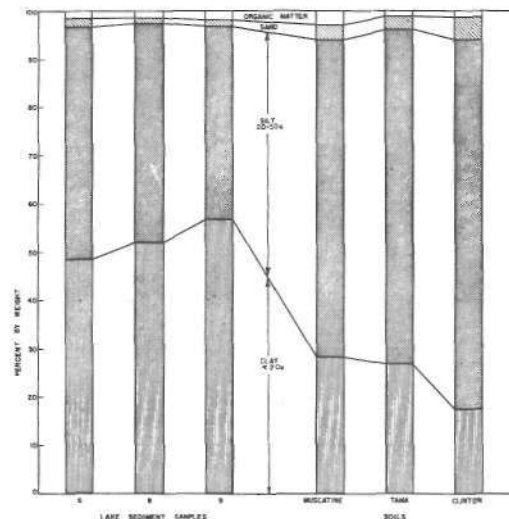
FIG. 8. COMPARISON OF SEDIMENT TEXTURE TO WATERSHED SOILS.
