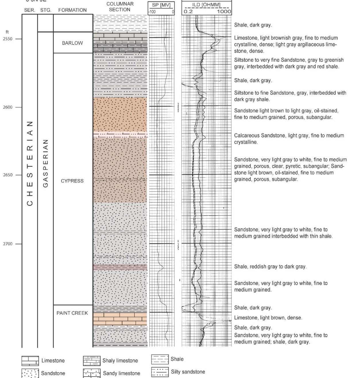
Figure 2 Stratigraphic column and electric log of Podolsky Oil Company, Foss #1 well (API 121592388700), Section 8, T3N, R9E, in Noble Field, Richland County, showing lithologic units of the interval studied, lithologic column, and description of well samples. Sample studies indicate oil stained sandstone below the producing oil-water contact.
