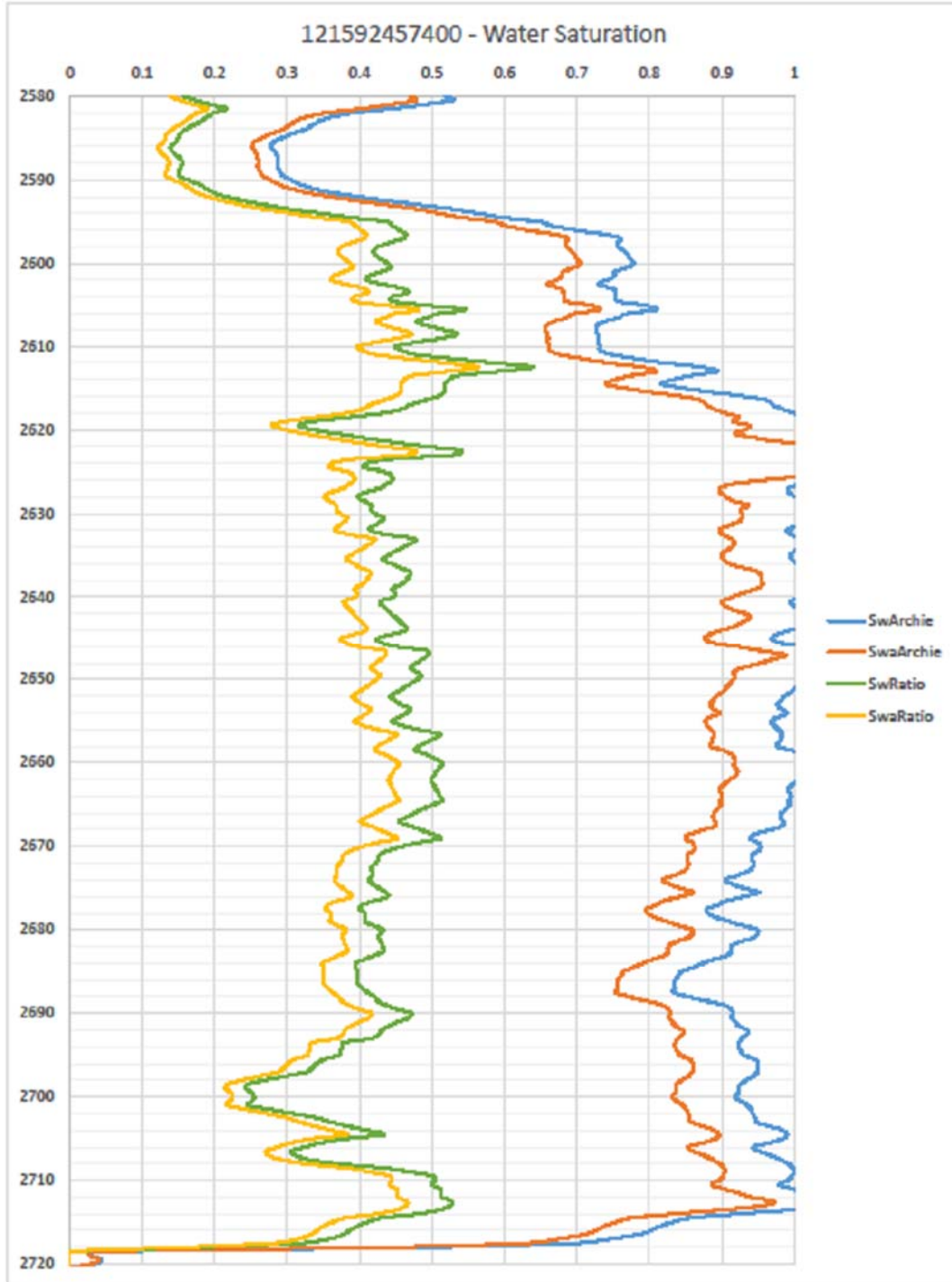
Figure 1 Preliminary results from petrophysical analysis of the Bourne #5 well (API 121592457400) using the ratio water saturation and Archie water saturation methods. The disparity between the water saturation curves may indicate microporosity within the thick Cypress Sandstone, which will require petrographic analysis to confirm. The y-axis is depth in feet and the x-axis is the ratio value.
