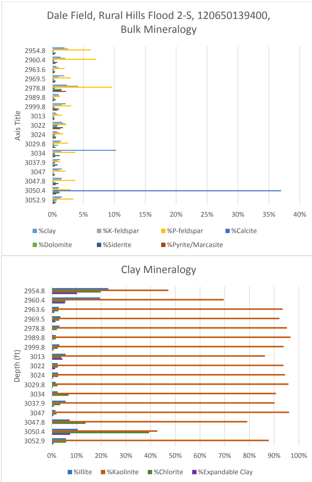
Figure 4 Example results of bulk mineralogy (with quartz omitted to show minor constituents) and clay mineralogical analysis from the Rural Hills Flood 2-S well (API 120650139400) showing total bulk mineralogy (above) and the relative abundance of clay minerals within the clay fraction (below).
