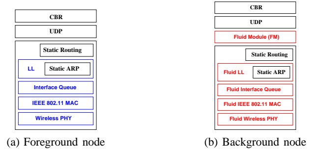
Fig. 7. Protocol stacks for packet level simulation and fluid model based simulation.
