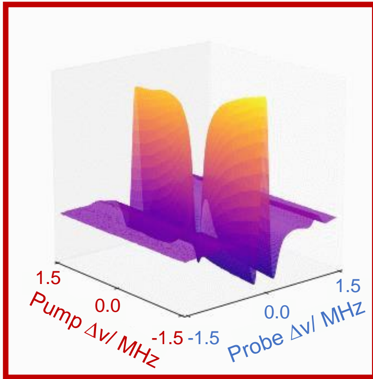
Autler-Townes splitting
