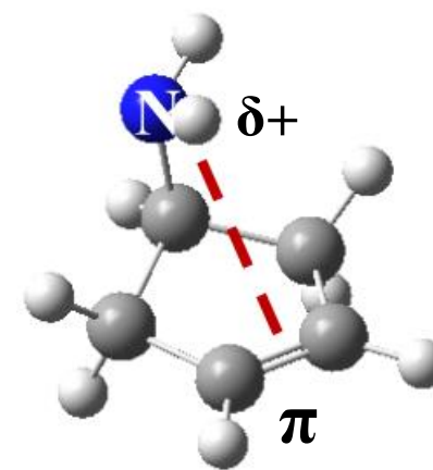
3-cyclopenten-1-amine
