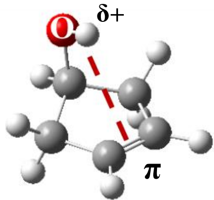
3-cyclopenten-1-ol
