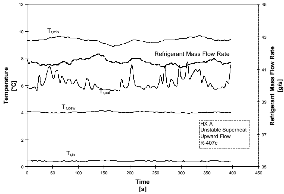
Figure 6.4 Unstable operation of evaporator (R-407c)
