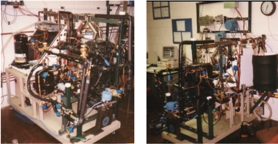
Figure C.12 Photographs of experimental facility (front and back)
