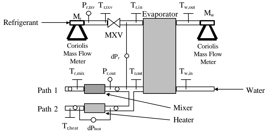
Figure 3.3 Test section during Experiment 5-6
