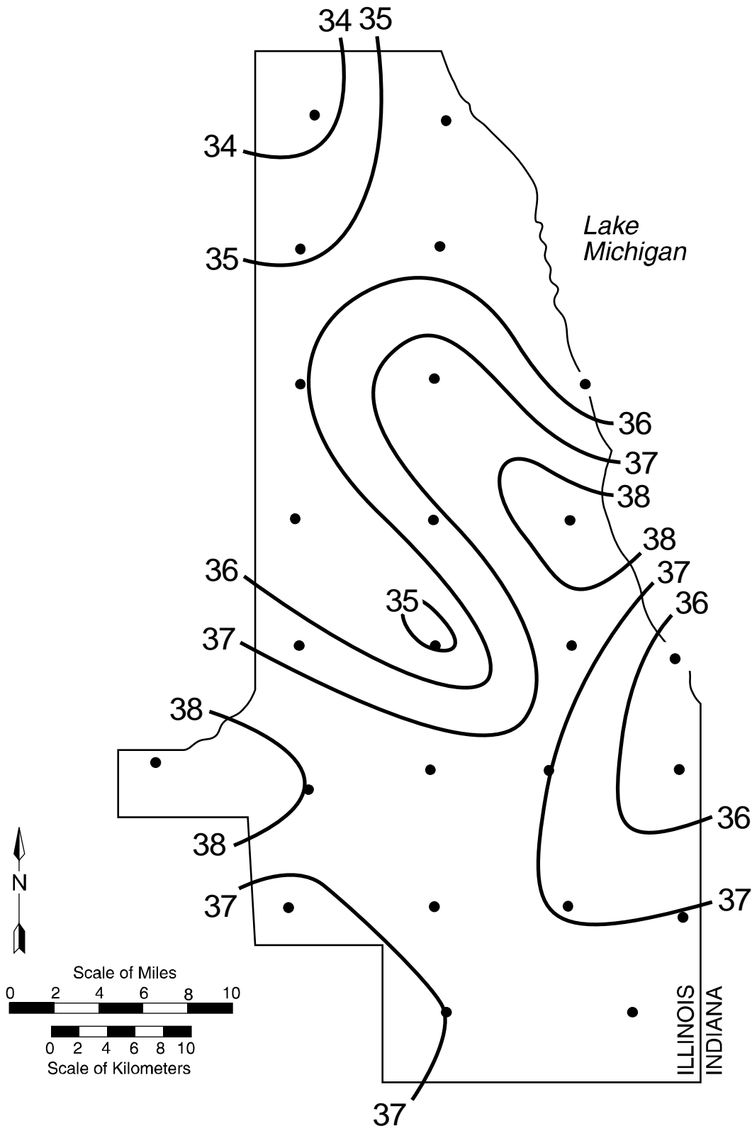
Figure 6. Twenty-year average precipitation pattern (inches), Water Years 1990–2009
