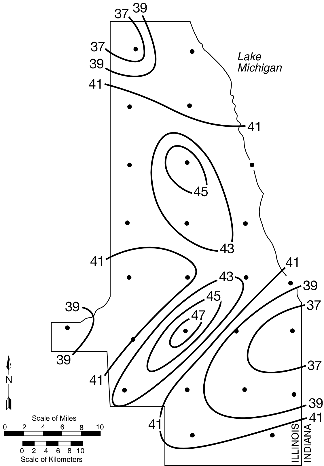
Figure 3. Precipitation pattern (inches) for Water Year 2009
