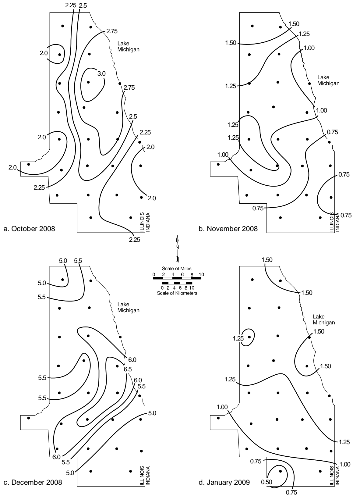
Figure 5. Precipitation pattern (inches) for October 2008–September 2009
