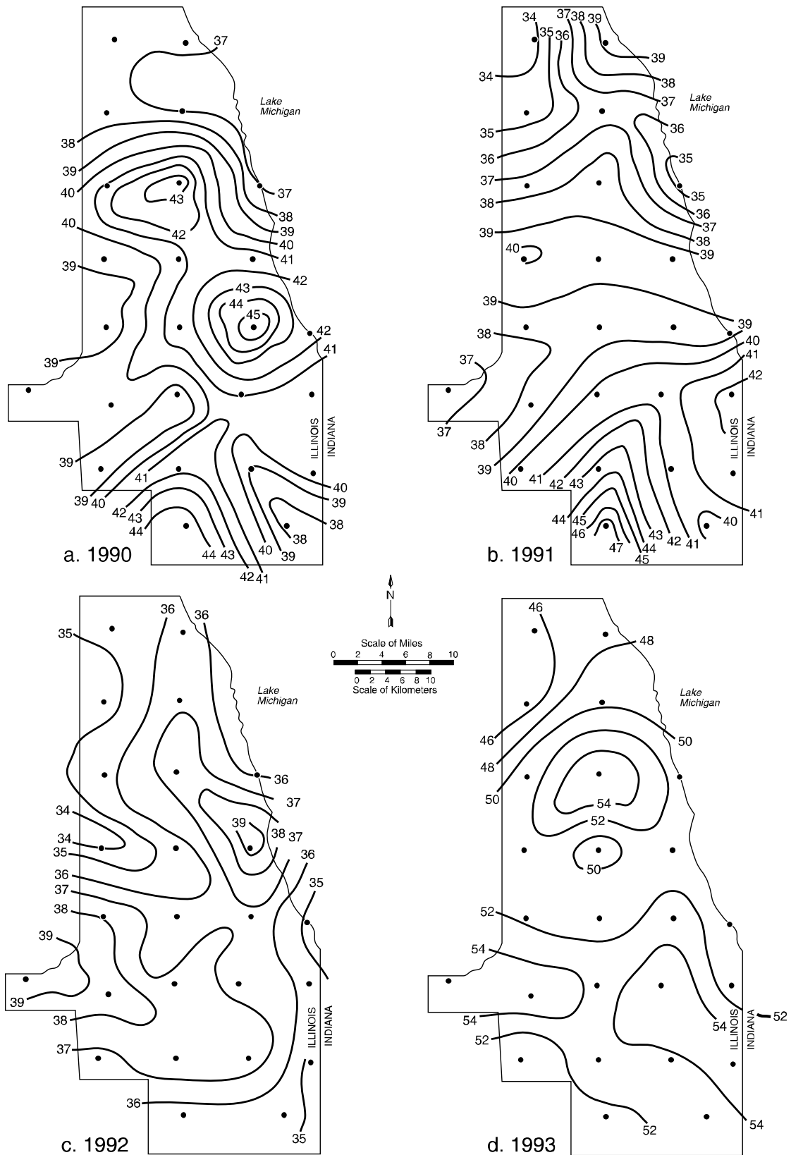
Figure 4. Precipitation pattern (inches) for Water Years 1990–2008
