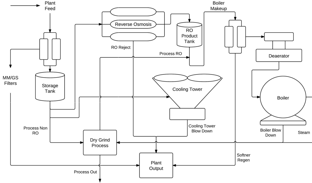
Figure 1.1: Water routing in Dry Grind Ethanol plant.
