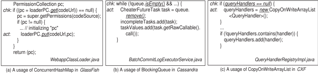
Figure 1. Three instances of misused CHECK-THEN-ACT idioms of concurrent collections used in real-world applications.
