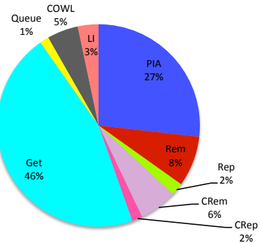
(b) The distribution of correct idioms. The total number is 545.
