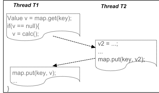
Figure 3. An example of buggy interleaving for Fig. 2(a)
