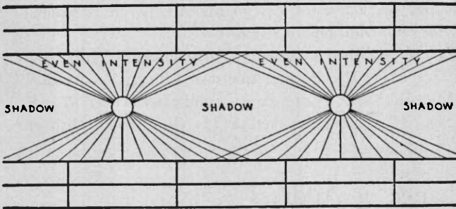
End view of aisle (above), showing how Snead Reflector distributes light of an even intensity on upper and lower shelves. Diagram below shows top view of aisle. Note even light distribution along aisle and absence of glare.
