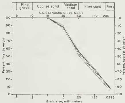
Figure 10. Particle-size distributions of spiral feed. Each line represents a separate spiral sample.
