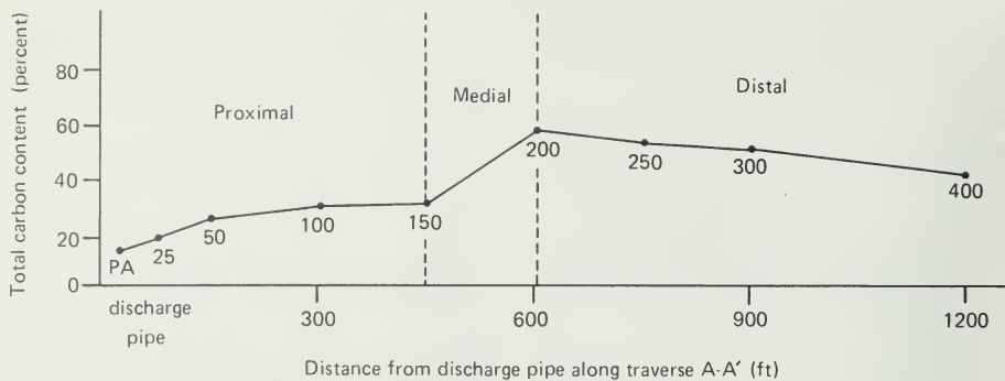
Figure 4. Trend in carbon content along traverse A-A'.
