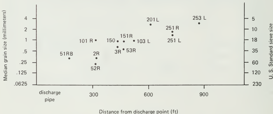
Figure 2. Increase in slurry particle size with increasing distance from the discharge pipe.
