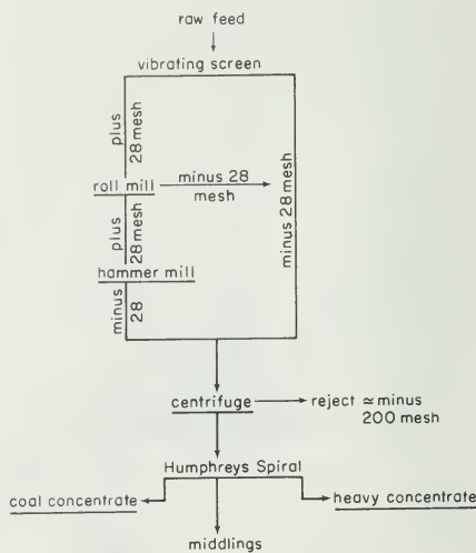
Figure 8. Flowsheet of raw slurry preparation and spiral concentration.
