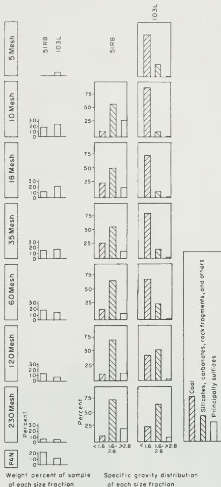
Figure 3. Particle-size and specific gravity distributions of two selected slurry samples.
