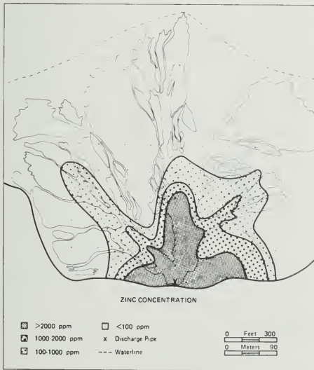
Figure 6. Zinc concentration in the slurry deposit.
