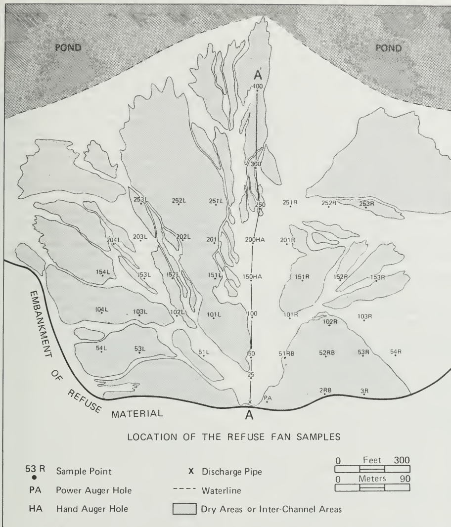
Figure 1. Plan view of slurry deposit and location of samples.
