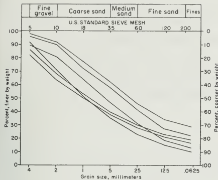
Figure 9. Particle-size distributions of raw slurry samples selected for spiral tests. Each line represents a separate slurry sample.
