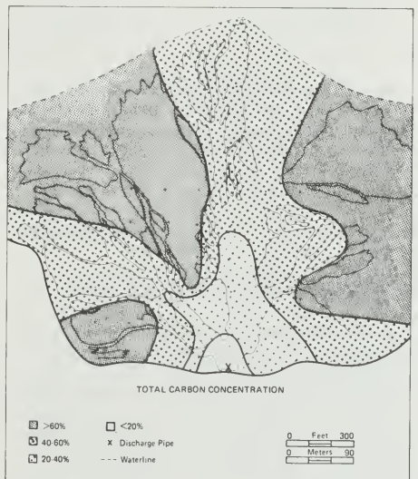
Figure 7. Carbon concentration in the slurry deposit.
