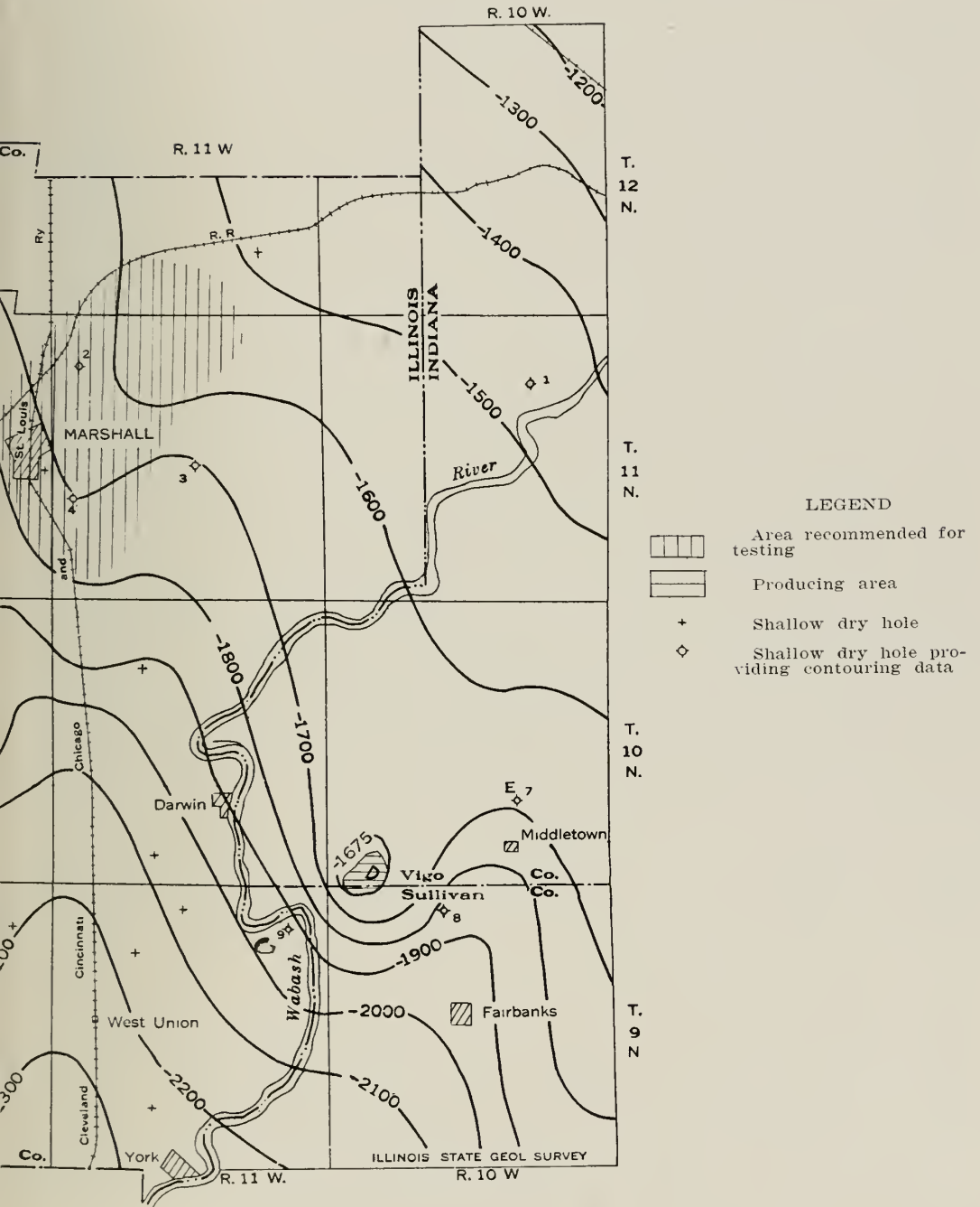
County and adjoining area, showing the locations of dry holes
