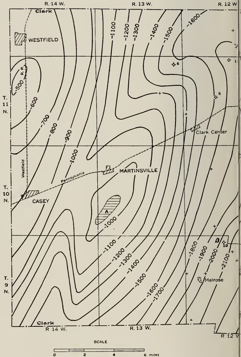
FIG. 3. Structure map of the top of the Devonian limestone in Clark
