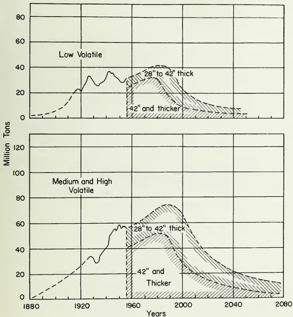
Fig. 13 - Projected production of major coking coals by thickness of beds .
