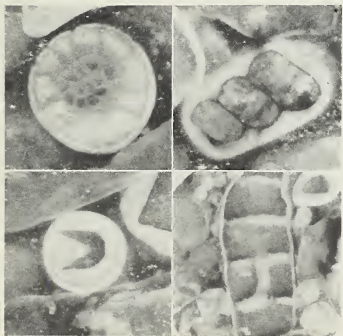
FIG. 2.—Oolites with recognizable fossil centers.
