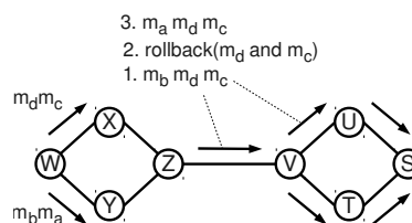
Figure 3: Example: rolling back across nodes.
