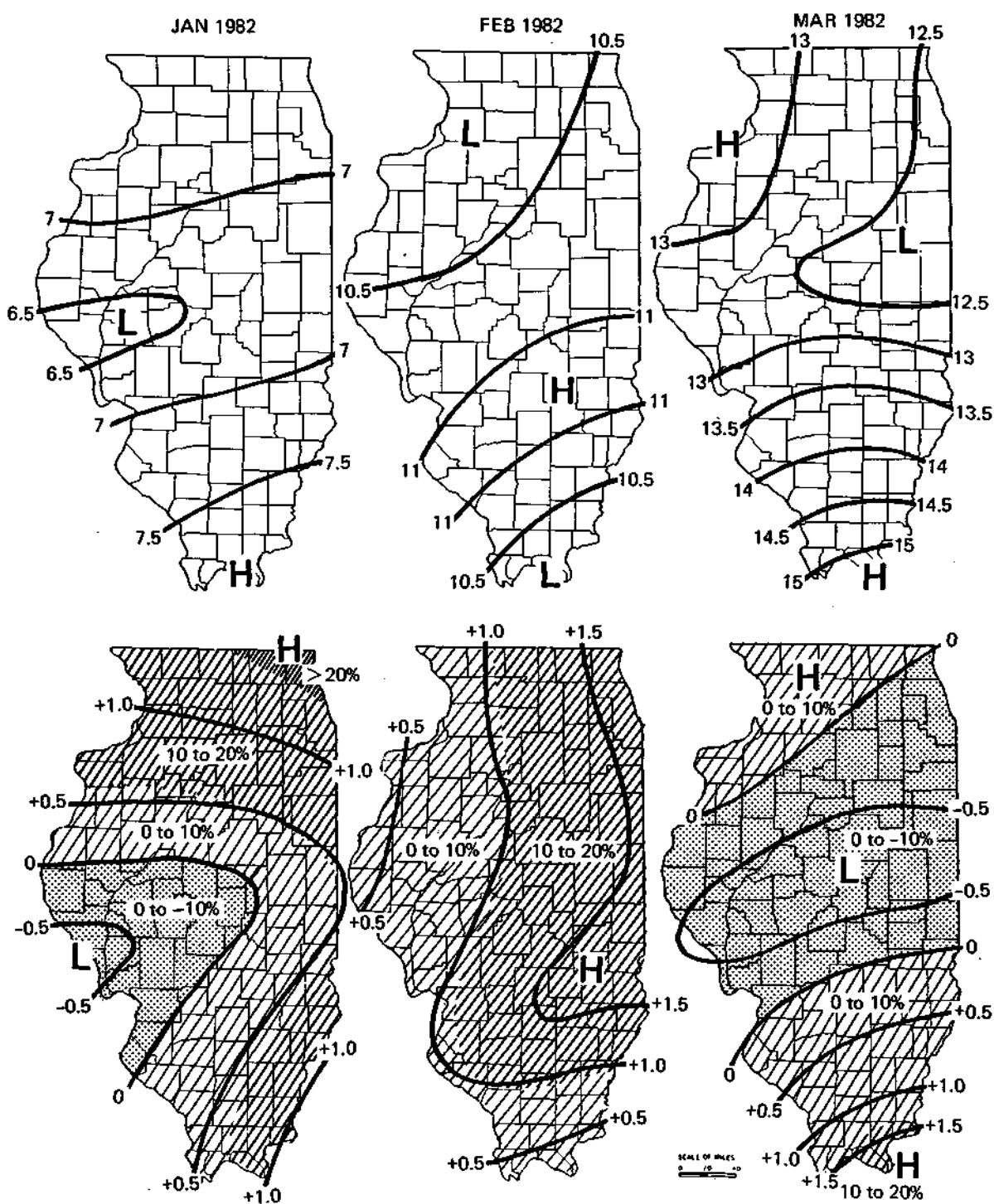
Figure 4. Upper; Distribution of monthly values of mean daily incoming solar radiation (MJ m -2 ) for January-March 1982.
