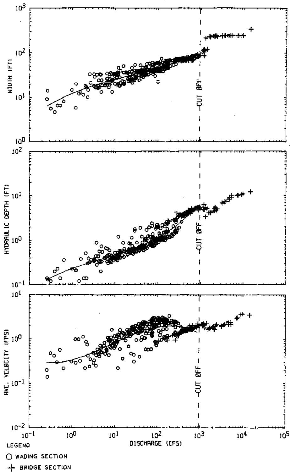
Figure 8. Station hydraulic geometry, Sangamon River at Mahomet
