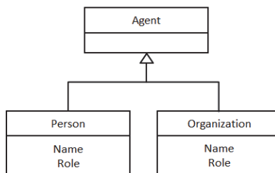
Figure 6: Agent Entities
