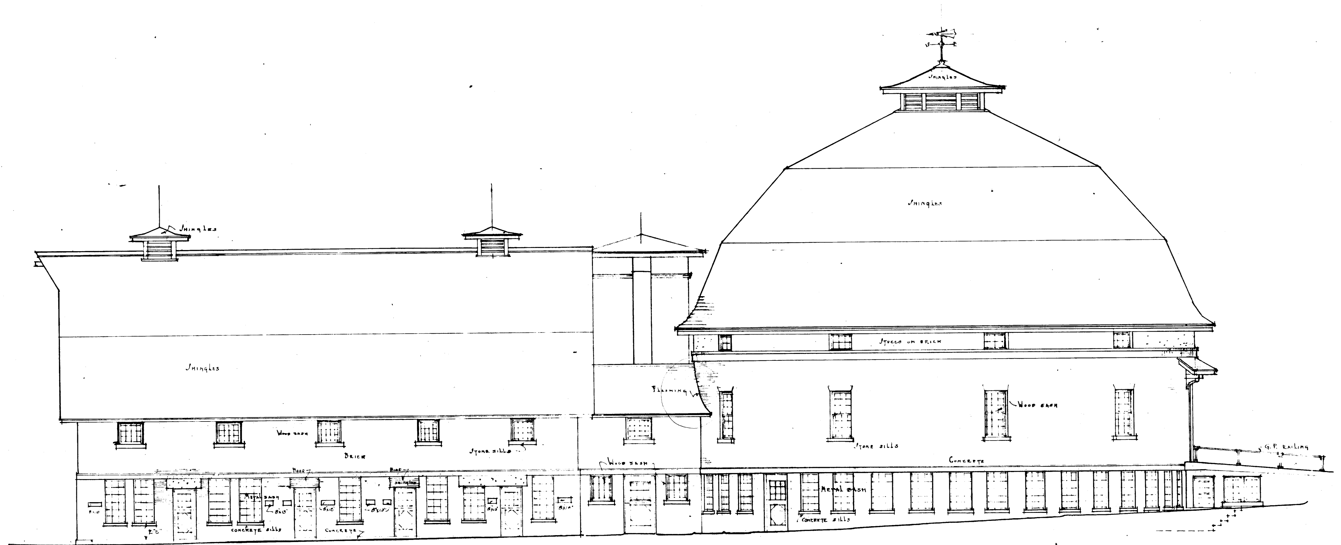
• SOUTH - EAST - ELEVATION • Scale \frac{1}{8}'' = 1'-0''
