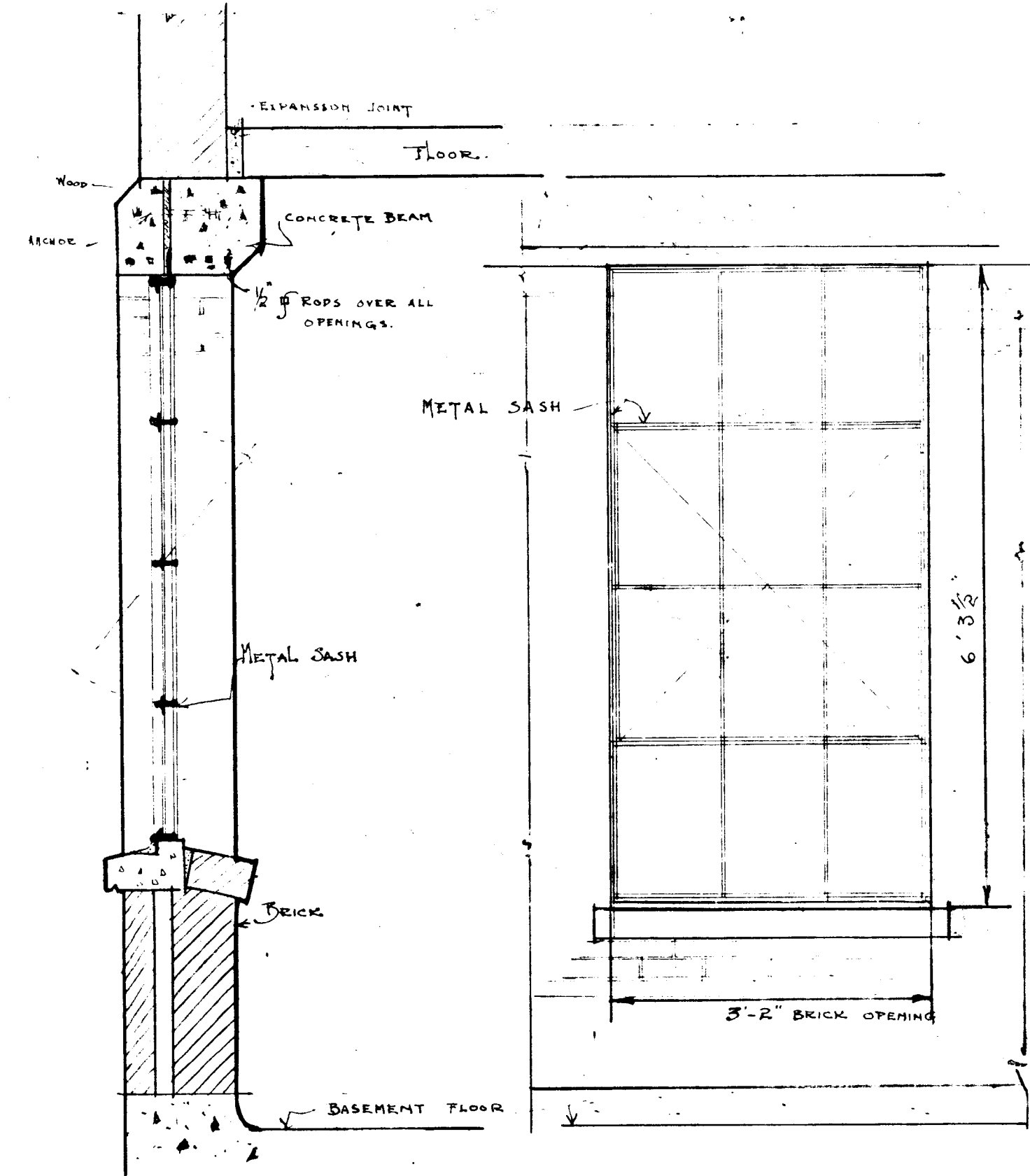
INSIDE ELEVATION OF WINDOWS IN RECTANGULAR BARN 3/4 scale.
