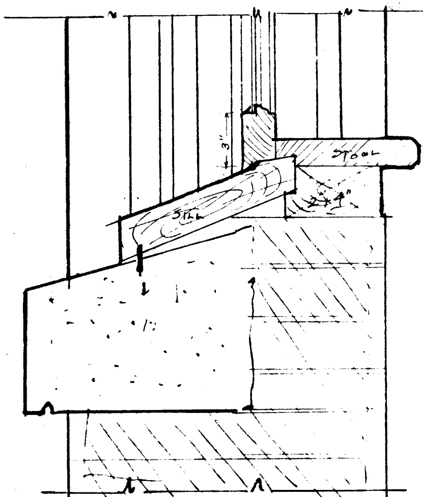
SECTION THRO SILL
