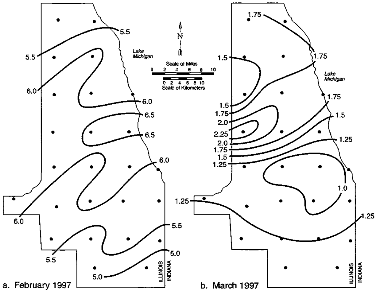
Figure 7. Precipitation pattern (inches) for a) February 1997, and b) March 1997
