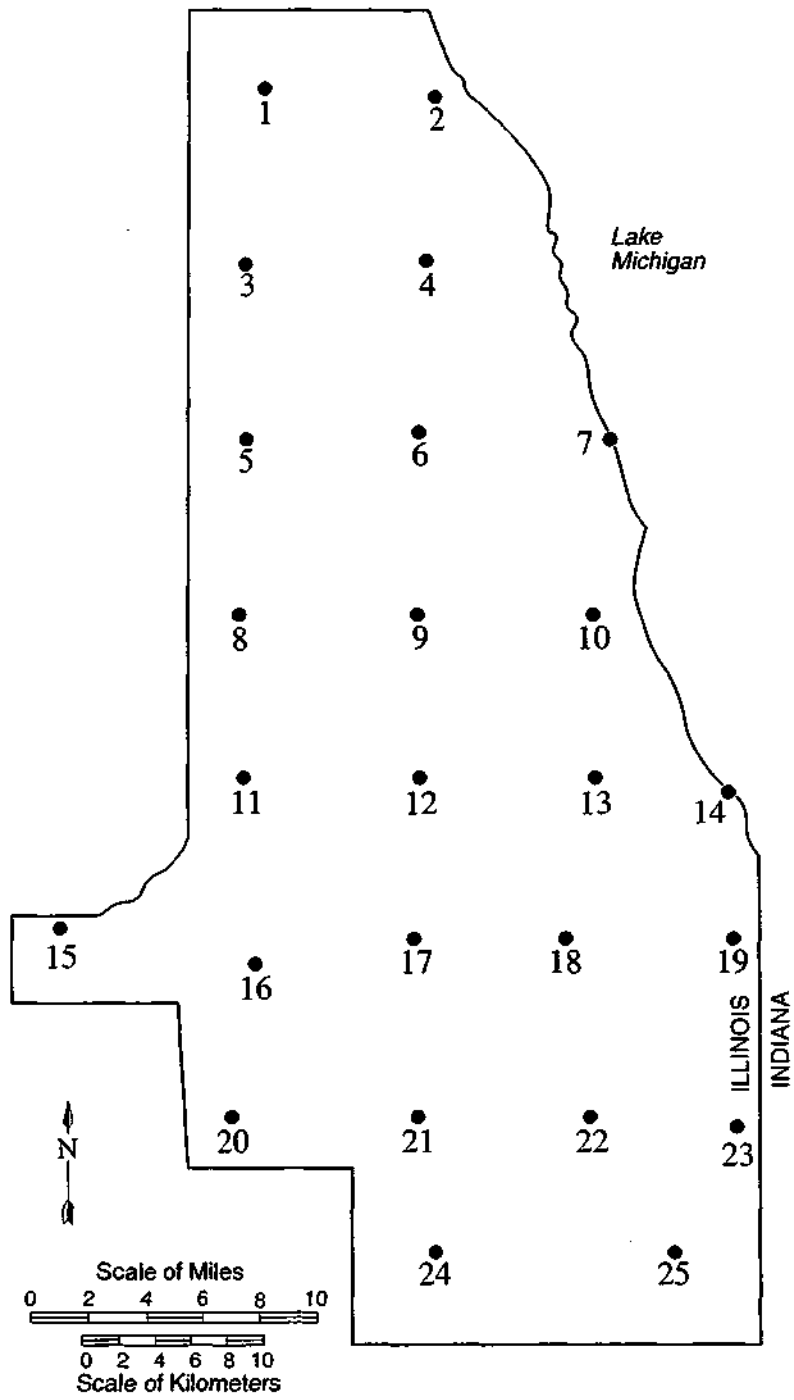
Figure 2. The 25-site raingage network used during Water Years 1990 to 1997
