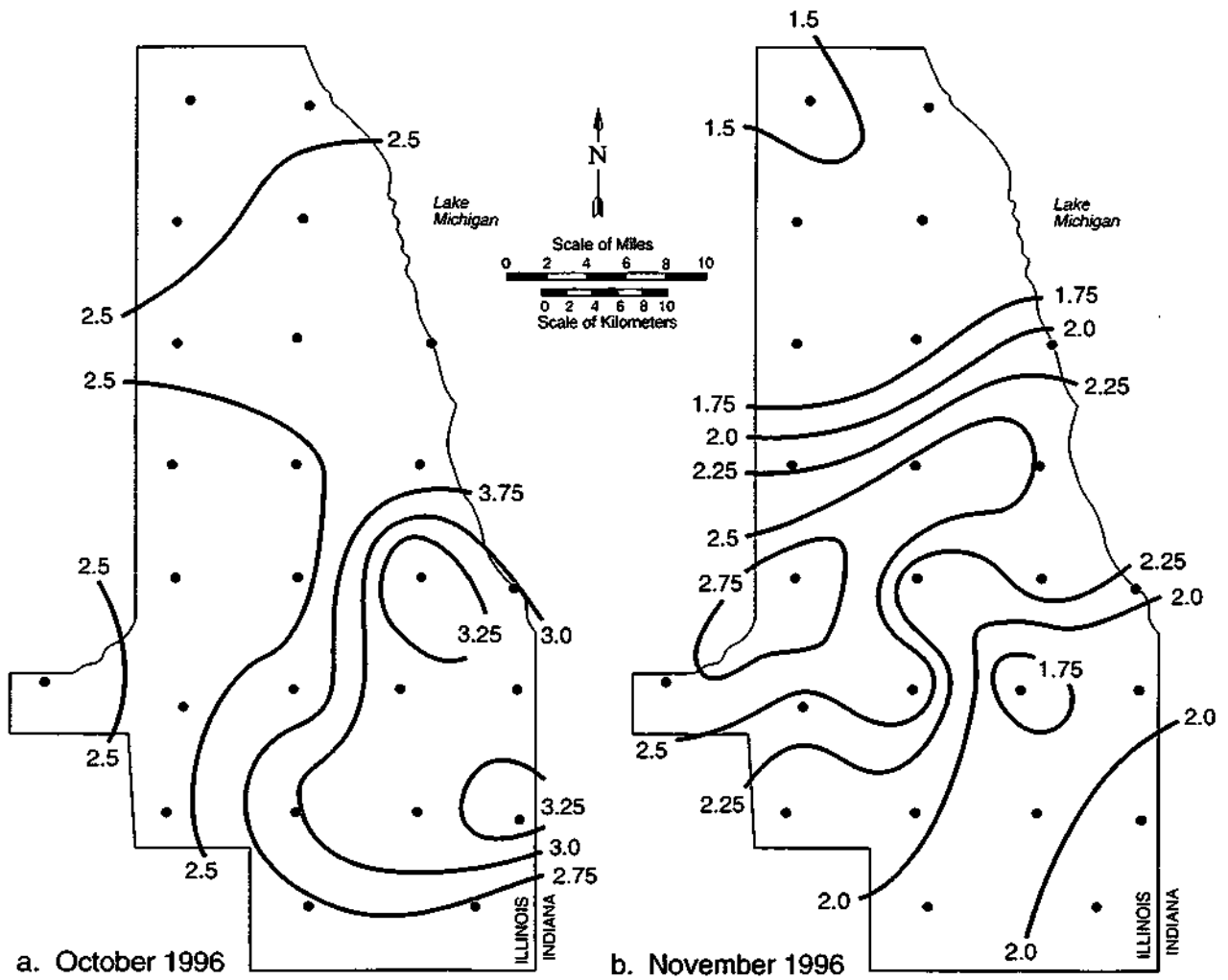
Figure 5. Precipitation pattern (inches) for a) October 1996, and b) November 1996
