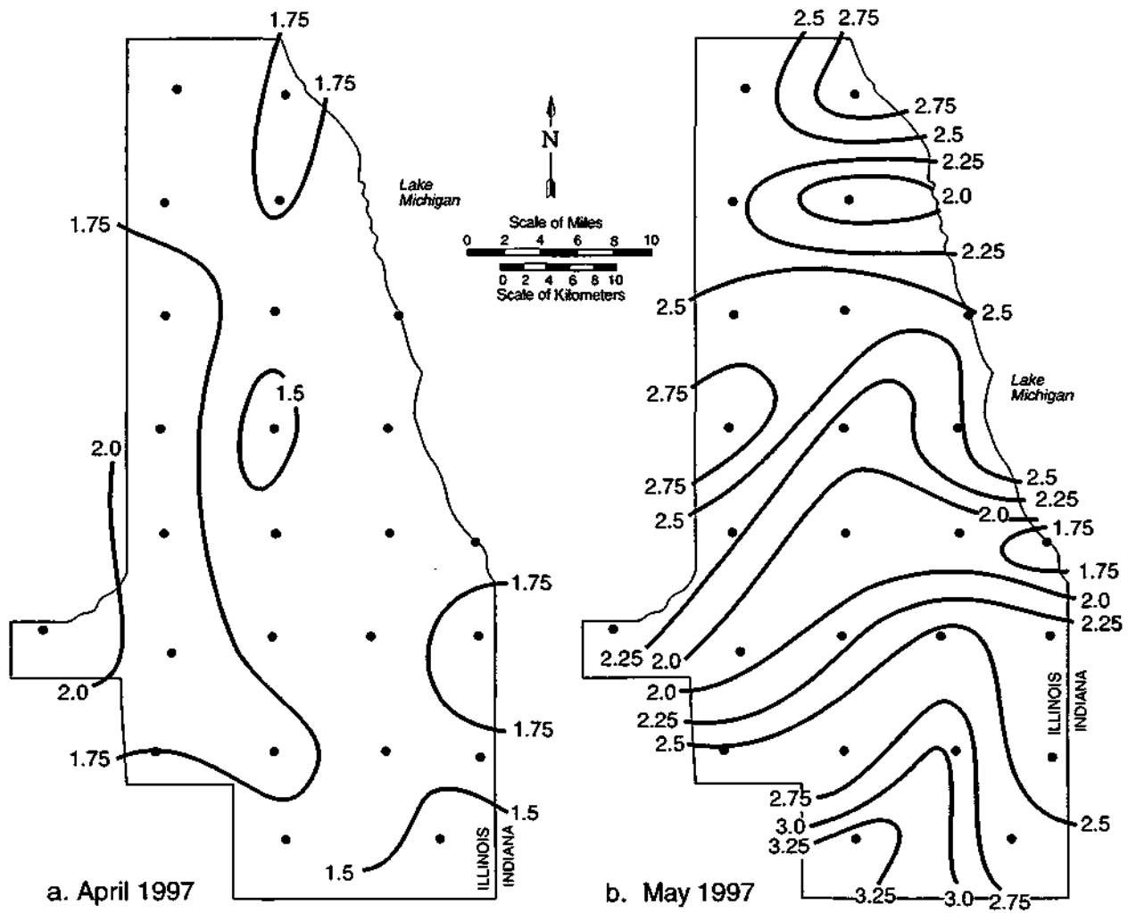
Figure 8. Precipitation pattern (inches) for a) April 1997, and b) May 1997
