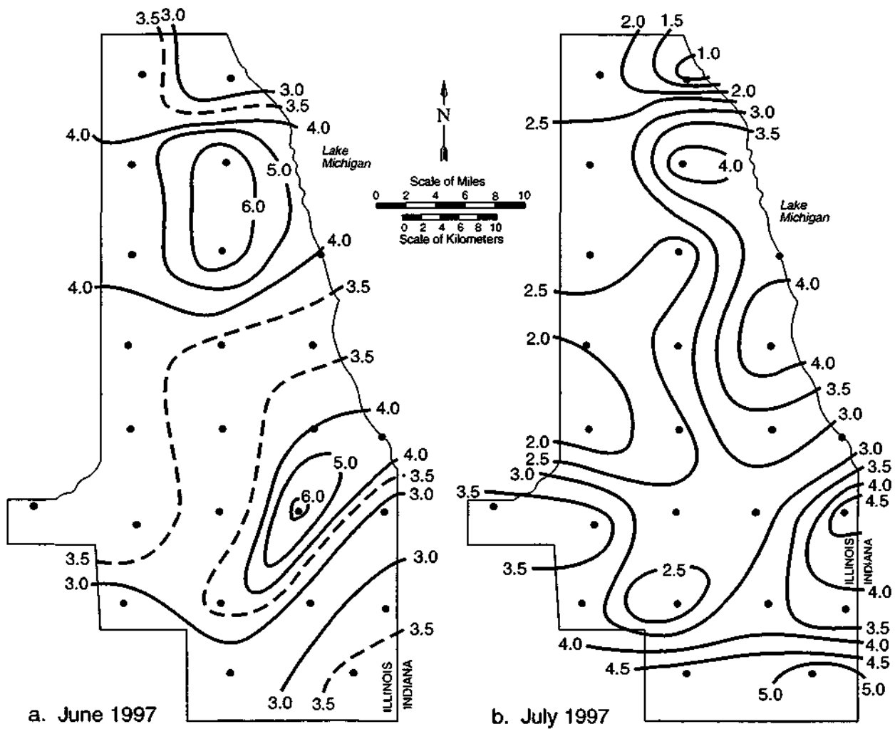
Figure 9. Precipitation pattern (inches) for a) June 1997, and b) July 1997
