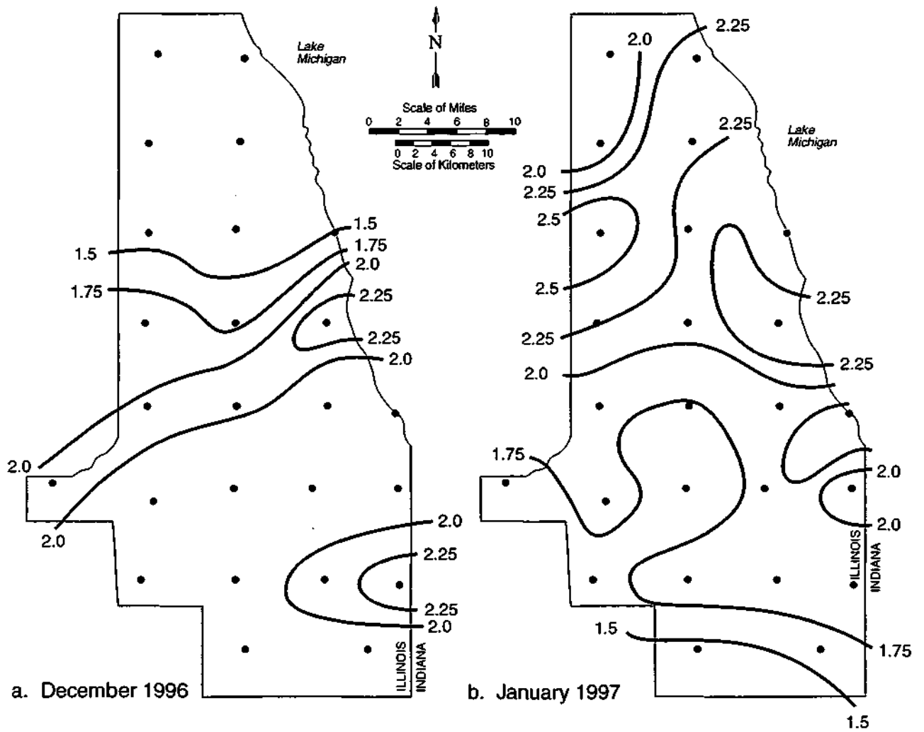
Figure 6. Precipitation pattern (inches) for a) December 1996, and b) January 1997
