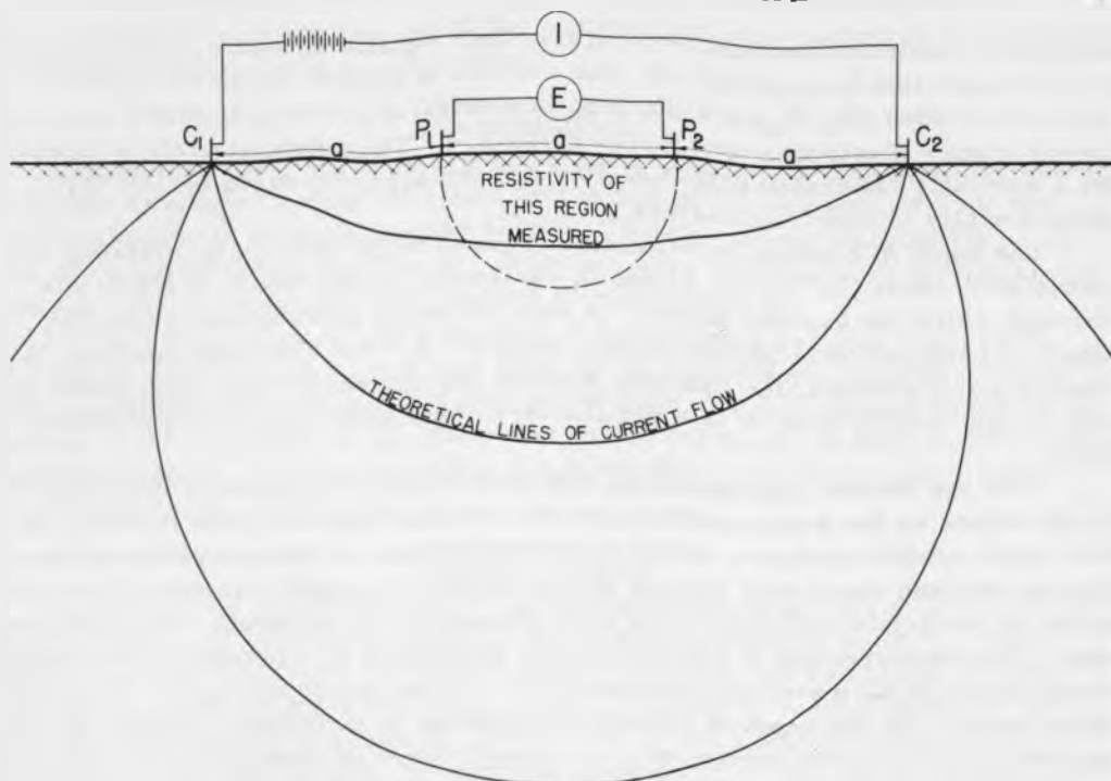
Fig. 2. - Wenner four-electrode configuration.
