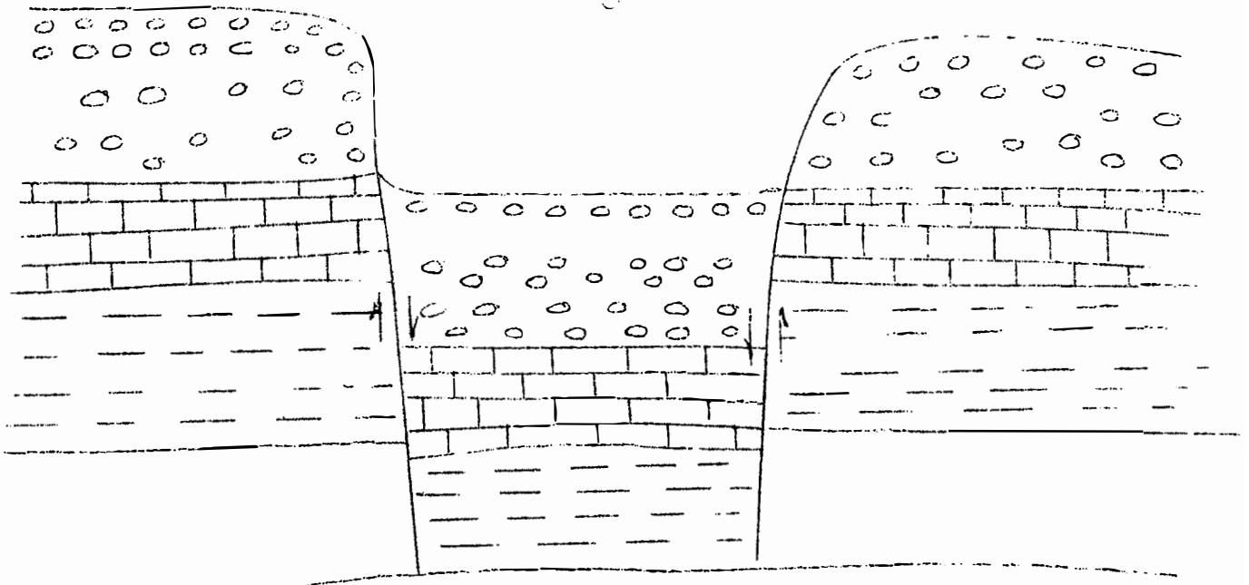
Generalized diagram of the Rock Creek Graben, before erosion
