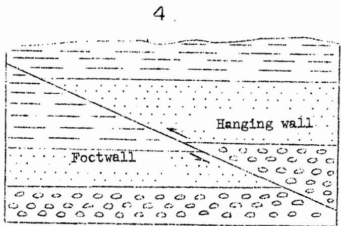
Thrust fault
