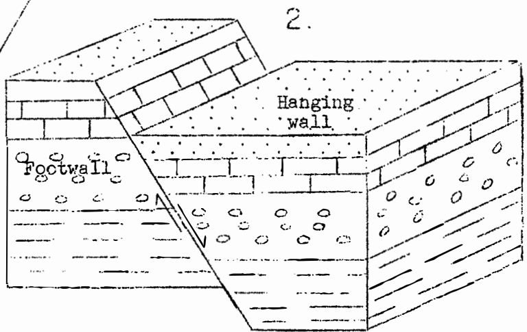
Normal or gravity fault
