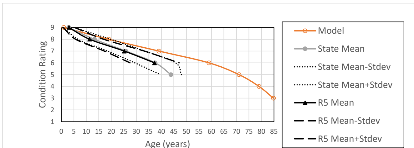
Figure 27. Chart. Culvert with fill equal to or greater than 2 feet deterioration curves: model vs state vs Region 5.
