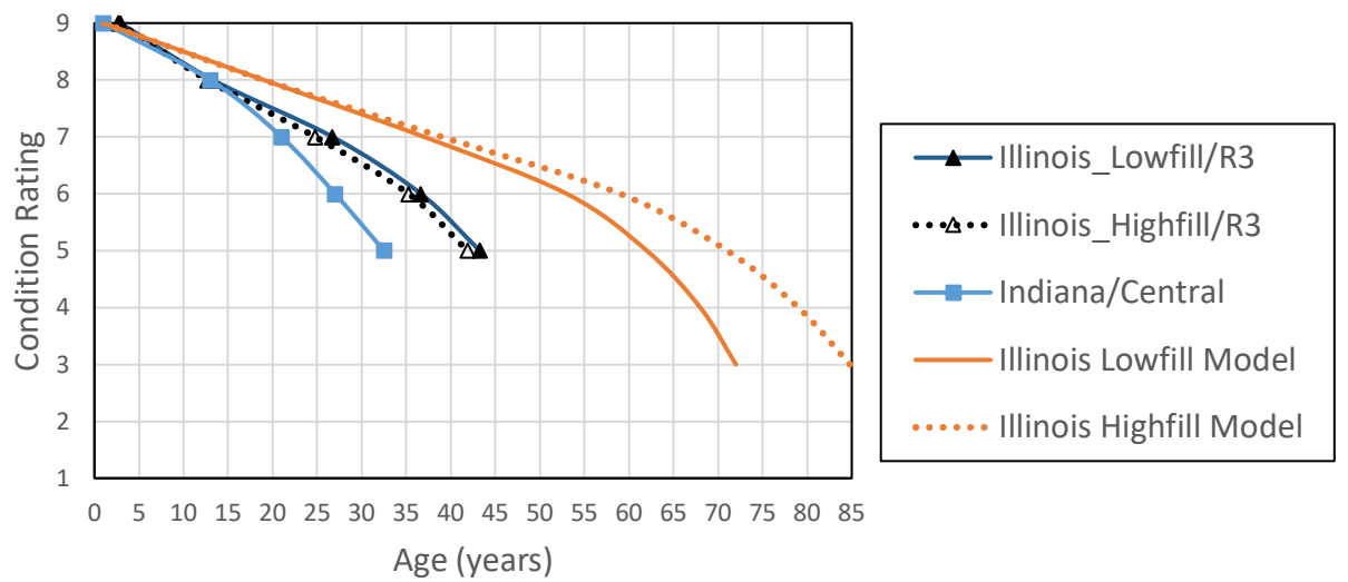
Figure 43. Chart. Illinois Region 3 vs Indiana Central: Culvert.
