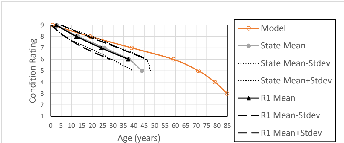
Figure 23. Chart. Culvert with fill equal to or greater than 2 feet deterioration curves: model vs state vs Region 1.
