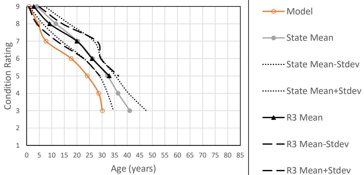
Figure 30. Chart. Deck beam deterioration curves: model vs state vs Region 3.
