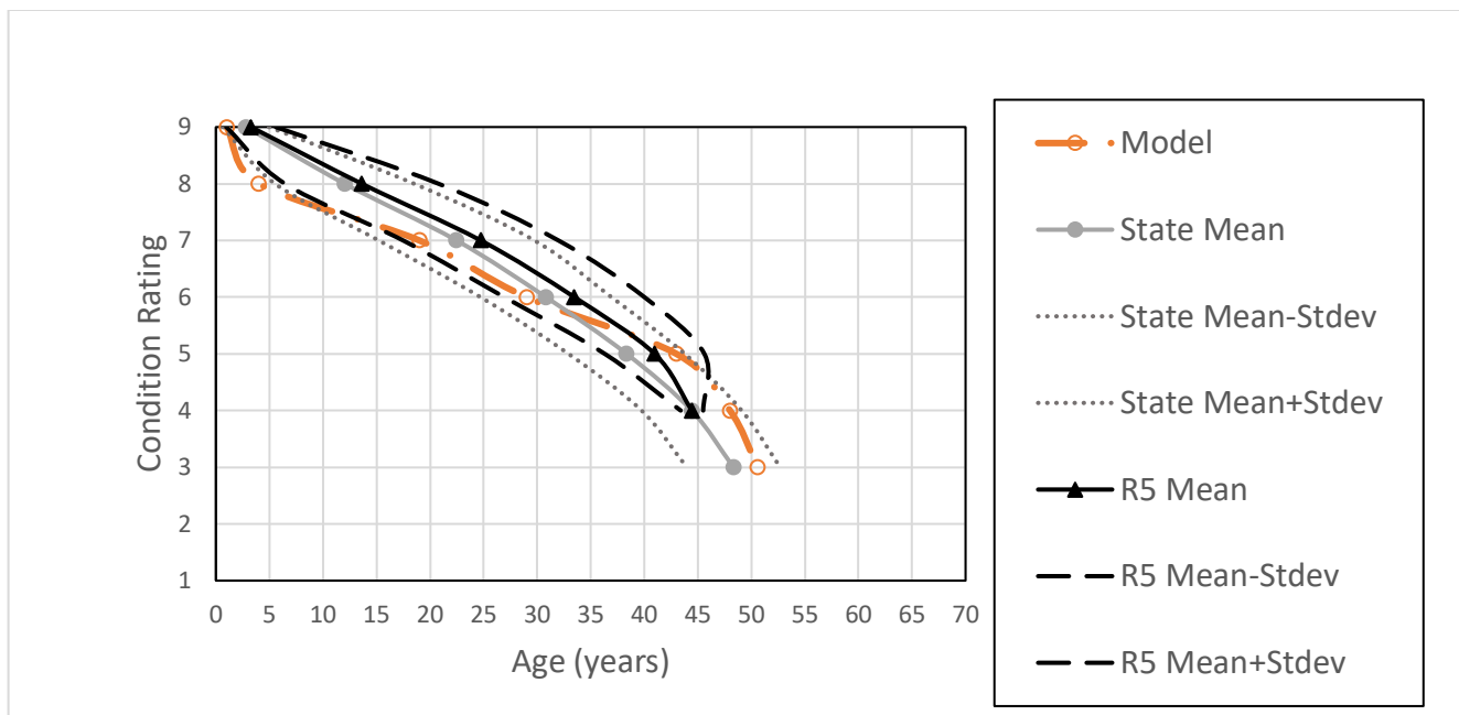
Figure 7. Chart. Deck deterioration curves: model vs state vs Region 5.
