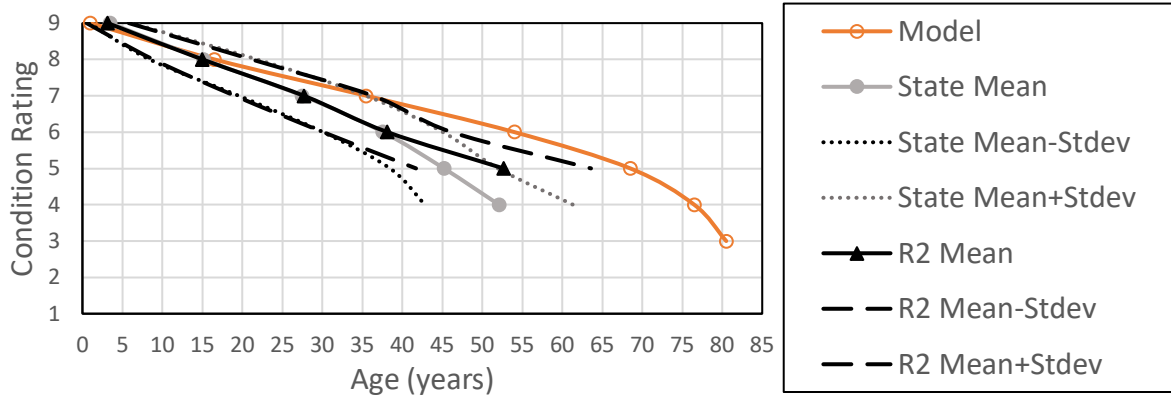
Figure 14. Chart. Substructure deterioration curves: model vs state vs Region 2.
