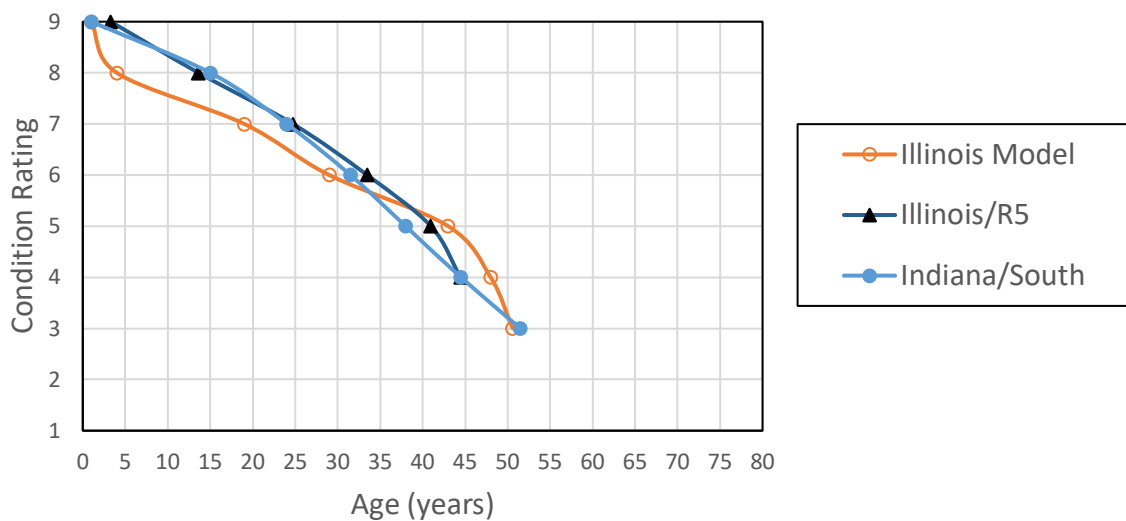
Figure 35. Chart. Illinois Region 5 vs Indiana South: Deck.
