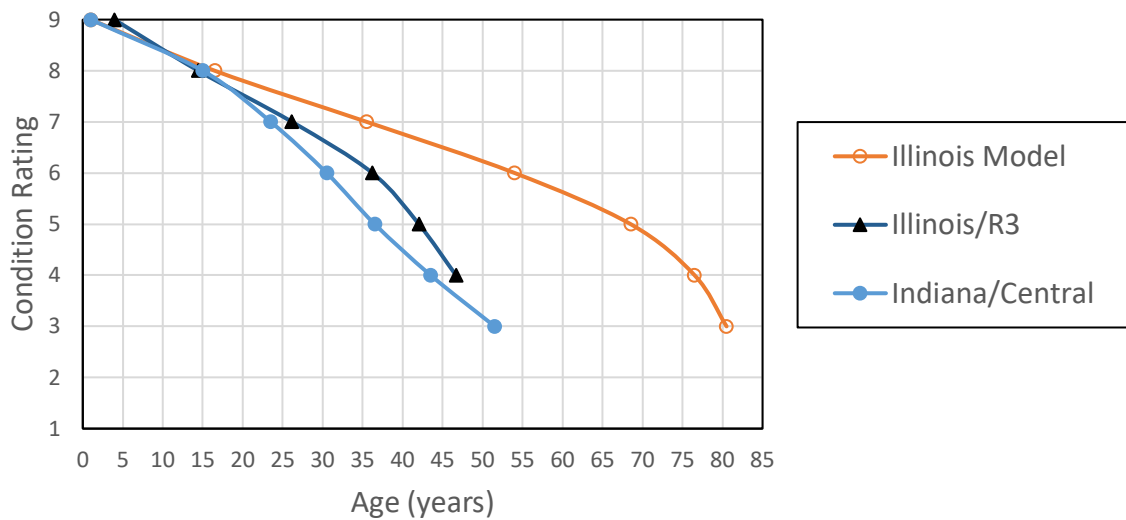
Figure 40. Chart. Illinois Region 3 vs Indiana Central: Substructure.
