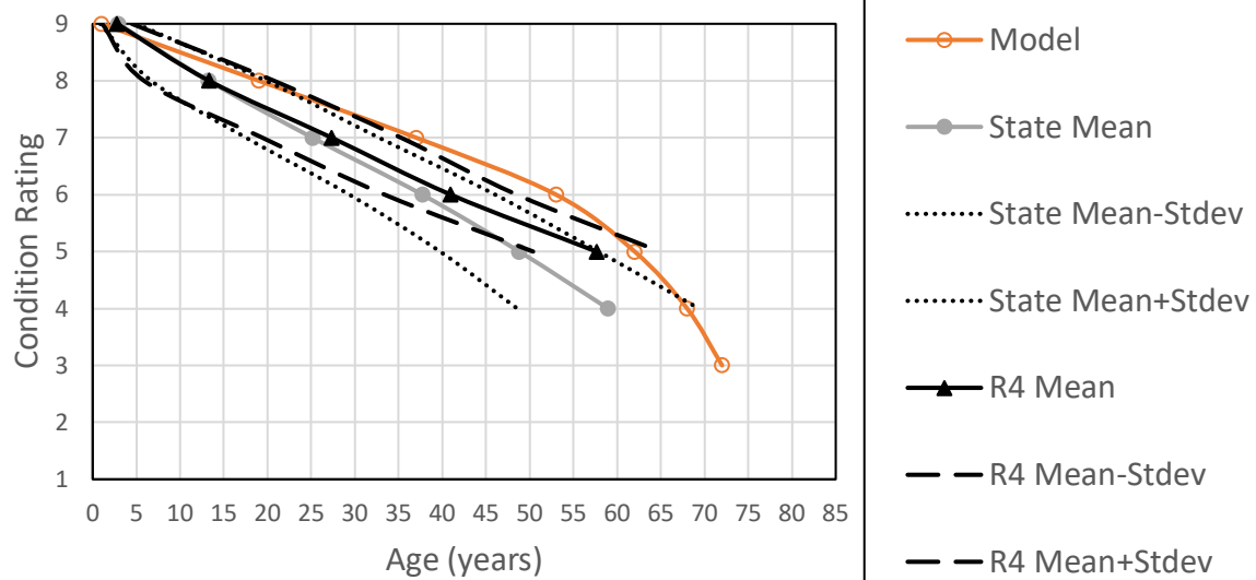
Figure 21. Chart. Culvert with fill less than 2 feet deterioration curves: model vs state vs Region 4.
