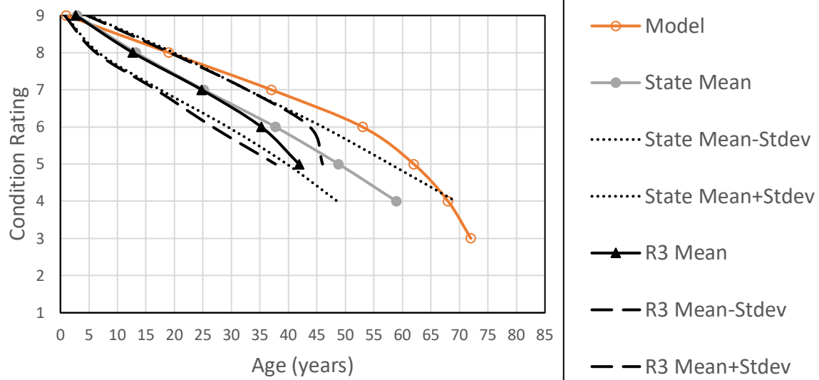
Figure 20. Chart. Culvert with fill less than 2 feet deterioration curves: model vs state vs Region 3.
