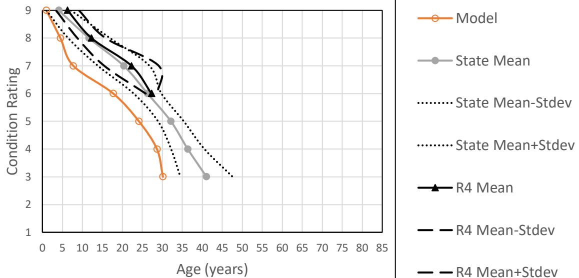
Figure 31. Chart. Deck beam deterioration curves: model vs state vs Region 4.
