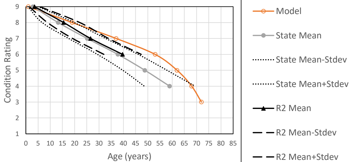
Figure 19. Chart. Culvert with fill less than 2 feet deterioration curves: model vs state vs Region 2.
