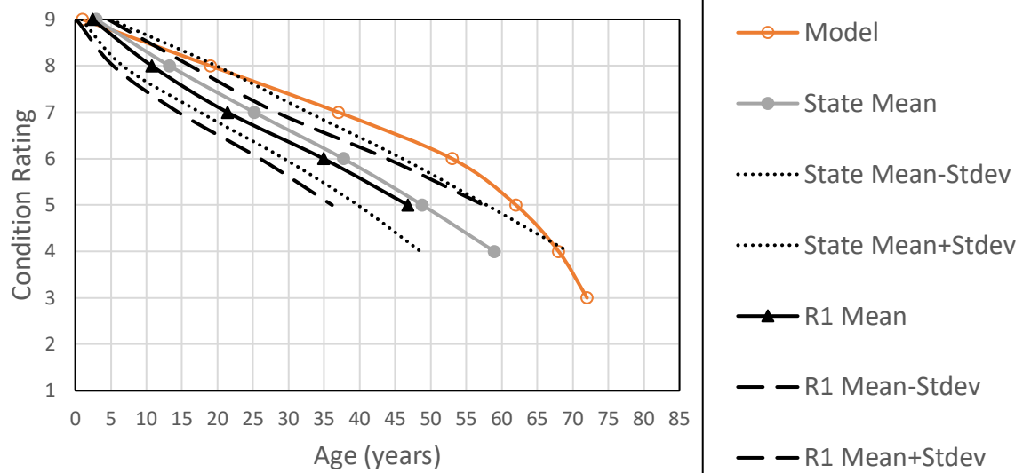
Figure 18. Chart. Culvert with fill less than 2 feet deterioration curves: model vs state vs Region 1.
