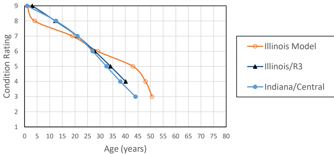
Figure 34. Chart. Illinois Region 3 vs Indiana Central: Deck.
