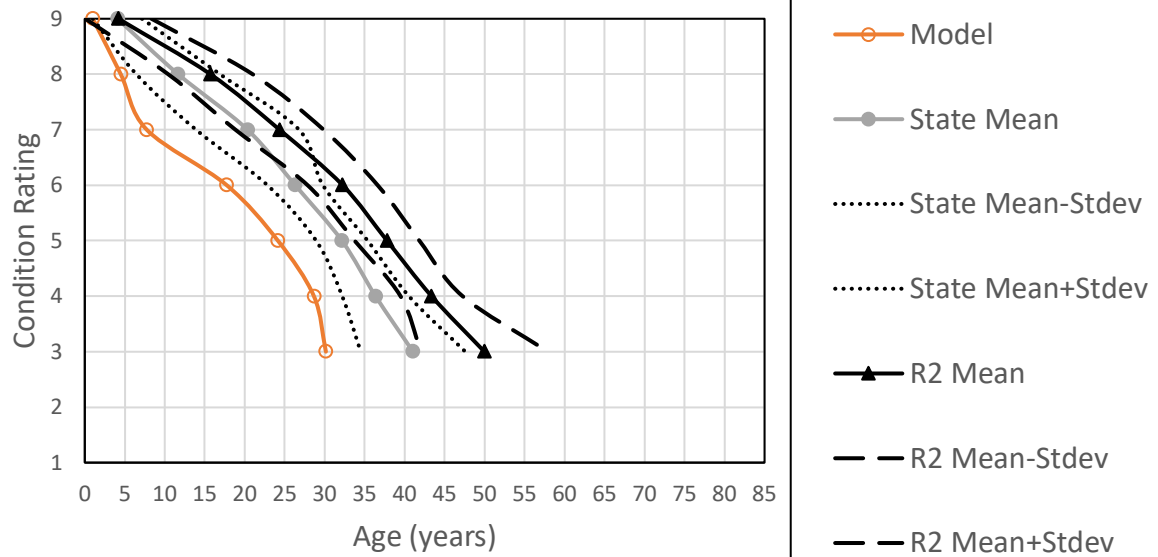
Figure 29. Chart. Deck beam deterioration curves: model vs state vs Region 2.
