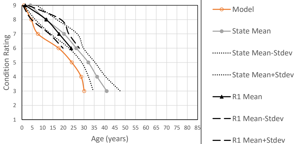
Figure 28. Chart. Deck beam deterioration curves: model vs state vs Region 1.
