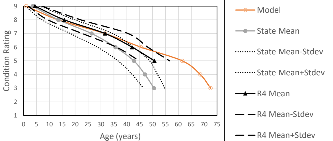
Figure 11. Chart. Superstructure deterioration curves: model vs state vs Region 4.
