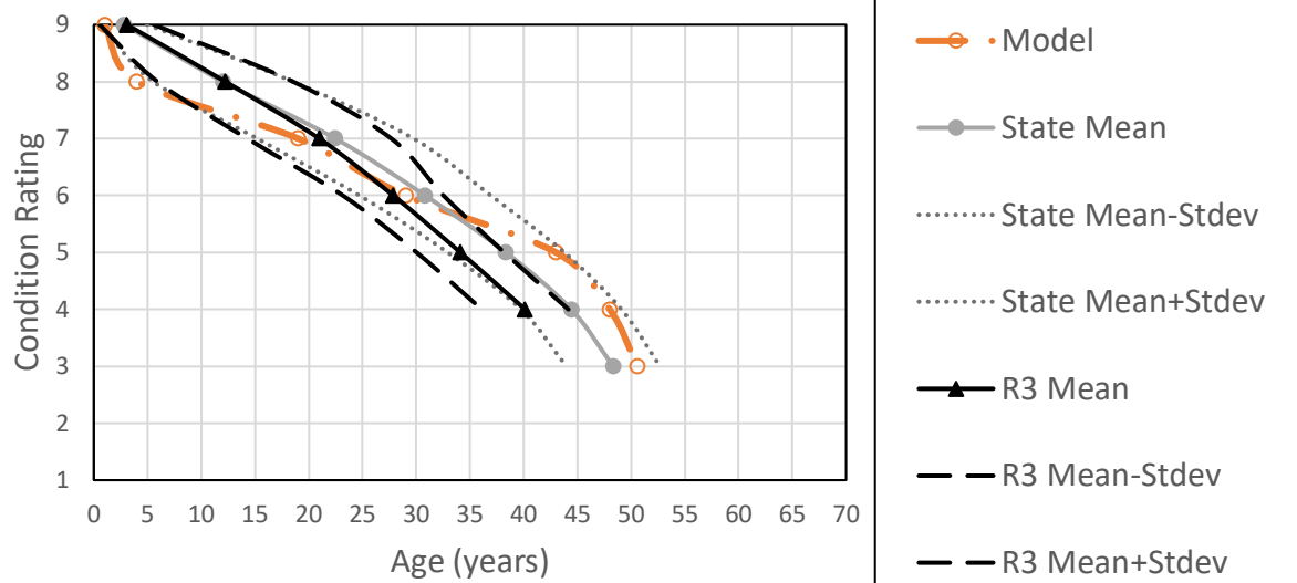
Figure 5. Chart. Deck deterioration curves: model vs state vs Region 3.
