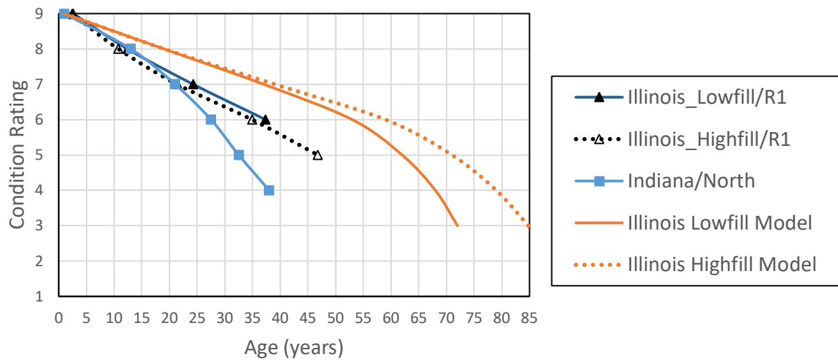
Figure 42. Chart. Illinois Region 1 vs Indiana North: Culvert.
