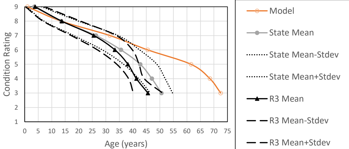
Figure 10. Chart. Superstructure deterioration curves: model vs state vs Region 3.
