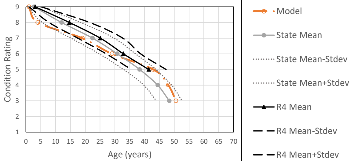
Figure 6. Chart. Deck deterioration curves: model vs state vs Region 4.
