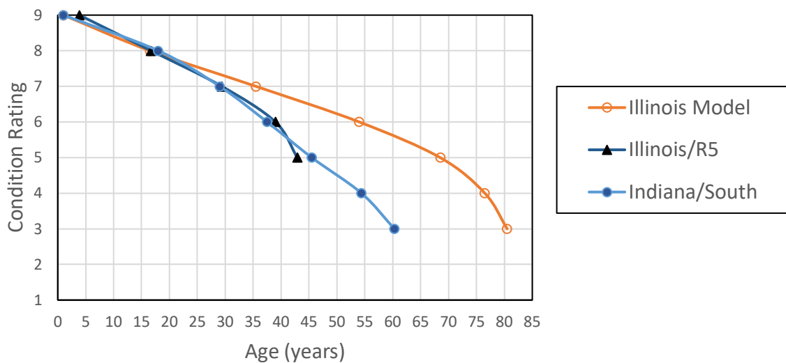
Figure 41. Chart. Illinois Region 5 vs Indiana South: Substructure.
