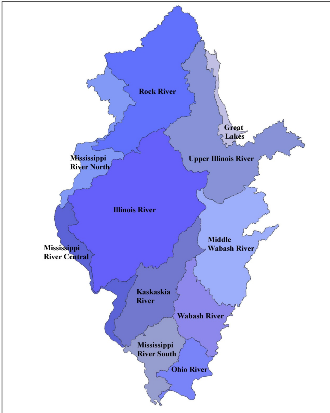
Figure 2.4. Ecological Drainage Units (EDUs) for Illinois were derived using drainages and HUC8s with relatively similar fish and mussel species assemblages.
