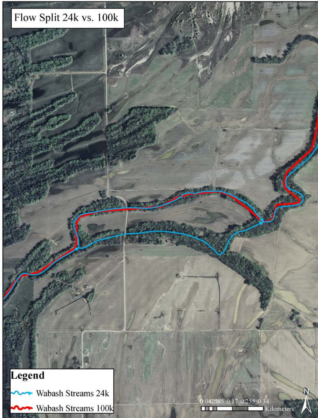
Figure AI.5. Flow Split. We defined flow splits as portions of the digital stream network where water from a single channel flows into two separate channels. The 2005 stream network (red lines) required water to flow along a single path necessitating the removal of some existing stream connections. With the switch to an ArcHydro framework we were able to include these existing connections in the 2014 digital stream network (blue lines).
