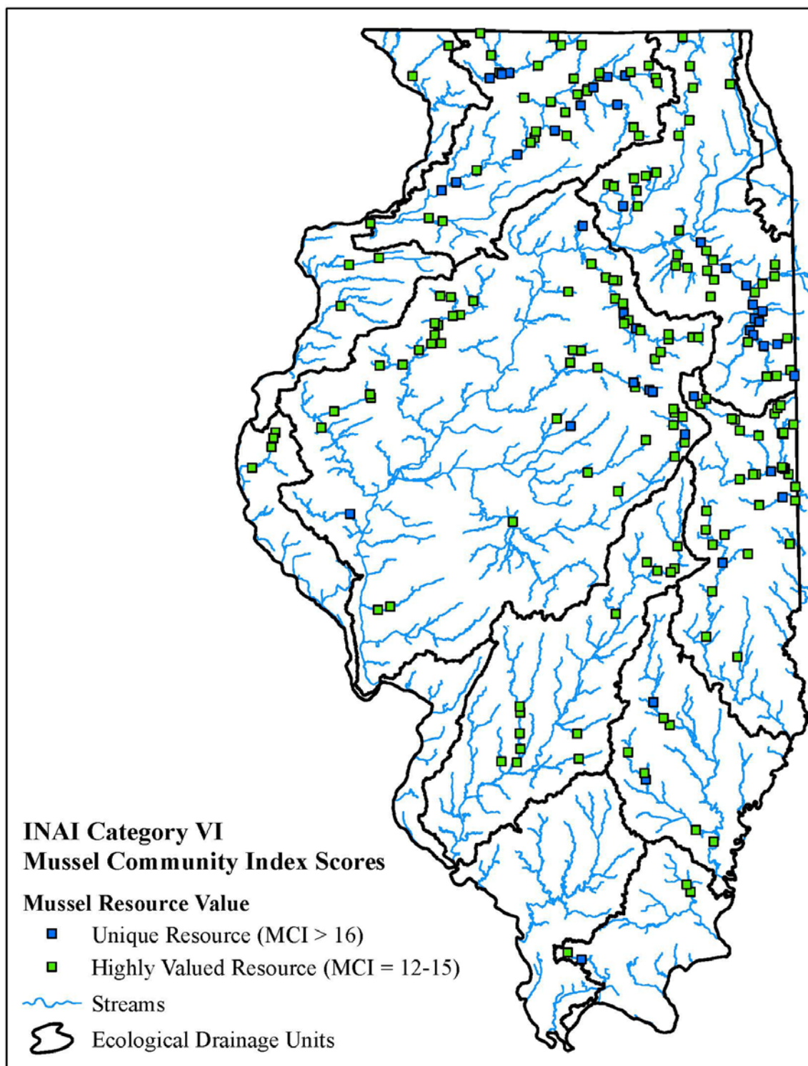
Figure 6.2. Reaches identified with Mussel Classification Index Scores that would qualify as the INAI Category VI criteria for “Unusual concentration of flora or fauna” under existing criteria. This analysis was based on all community samples collected during the period 2000-2014.
