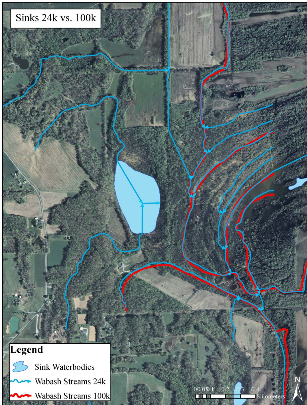
Figure AI.6. Sinks. We defined sinks as points, or polygons, with drainages that are disconnected from any portion of the stream network that eventually flows out of the EDU. These are essentially isolated drainages. The 2005 stream network filled all sinks so that water would contribute directly to the stream network (red lines). The 2014 digital stream network (blue lines) has isolated drainages, such as the sink waterbody shown here, that do not contribute to adjacent drainages.
