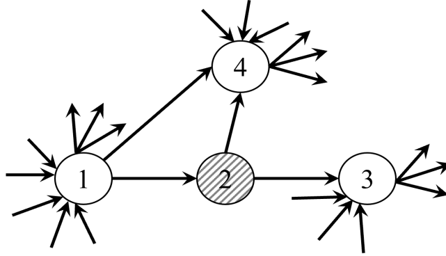
Figure 3.2: Illustration of different vertex connectivity.
