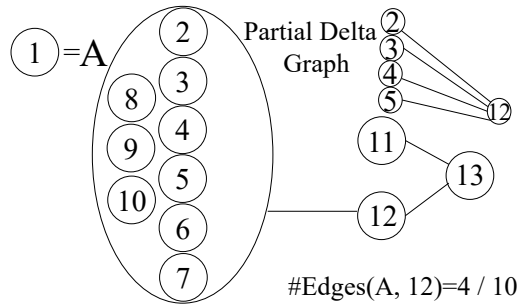
(c) G_t + 2 , delete \{2, 11\}, \{4, 11\}
