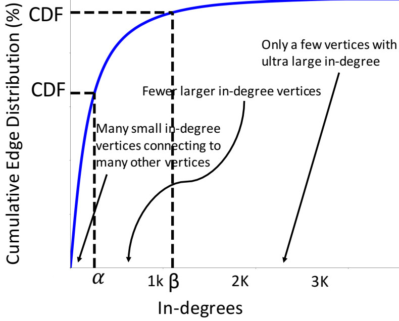
Figure 3.8: Finding \alpha and \beta based on the cumulative edge distribution.
