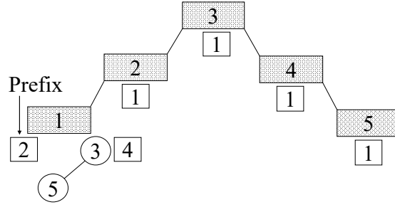
Figure 4.2: Aspen for Figure 4.1 for the first query.
