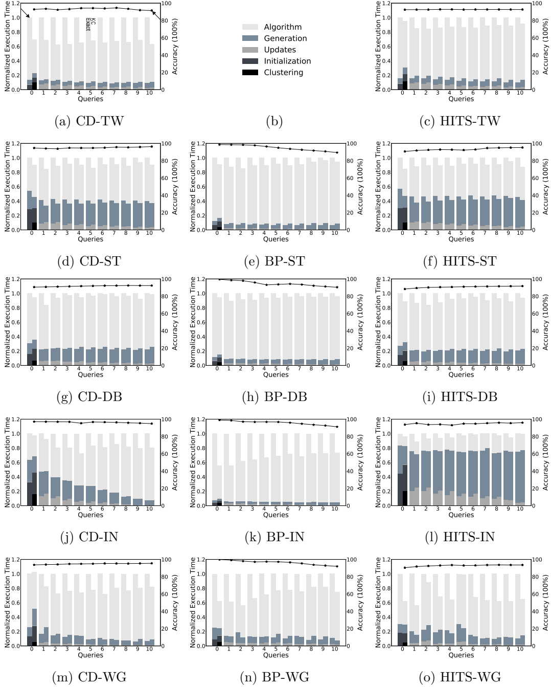
Figure 4.7: Comparing execution times (left Y-axis) and accuracy (right Y-axis) in exact (first bar) and KC (second bar) configurations.
