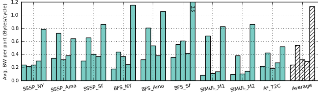
Figure 2.8: Average bandwidth consumption in each of the global crossbar ports connected to the core clusters. The bars in each application and input are ordered as in Figure 2.6.
