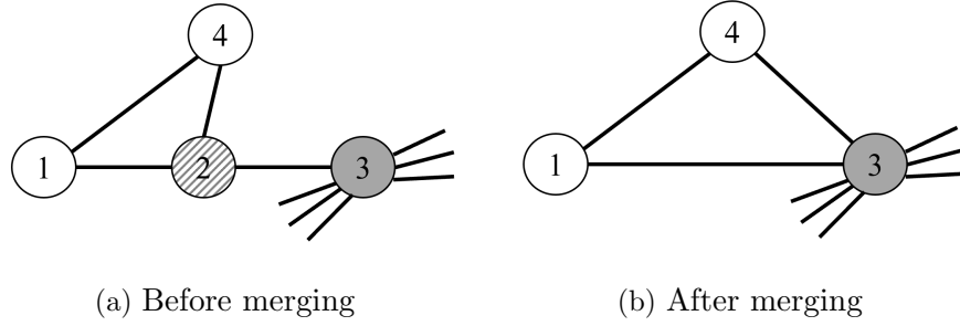
Figure 3.7: Merging subnode ② into supernode ③.
