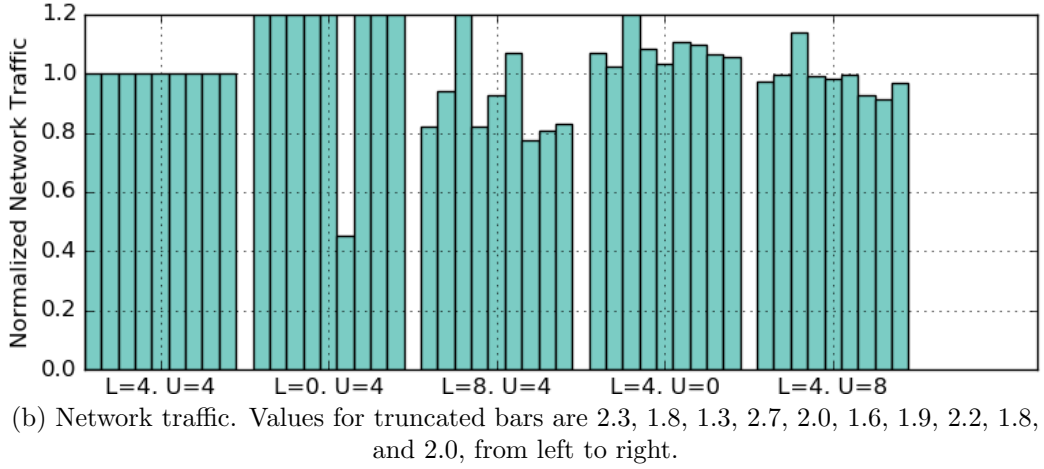
Figure 2.12: Sensitivity to the number of local accesses ( L ) and reuses of a snapshot ( U ).
