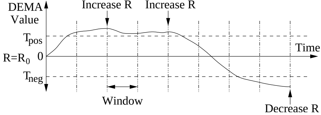
Figure 2.5: Example of how SNUG sets R .
