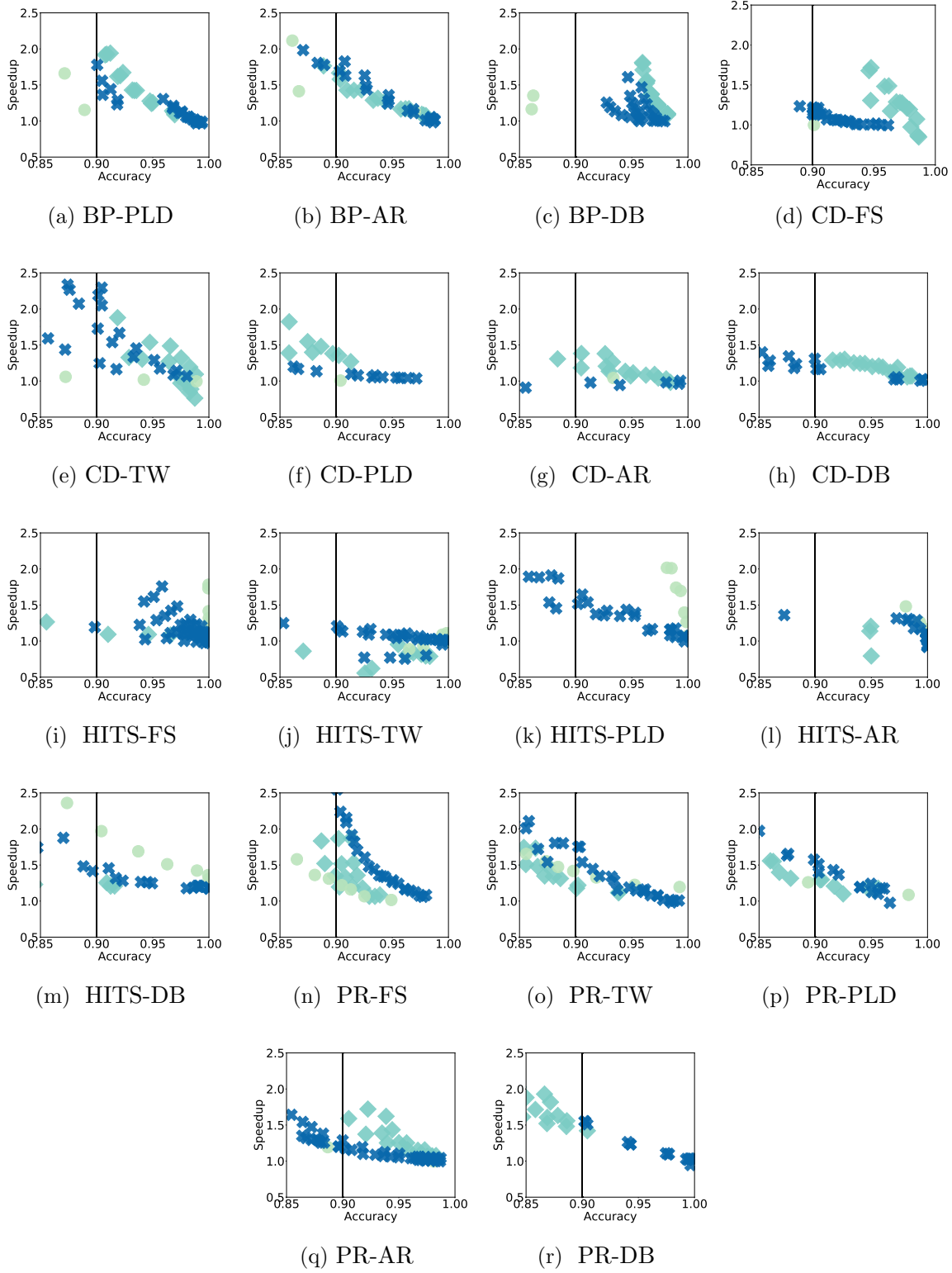
Figure 3.9: Pairs of (speedup, accuracy) for V-Combiner (✕), k-core (●), and sparsification (◆). Speedups only include algorithm execution time. The vertical line shows the 0.9 accuracy threshold.
