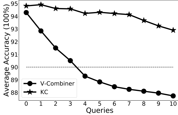
Figure 4.8: Comparing the accuracy of V-Combiner and KC for all queries.
