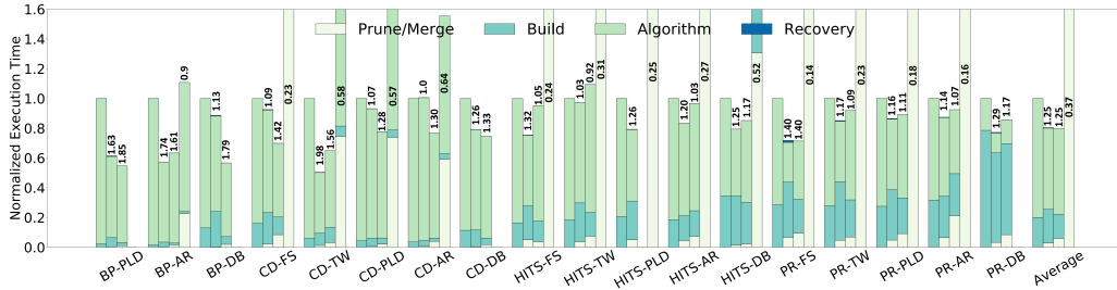
Figure 3.10: Total execution time of the best end-to-end configurations for the different benchmark-graph pairs and different techniques. For each benchmark-graph pair, we show, from left to right, bars for the exact, V-Combiner, sparsification, and k-core techniques, all normalized to exact. The numbers on top of the bars are the end-to-end speedups over exact. The missing bars (one in sparsification and four in k-core) are for configurations that failed to reach the threshold accuracy.
