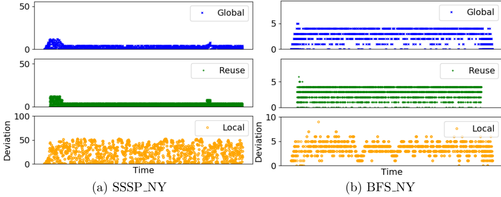
Figure 2.10: Difference between the priority returned by PickHead and the best priority in snapshot.
