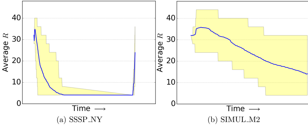
Figure 2.13: Average value of R as execution progresses.
