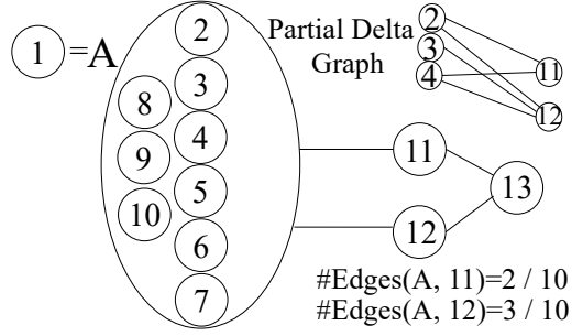
(a) G_t , initialize a compressed graph
