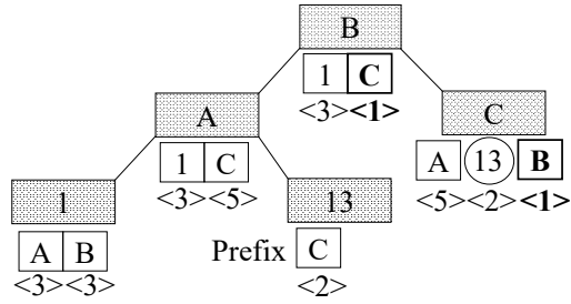
(b) Adding \{5, 12\} at t + 1
