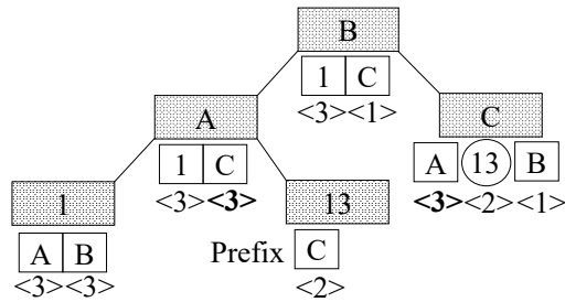
(c) Deleting \{2, 11\} , \{4, 11\} at t + 2
