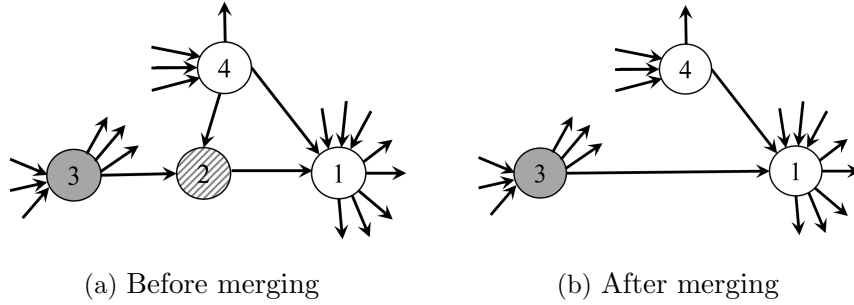
Figure 3.6: Merging out-subnode ② into out-supernode ③.
