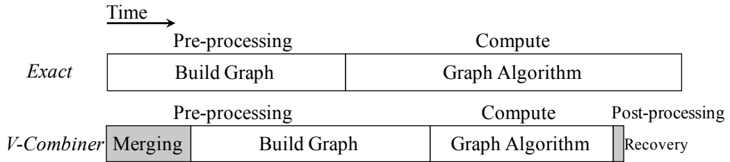
Figure 3.4: End-to-end execution steps of a graph algorithm.
