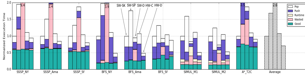
Figure 2.6: 64-core execution time of the evaluated applications and inputs on different priority queue implementations.
