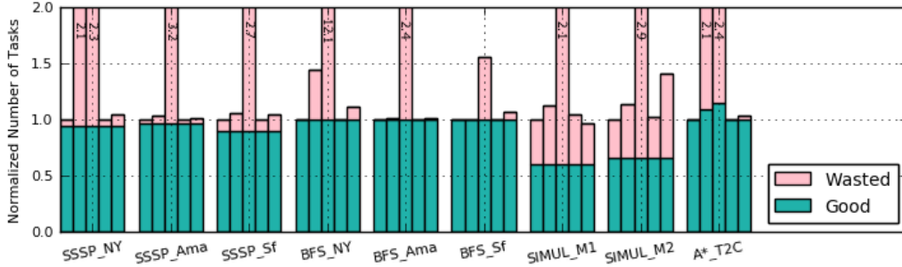
Figure 2.7: Breakdown of the tasks in the applications into good and wasted tasks. The bars in each application and input are ordered as in Figure 2.6.
