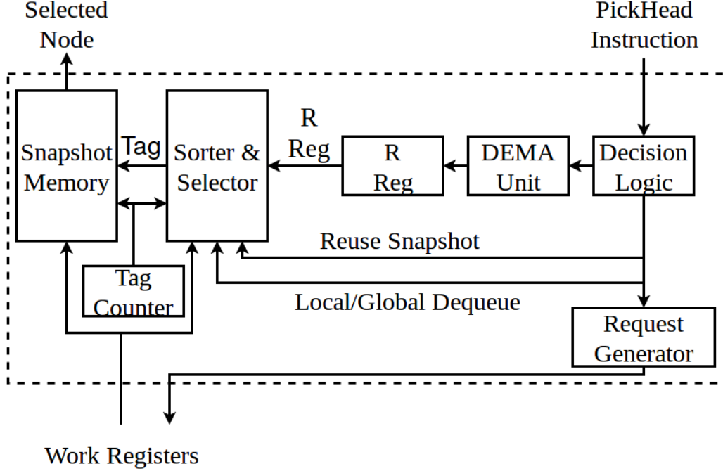
Figure 2.2: PickHead module.
