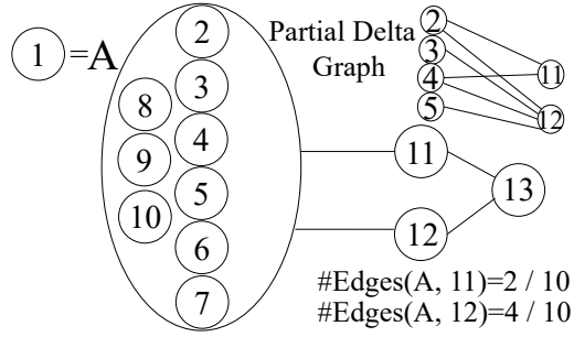
(b) G_t + 1 , add \{5, 12\}
