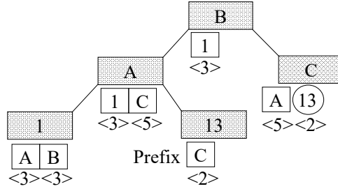
(a) Initializing reference graph at t . Vertices ordered as \textcircled{1} , \textcircled{A} , \textcircled{13} , \textcircled{B} , \textcircled{C} . \textcircled{13} is a key
