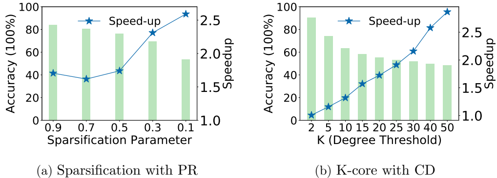
Figure 3.3: Illustration of sparsification and k-core.
