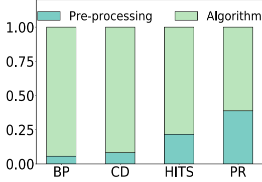
Figure 3.1: Impact of pre-processing time.
