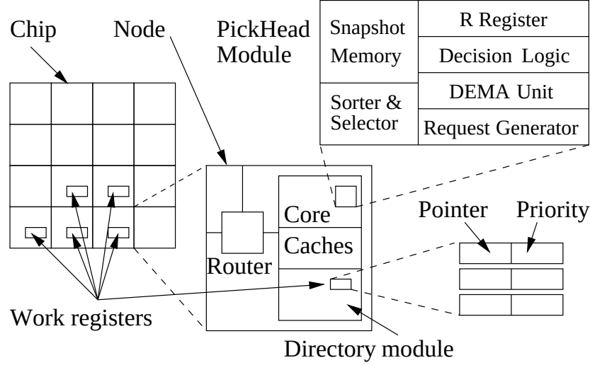
Figure 2.1: SNUG architecture in a directory-based manycore. Each directory module has a set of work registers, and each core has a PickHead module.
