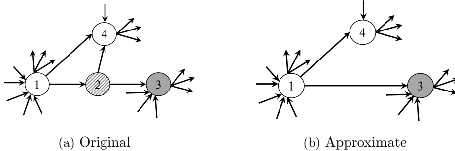
Figure 3.5: Vertex merging in V-Combiner.
