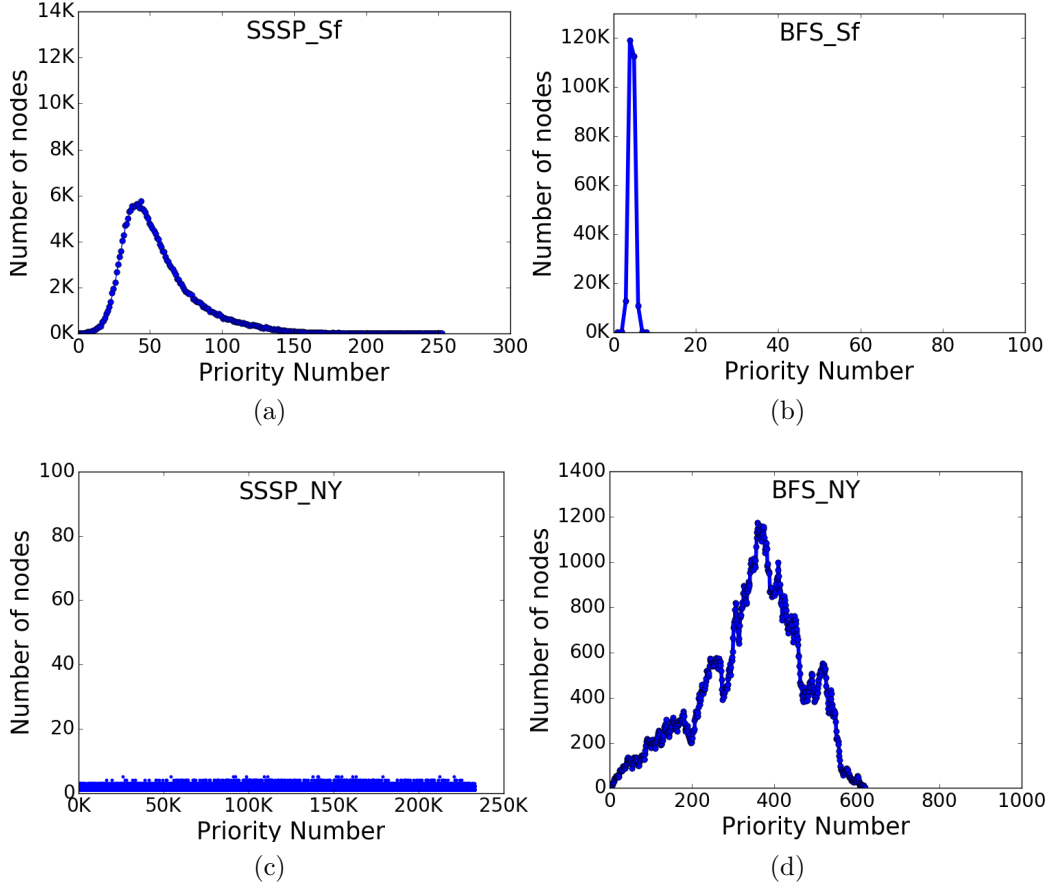
Figure 2.9: Priority distribution for applications and inputs.
