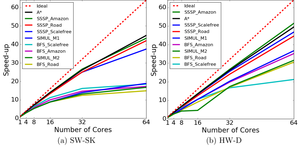
Figure 2.11: Speedup of SW-SK (a) and HW-D (b).
