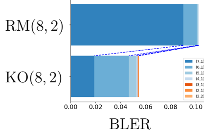
Figure 4.6: Separating each sub-code contribution in the \text{KO}(8, 2) decoder and the \text{RM}(8, 2) decoder reveals that \text{KO}(8, 2) improves in the total BLER by balancing the contributions more evenly over the sub-codes.
