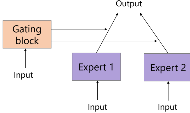
Figure 1.3: Mixture-of-Experts model.
