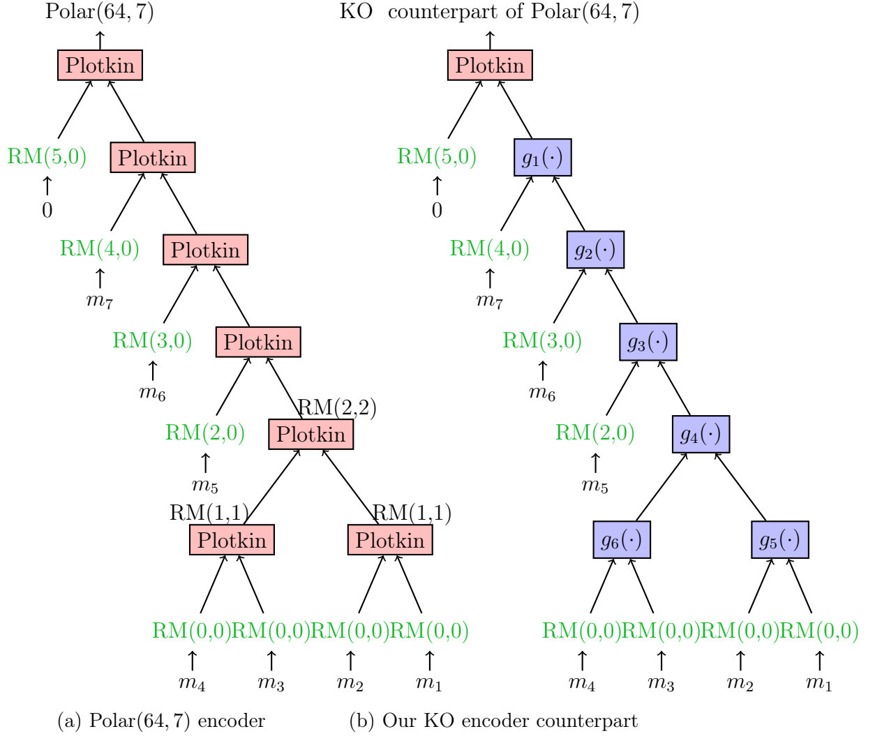
Figure C.1: Plotkin trees for the Polar(64, 7) encoder and our neural KO encoder counterpart. Both codes have dimension k = 7 and blocklength n = 64 .
