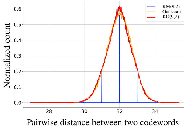
Figure 4.2: Histogram of pairwise distances between codewords of the KO(9, 2) code shows a strong resemblance to that of the Gaussian codebook, unlike the classical Reed-Muller code RM(9, 2) .
