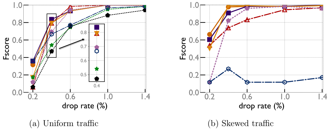
Figure 3.4: The extent of drop rates that each scheme can detect (each point averaged over 32 traces).
