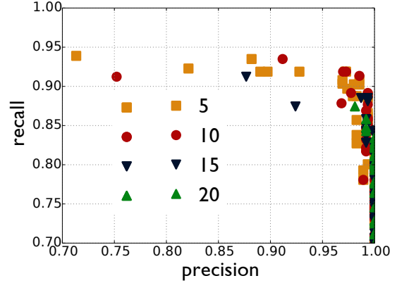
(b) Effect of changing priors
