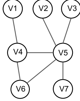
(b) A Markov Random Field (undirected PGM)
