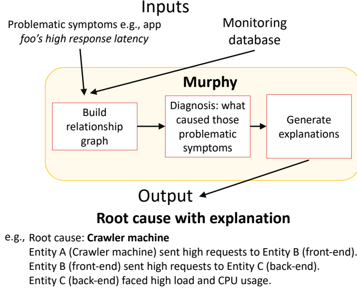
Figure 2.2: Murphy workflow
