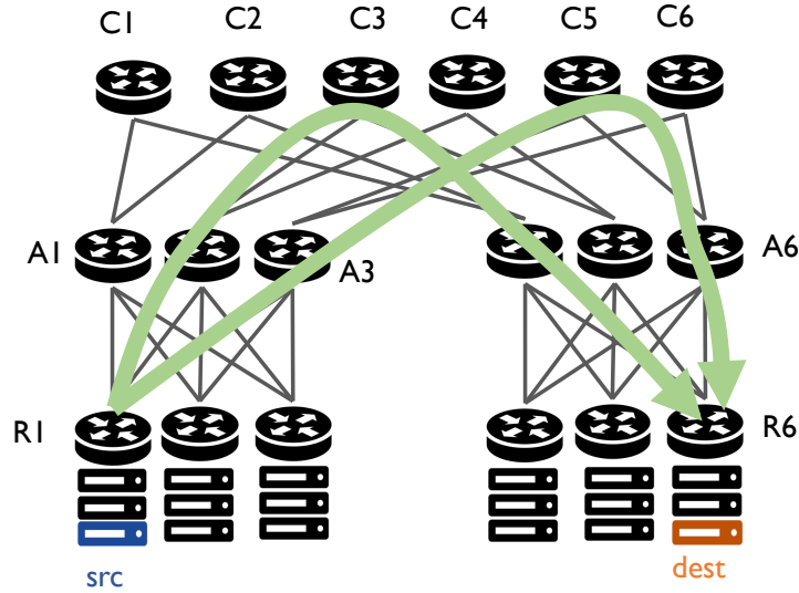
Figure 4.1: Symmetric links in a Clos topology make it very hard to localize faults completely. Consider a failure scenario where several flows from src → dest are getting dropped due to a network “black hole” at one of the core switches (C1 – C6). It’s impossible to distinguish between C1-C6 without knowing the exact ECMP path taken by the flows. Two such ECMP paths are shown: any flow that can possibly take one path can also take the other.
