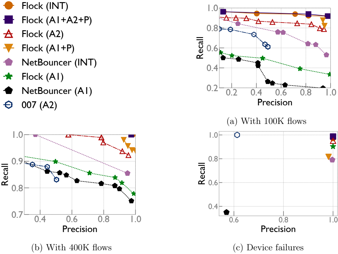
Figure 3.3: Accuracy for silent packet drops. (a), (b): Tradeoff curves for NetBouncer, 007 and Flock for silent drops, varying hyperparameters for each scheme. Schemes are annotated with the input data they use. (c): Accuracy on device failures.
