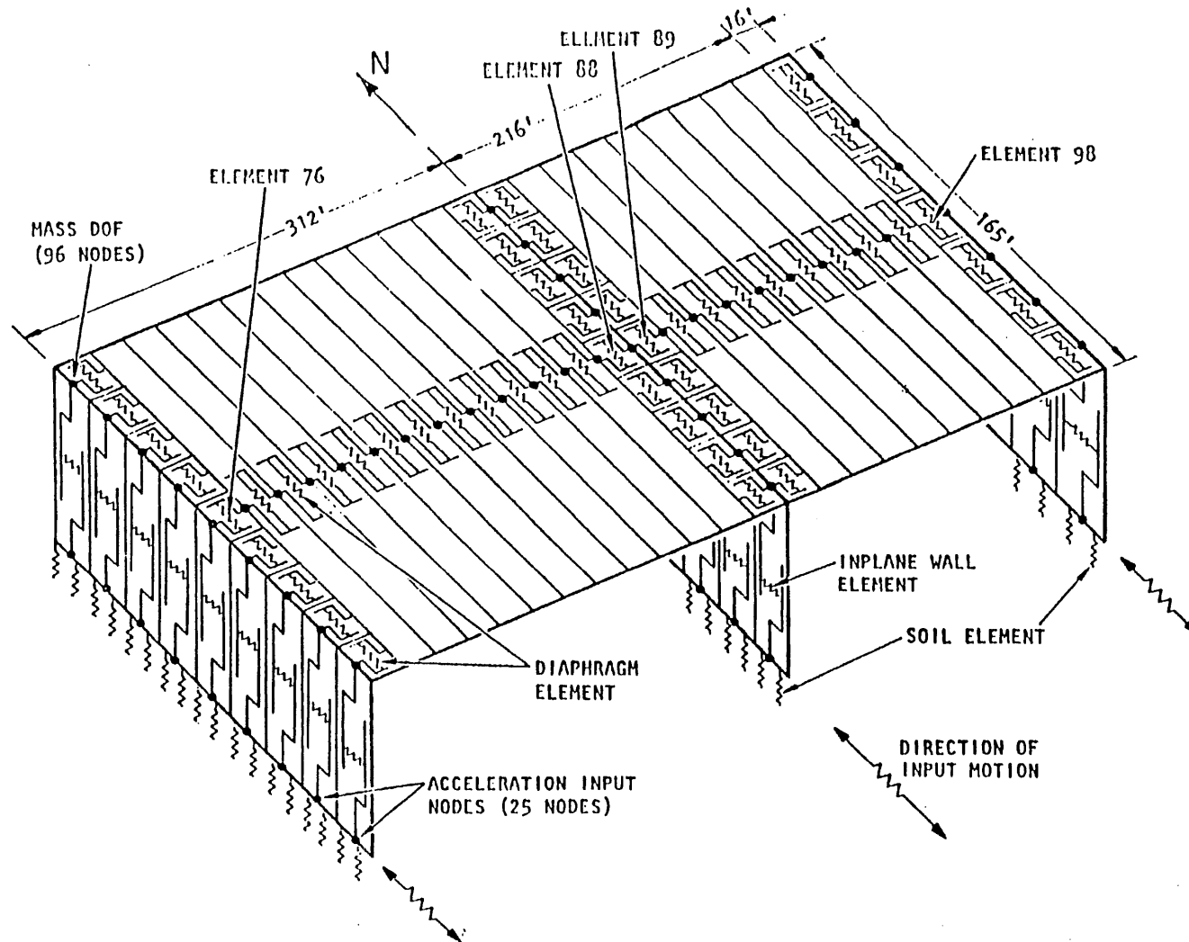
Fig. 4.27 Analytical model of Downey building for input motion in the transverse direction [9].
