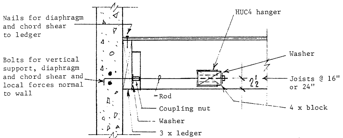
PLAN VIEW
