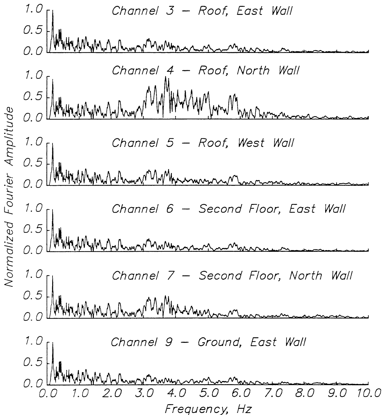
Fig. 5.41 Milpitas industrial building – 1989 Loma Prieta earthquake. (a) Normalized Fourier amplitude spectra of transverse acceleration response.
