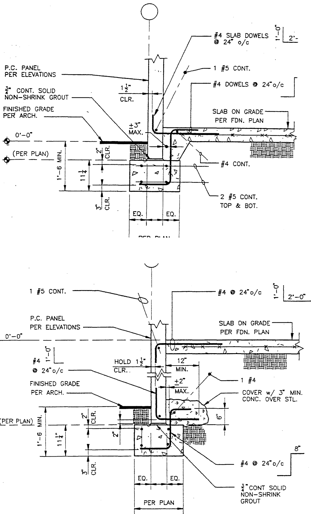
Fig. 3.17 Typical panel-to-foundation connections in buildings constructed after 1971 [40].
