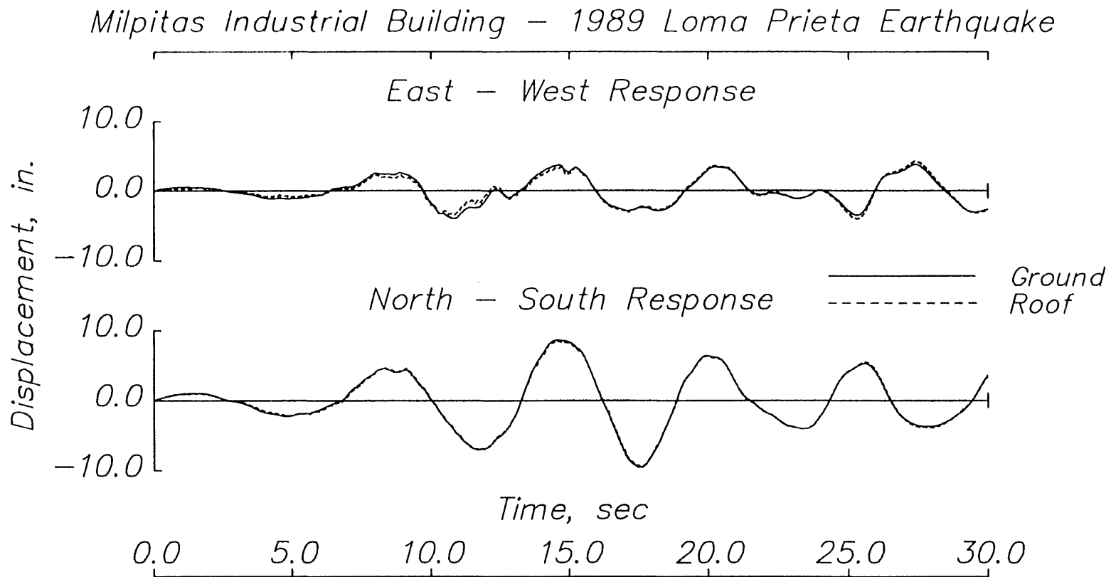
Fig. 5.42 (cont.) Milpitas industrial building – Absolute displacement response.
