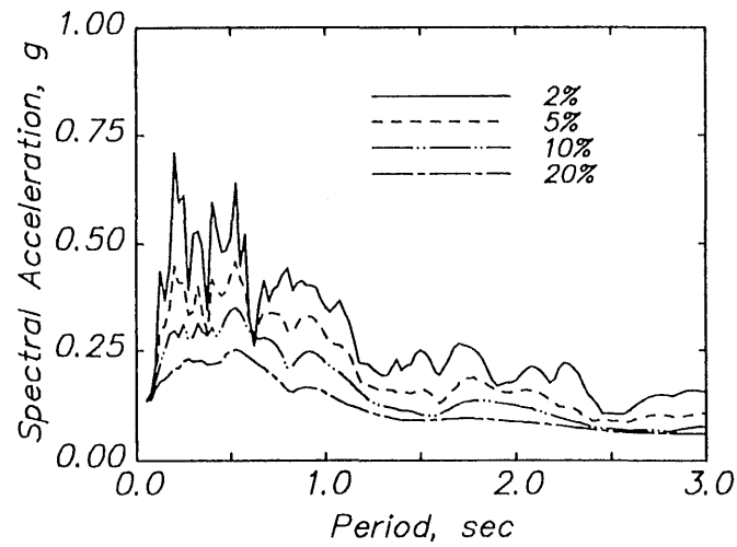
Fig. 5.37 (cont.) Linear response spectra – Milpitas industrial building.
