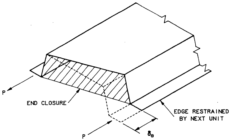
(a) UNIT RESTRAINED AGAINST END WARPING
