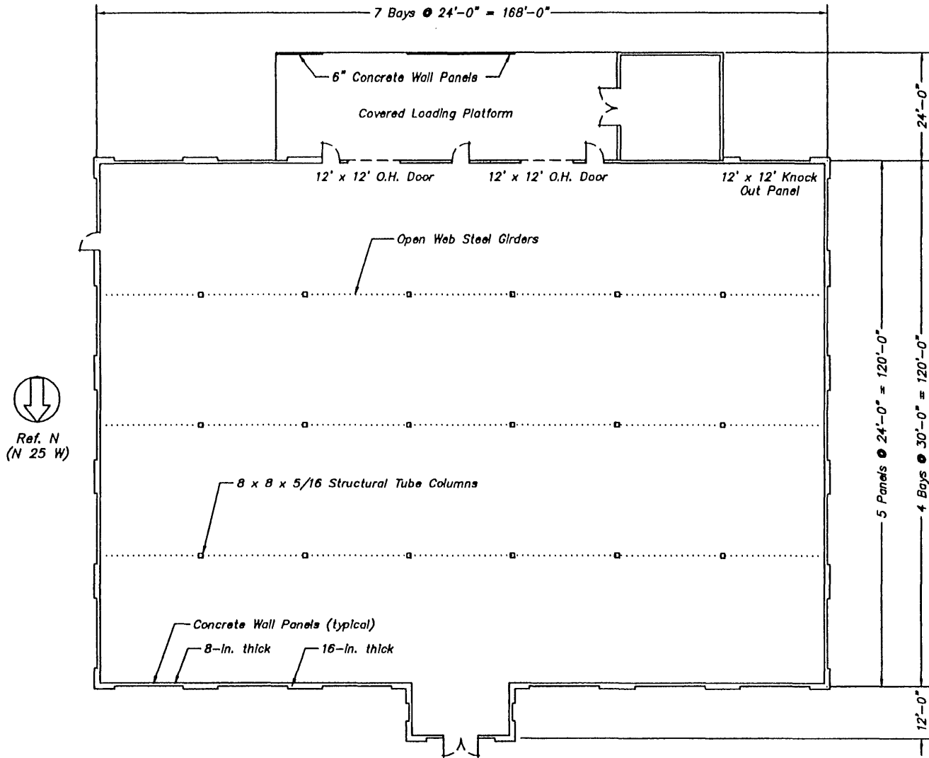
First-Story Plan - Milpitas Industrial Building
