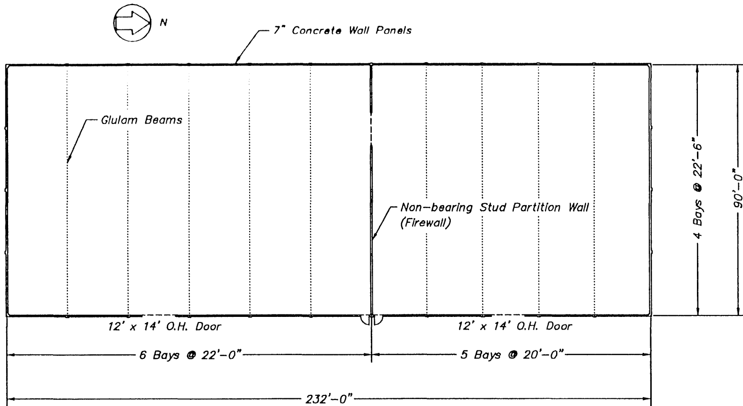
Fig. 5.20 Floor plan – Redlands warehouse.
