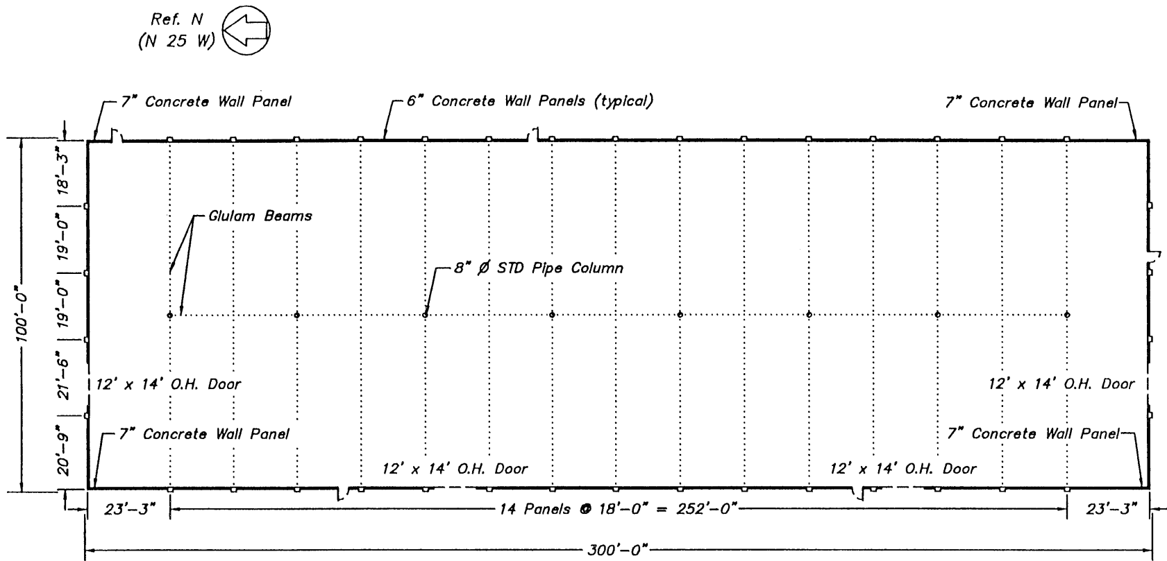
Fig. 5.2 Floor plan – Hollister warehouse.
