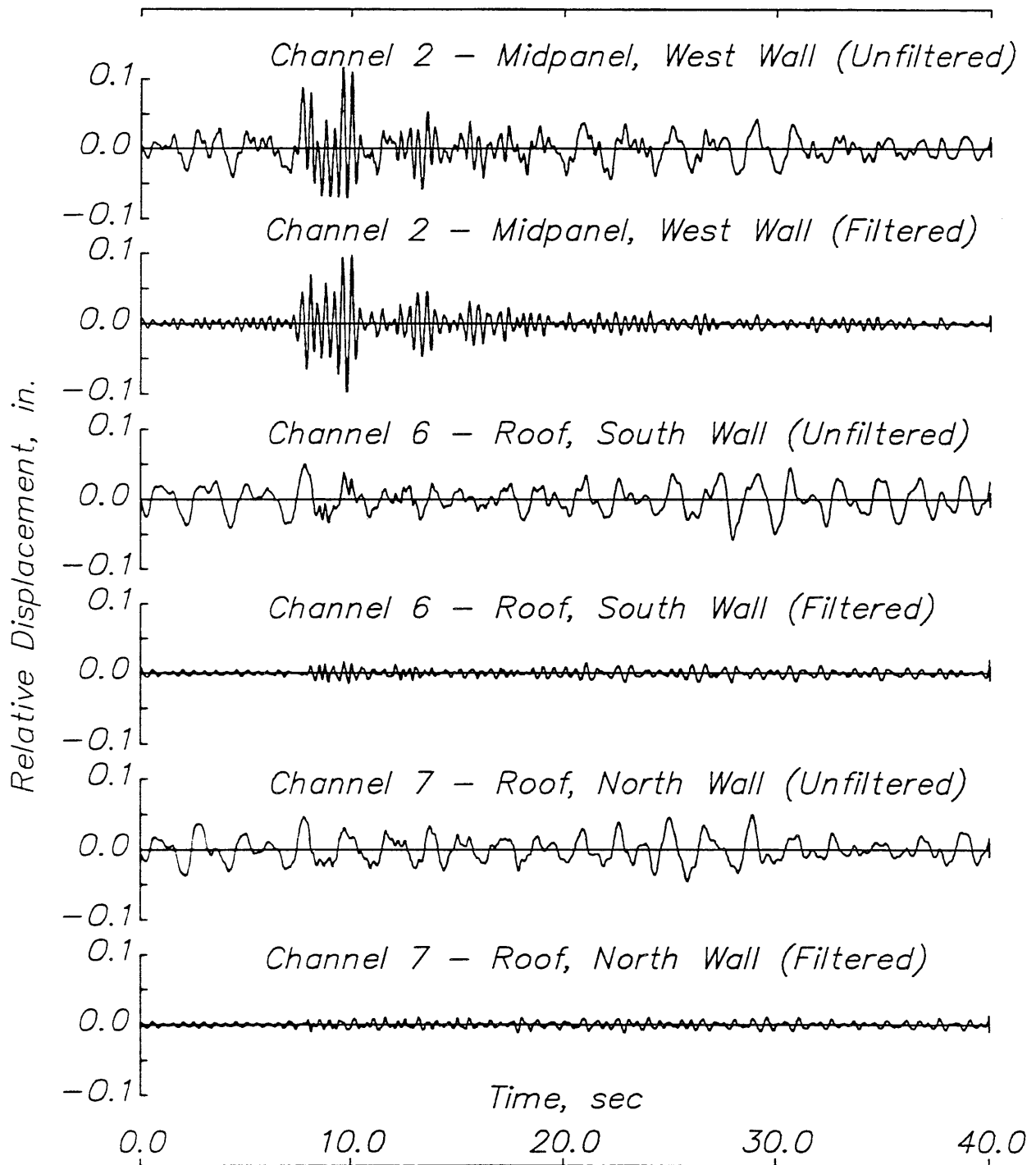
Fig. 5.31 (cont.) Redlands warehouse – 1986 Palm Springs earthquake. (a) (cont.) Transverse relative displacement response.
