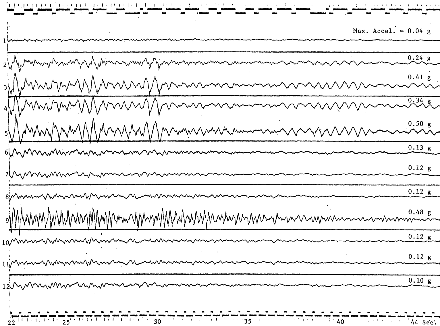
Fig. 5.27 (cont.) Redlands warehouse - 1992 Landers earthquake [66].
