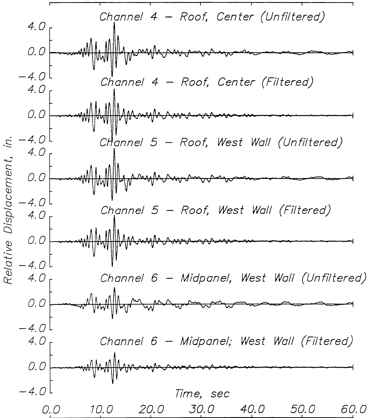
Fig. 5.18 Hollister warehouse – 1989 Loma Prieta earthquake.
