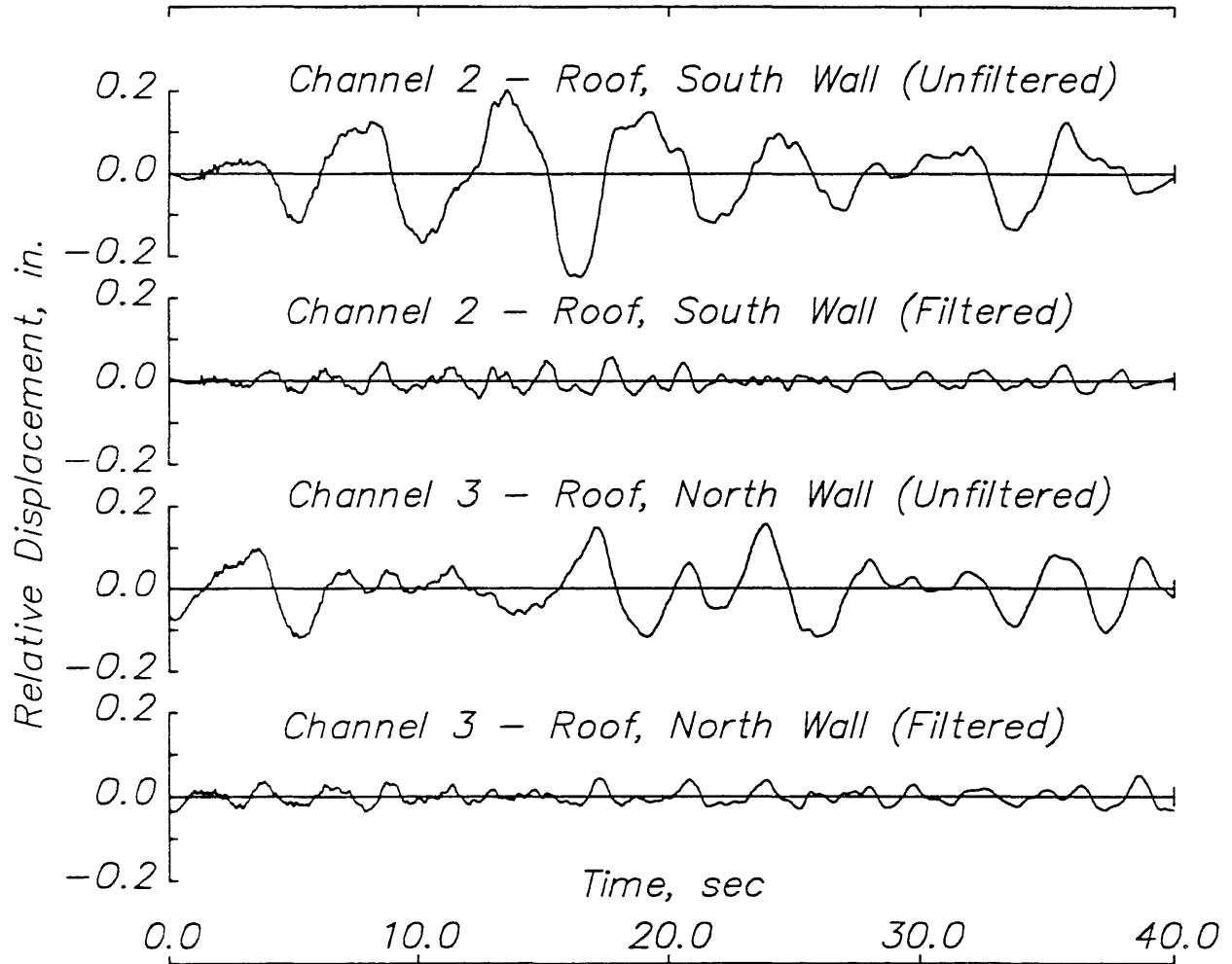
Fig. 5.16 (cont.) Hollister warehouse – 1984 Morgan Hill earthquake. (b) Transverse relative displacement response.
