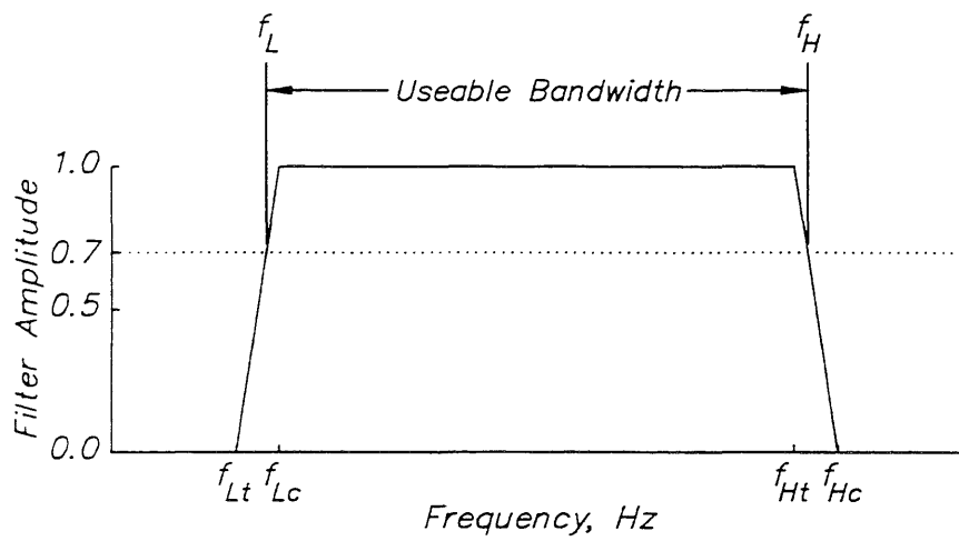
Fig. B.2 Ormsby filter used to process CSMIP records [38].
