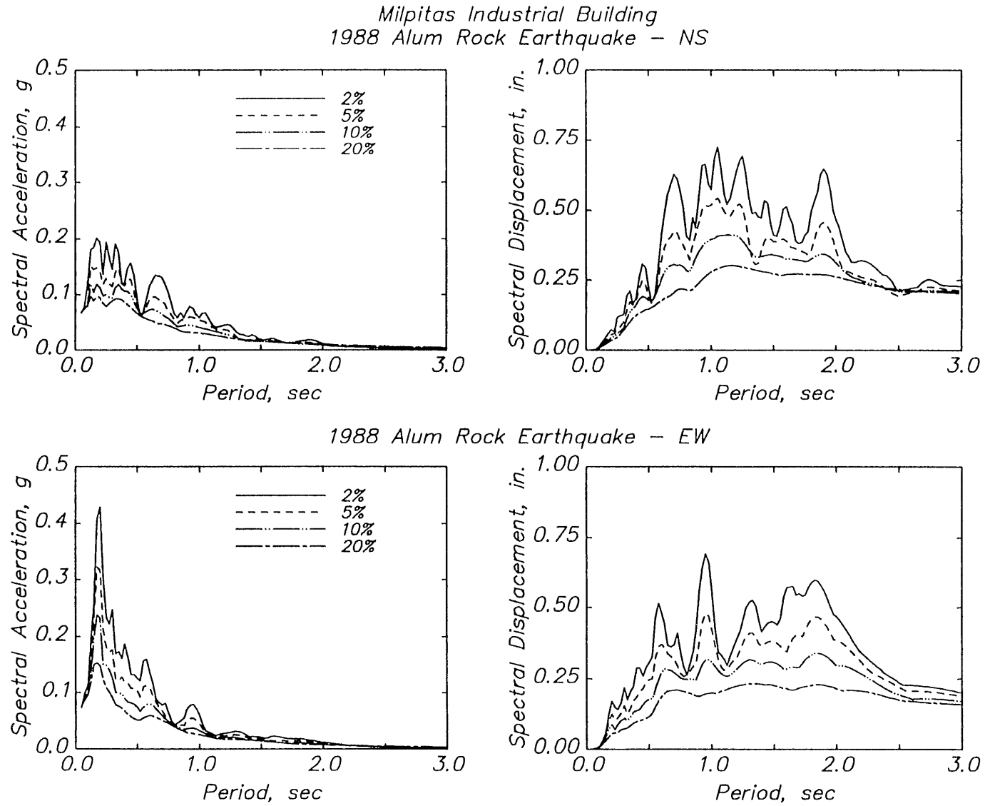
Fig. 5.37 Linear response spectra – Milpitas industrial building.
