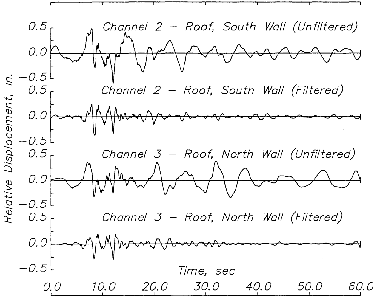
Fig. 5.18 (cont.) Hollister warehouse – 1989 Loma Prieta earthquake.
