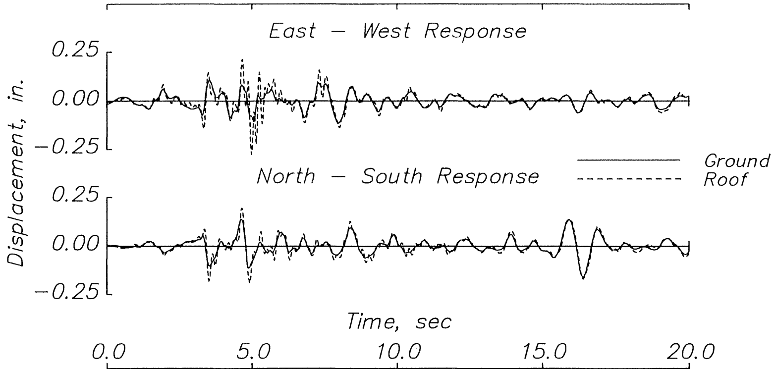
Fig. 5.42 Milpitas industrial building – Absolute displacement response.
