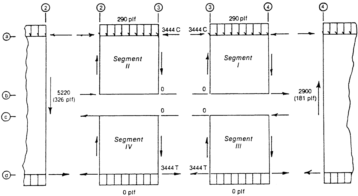
(b) Free-body diagram
