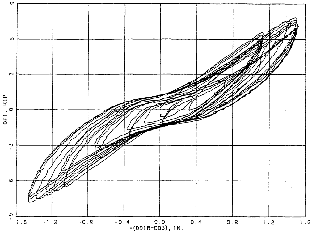
(c) Quasi-static load reversals [1].
