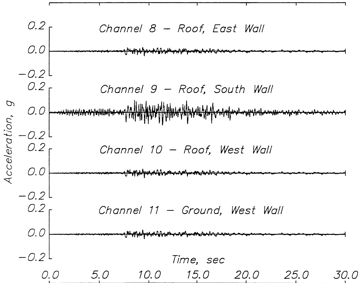
Fig. 5.26 Redlands warehouse – 1986 Palm Springs earthquake. (b) Longitudinal acceleration response.
