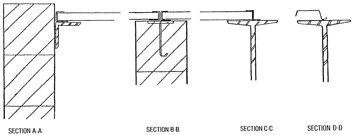
Fig. 2.10 Plan view of a steel diaphragm [64].
