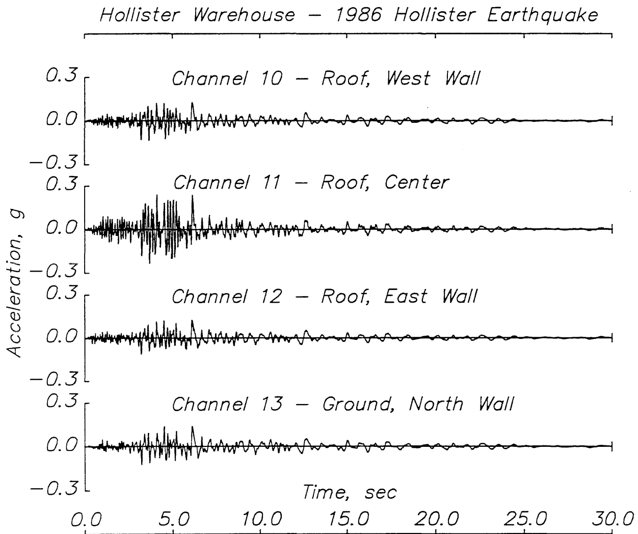
Fig. 5.10 (cont.) Hollister warehouse – 1986 Hollister earthquake. (b) Longitudinal acceleration response.
