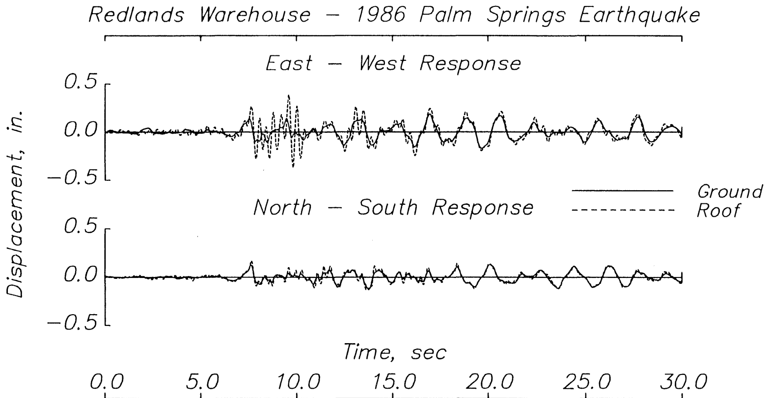
Fig. 5.30 Redlands warehouse – Absolute displacement response.
