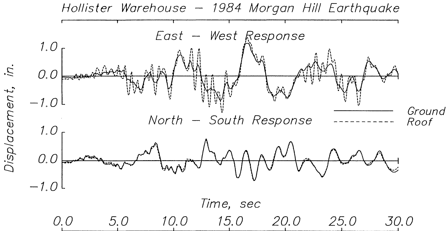
Fig. 5.15 Hollister warehouse – Absolute displacement response.
