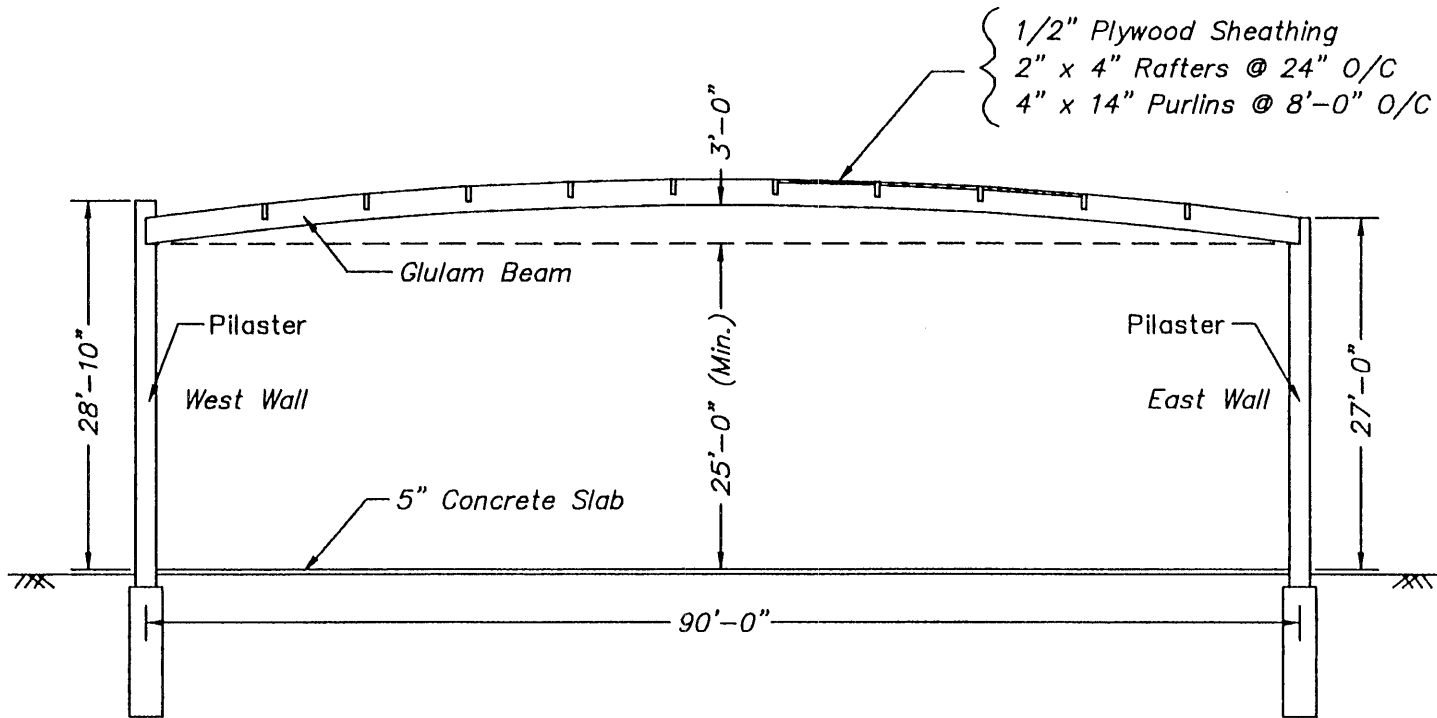
Fig. 5.21 Transverse cross section - Redlands warehouse.
