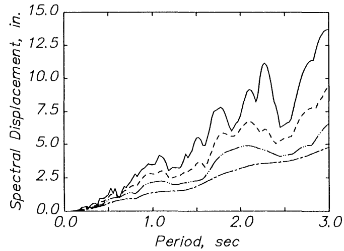
Fig. 5.37 (cont.) Linear response spectra – Milpitas industrial building.
