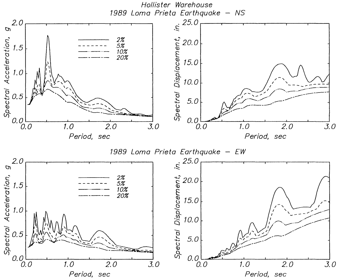
Fig. 5.8 (cont.) Linear response spectra – Hollister warehouse.
