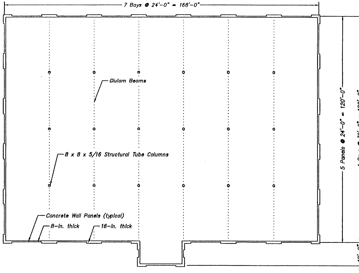
Second-Story Plan - Milpitas Industrial Building
