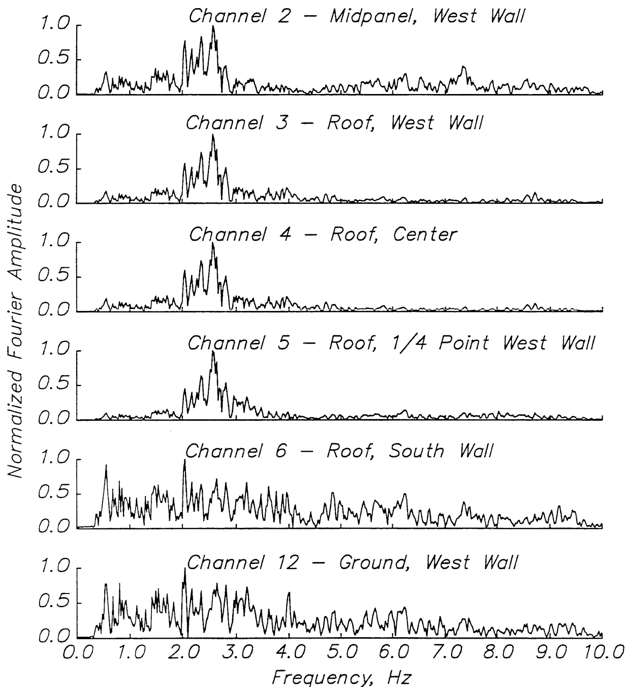
Fig. 5.29 Redlands warehouse – 1986 Palm Springs earthquake. (a) Normalized Fourier amplitude spectra of transverse acceleration response.
