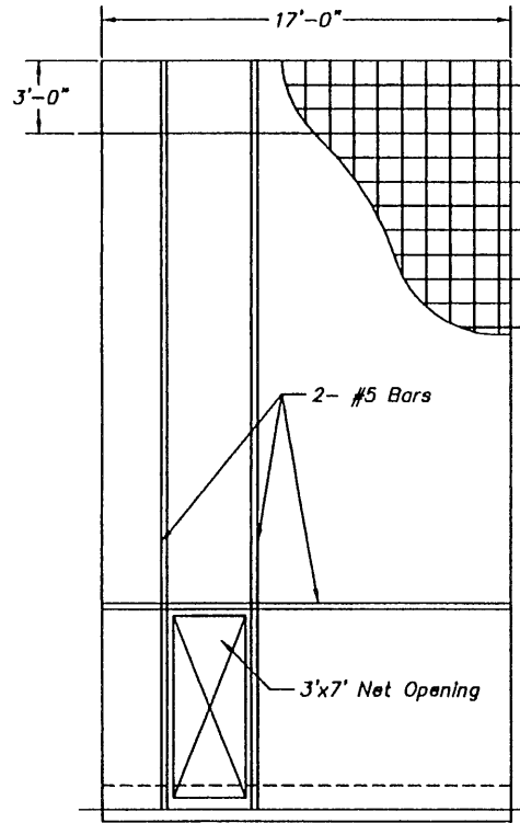
Fig. 5.4 Typical panel reinforcement details – Hollister warehouse.
