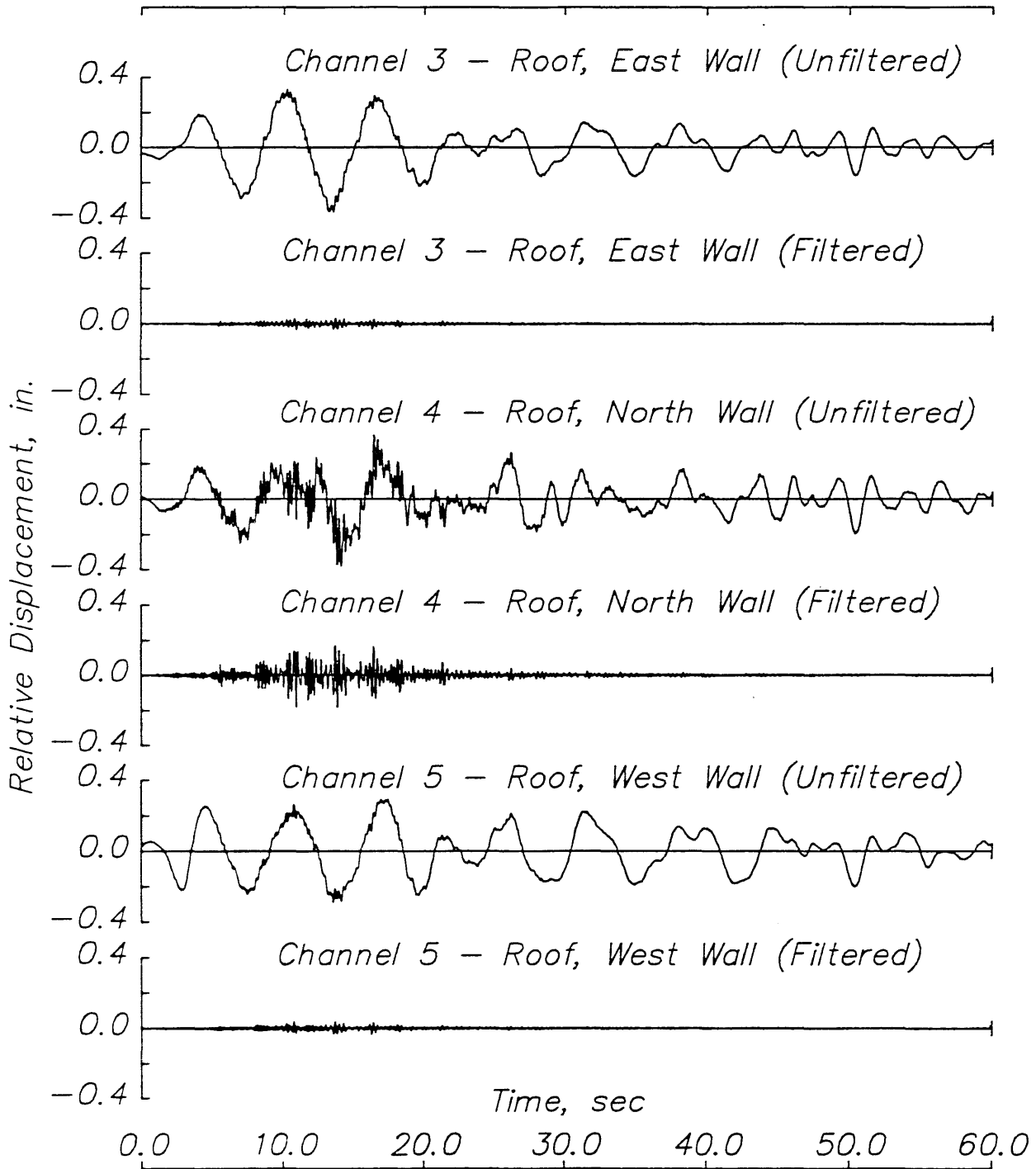
Fig. 5.44 Milpitas industrial building – 1989 Loma Prieta earthquake. (a) Transverse relative displacement response.
