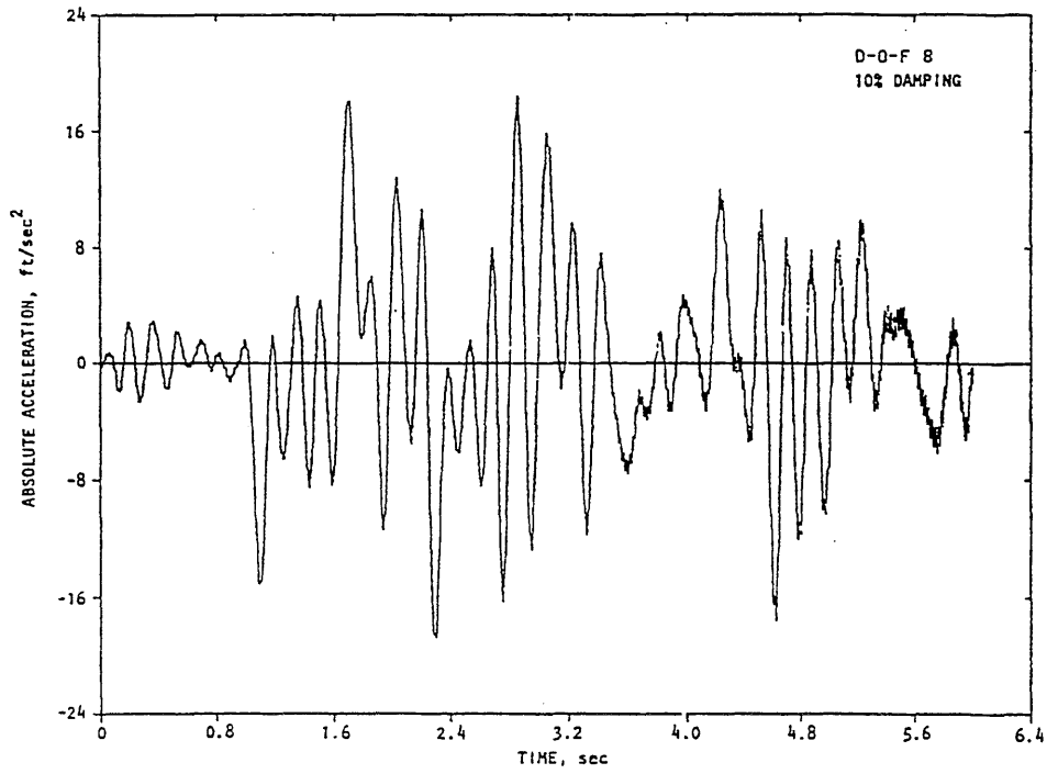
(a) Acceleration at mid-height of panel.
