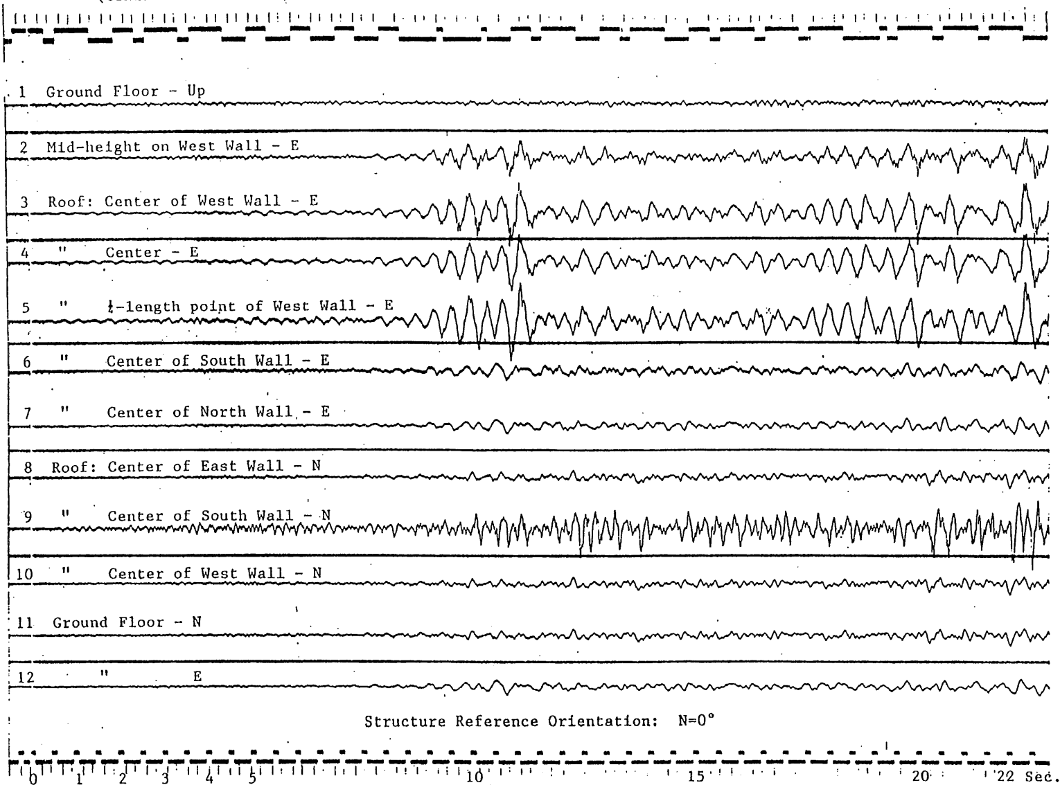
Fig. 5.27 Redlands warehouse - 1992 Landers earthquake [66].
