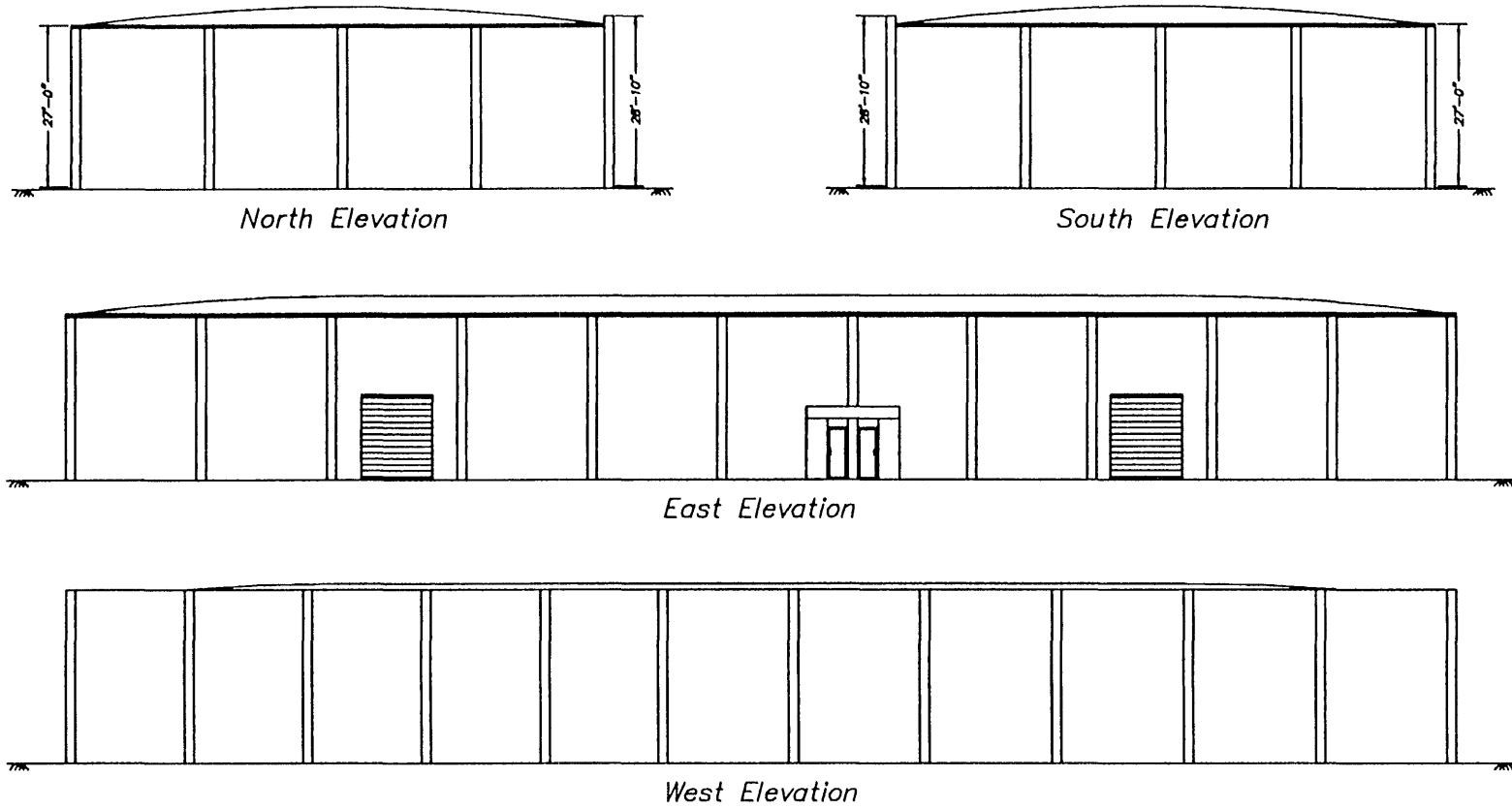
Fig. 5.22 Elevations – Redlands warehouse.
