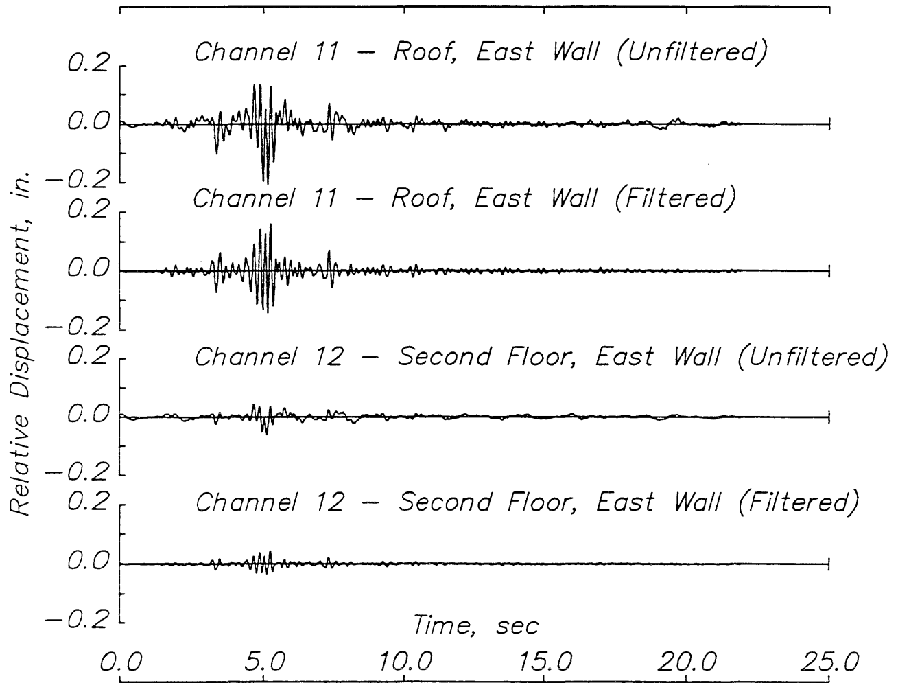
Fig 5.43 (cont.) Milpitas industrial building – 1988 Alum Rock earthquake. (b) Longitudinal relative displacement response.
