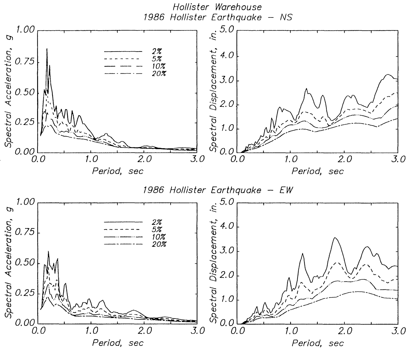
Fig. 5.8 (cont.) Linear response spectra – Hollister warehouse.
