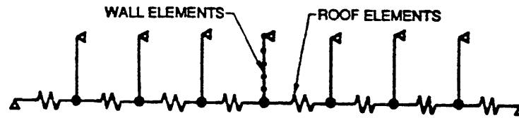
(c) Model used for nonlinear analyses.
