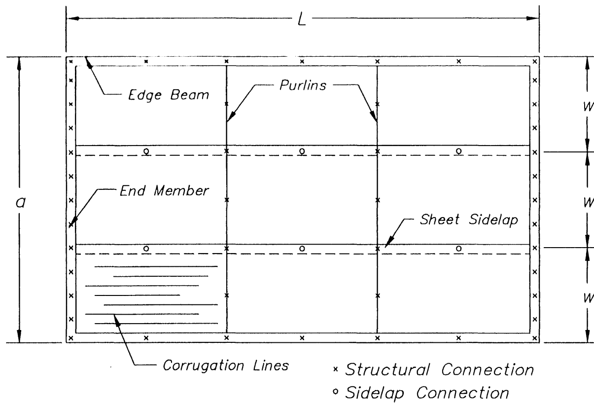
Fig. 3.6 Configuration of metal-deck diaphragm.
