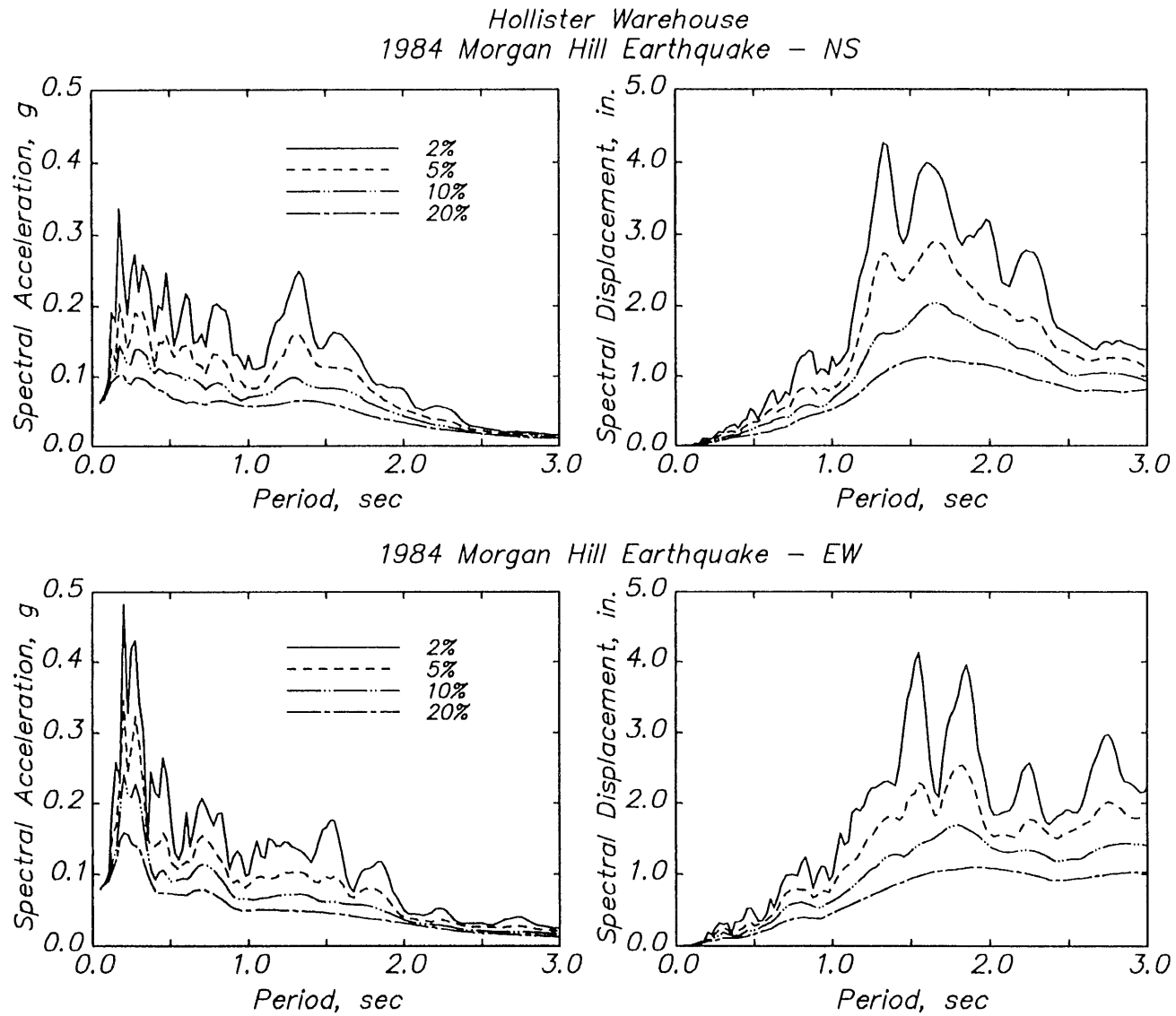
Fig. 5.8 Linear response spectra – Hollister warehouse.
