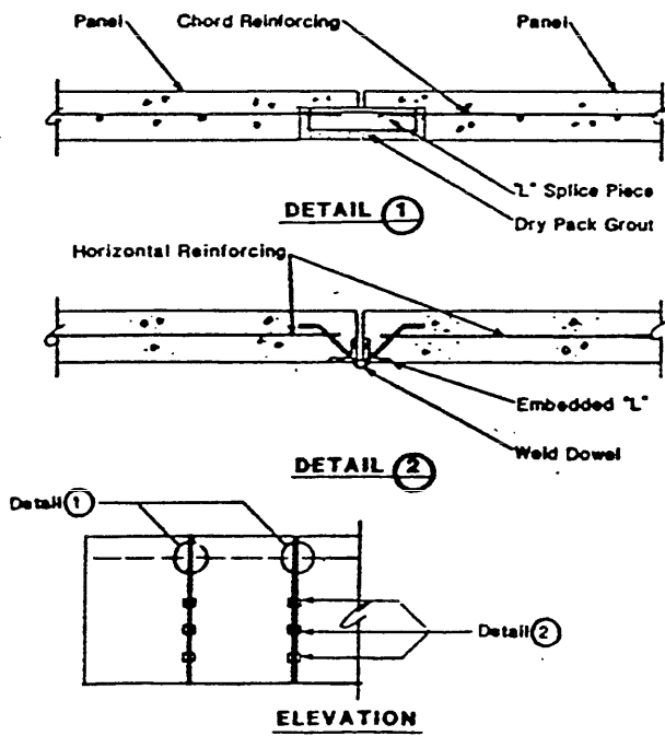
Fig. 3.18 Typical panel-to-panel connections in buildings constructed before 1971 [55,80]
