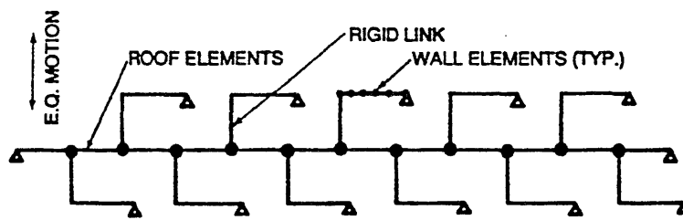
(b) Model used for linear analyses.
