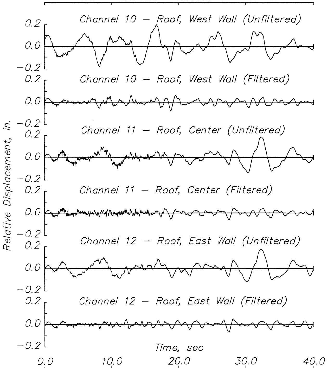
Fig. 5.16 (cont.) Hollister warehouse – 1984 Morgan Hill earthquake. (b) Transverse relative displacement response.
