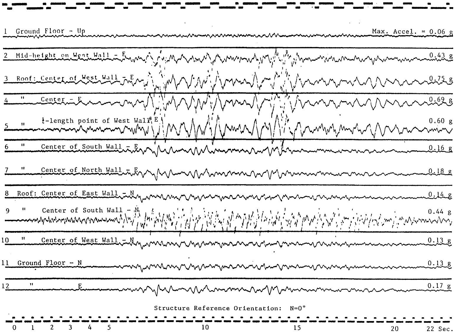
Fig. 5.28 Redlands warehouse - 1992 Big Bear earthquake [37].
