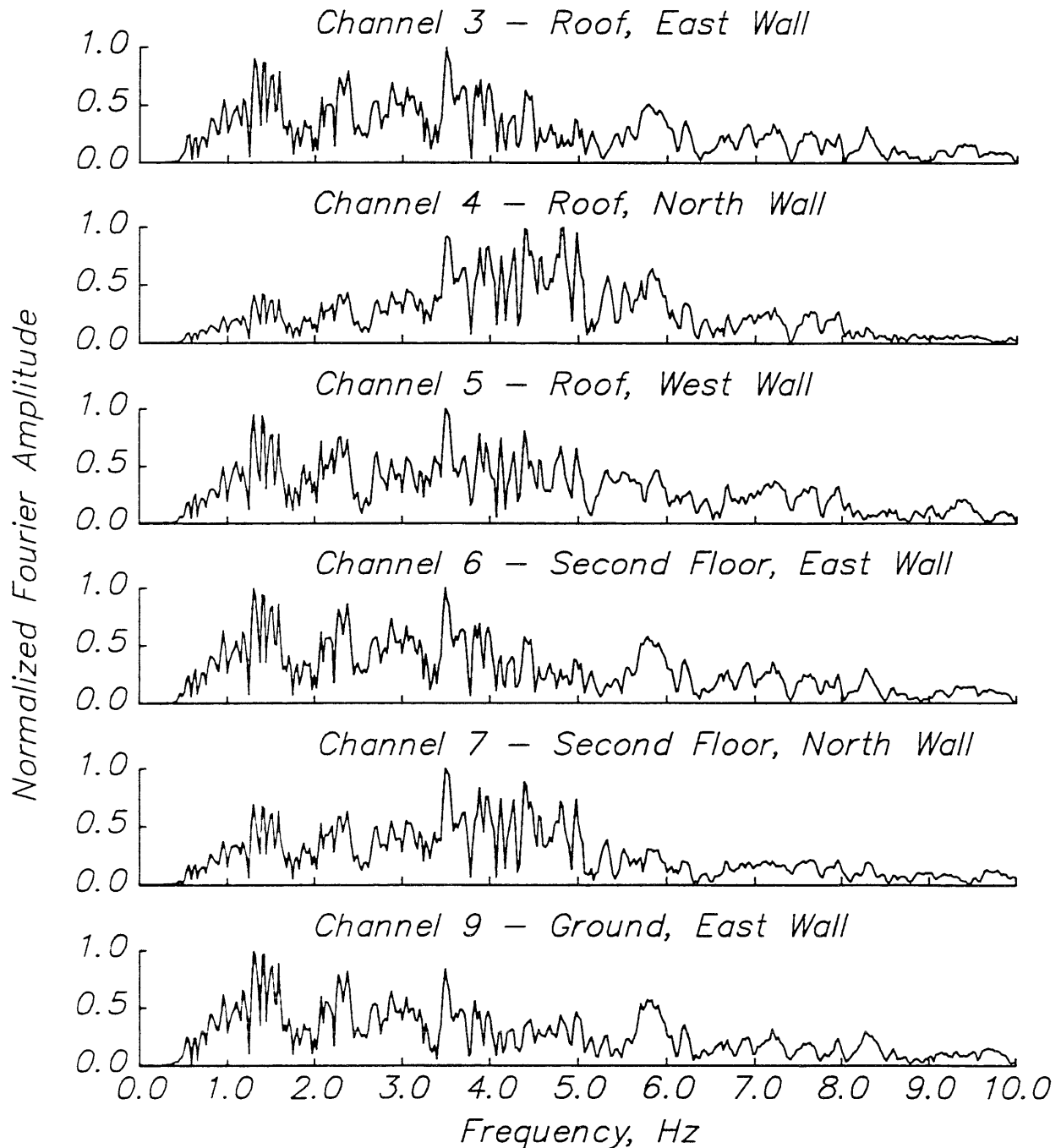
Fig. 5.40 Milpitas industrial building – 1988 Alum Rock earthquake. (a) Normalized Fourier amplitude spectra of transverse acceleration response.
