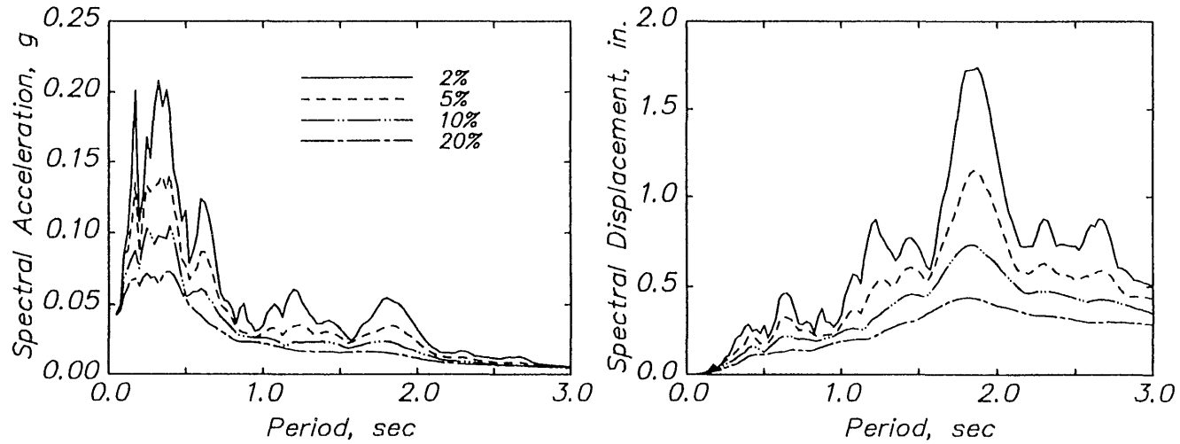
Fig. 5.25 Linear response spectra – Redlands warehouse.
