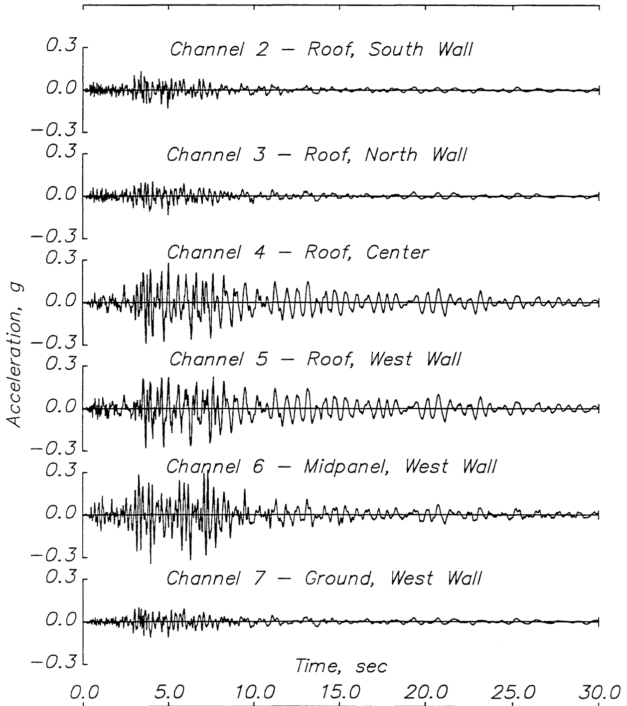
Fig. 5.10 Hollister warehouse – 1986 Hollister earthquake.
