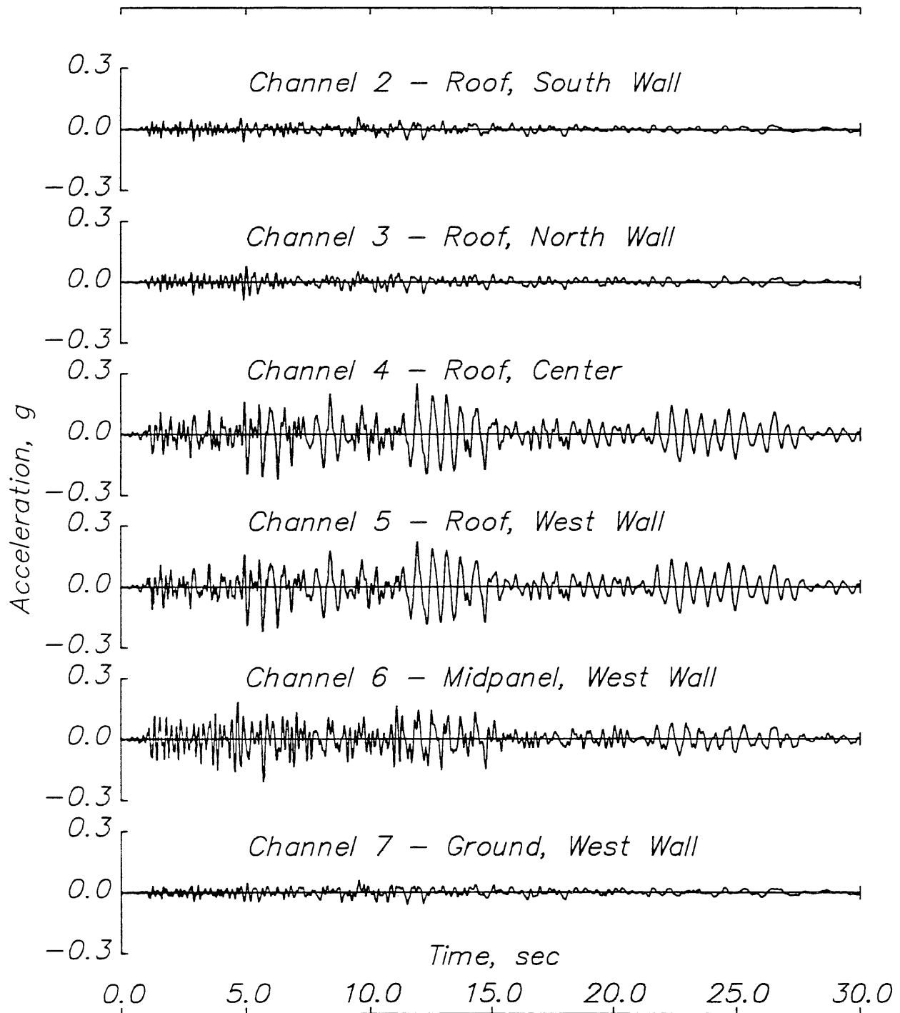
Fig. 5.9 Hollister warehouse – 1984 Morgan Hill earthquake. (a) Transverse acceleration response.
