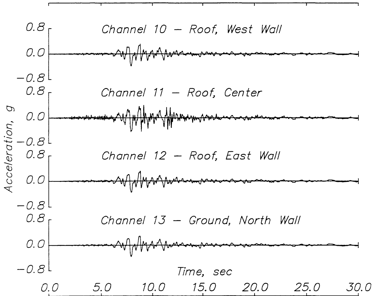
Fig. 5.11 (cont.) Hollister warehouse – 1989 Loma Prieta earthquake. (b) Longitudinal acceleration response.
