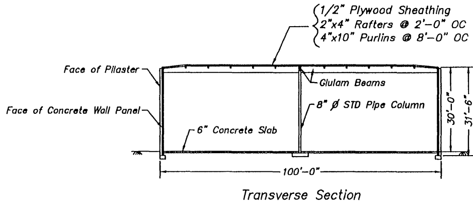
Fig. 5.3 Cross sections – Hollister warehouse.
