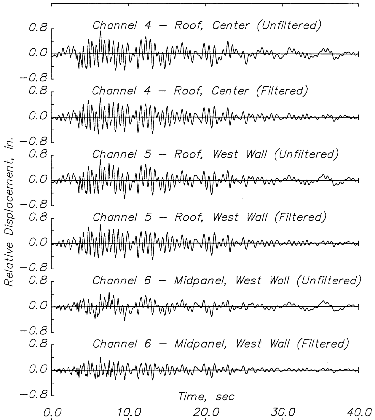
Fig. 5.17 Hollister warehouse – 1986 Hollister earthquake.
