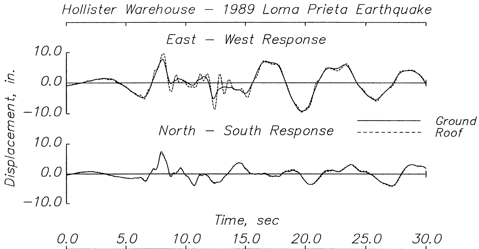
Fig. 5.15 (cont.) Hollister warehouse – Absolute displacement response.
