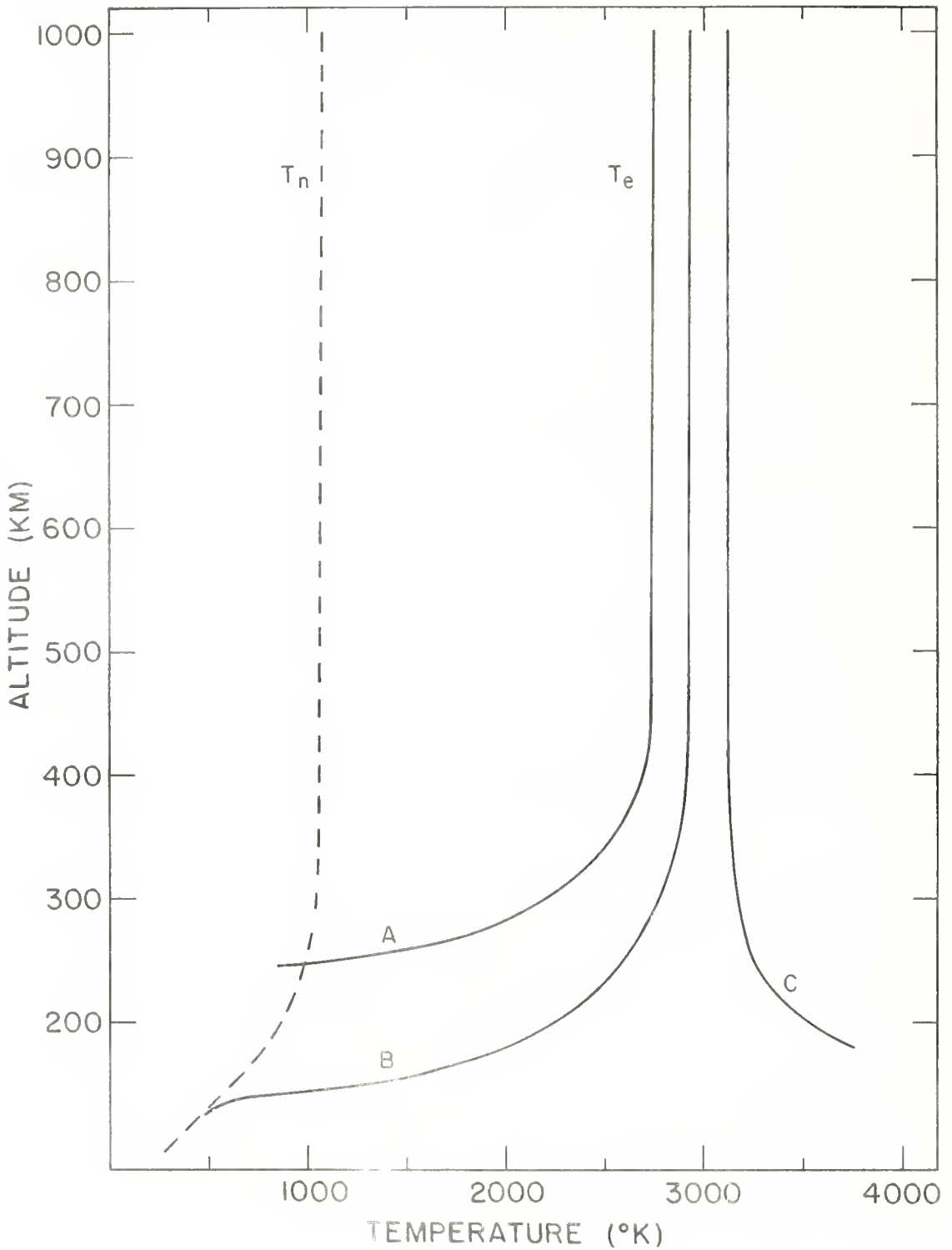
Figure 5.6 Behavior of the trial integrations of Equation (5.36). Profile of the type (A) results when the assumed initial value of T_e at 1000 km is too low, while profile of the type (C) results when this value is too high. Profile (B) is the solution satisfying the lower boundary conditions.
