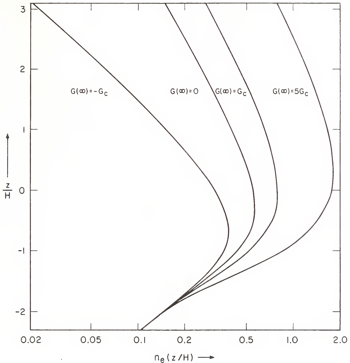
Figure 3.2 The photoaccretive layer distribution for various assumed values of the incoming flux (after Bowhill, 1962b). The curve labeled G(\infty) = -G_c represents the photodepletive layer for the largest possible outgoing flux. The abscissa is electron density divided by the constant factor outside the square brackets in Equation (3.60).
