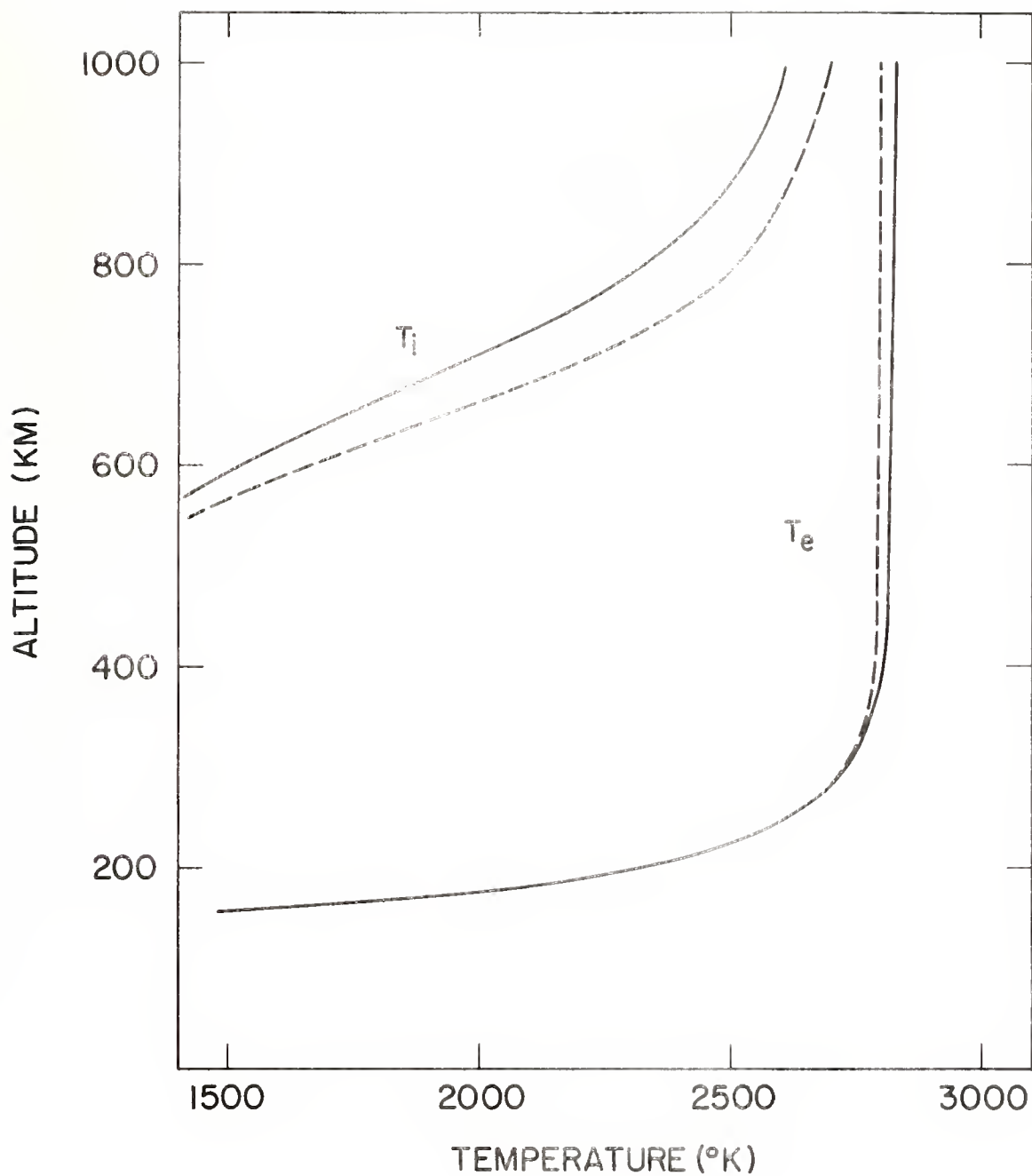
Figure 5.9 The effect on electron and ion temperature profiles of a change in relative abundance of helium ions. Profiles represented by the continuous line are obtained for 20% He + at 700 km; those represented by the broken line are obtained for 0.1% He + at 700 km.
