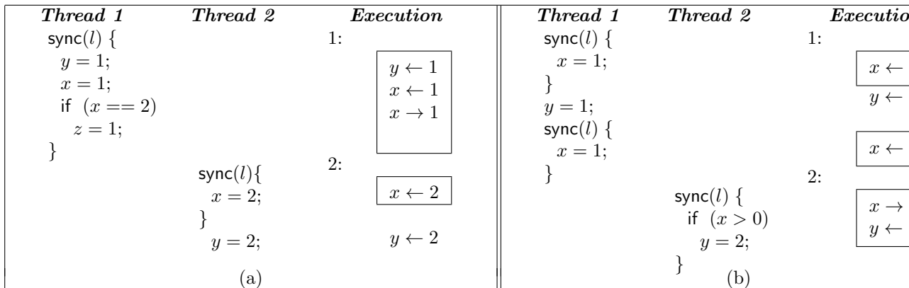
Figure 1: Motivating examples.
