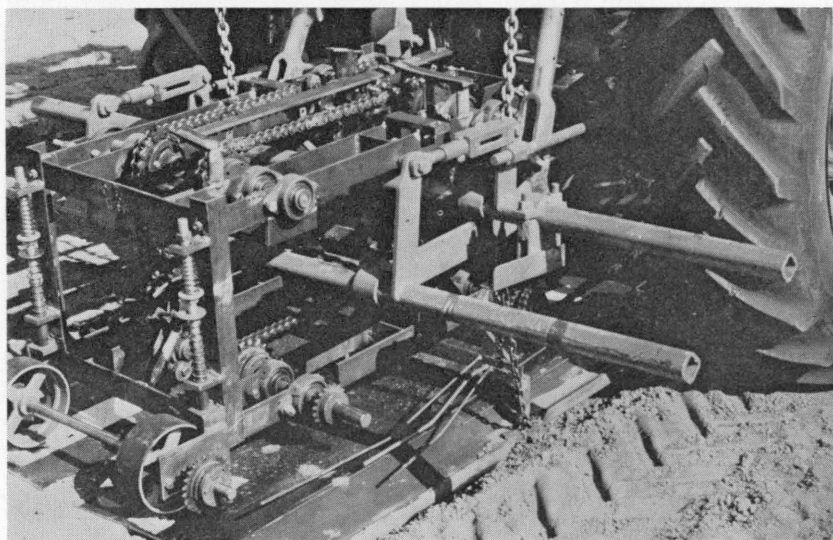
A prototype transplanter attachment for Celluponic mulch-laying machines. (Fig. 14)
