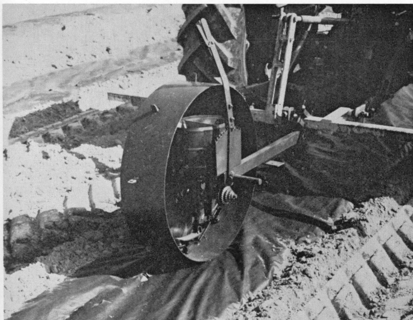
An experimental seeding wheel for paper mulches built by the Department of Agricultural Engineering at the University of Illinois. (Fig. 9)
