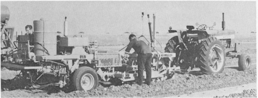
Self-propelled and tractor-drawn prototype mulching machines developed by Celluponic Systems. The machines apply mulch, punch holes in synchronization with a planting mechanism, and spray herbicide along the edge of the mulch. (Fig. 10)
