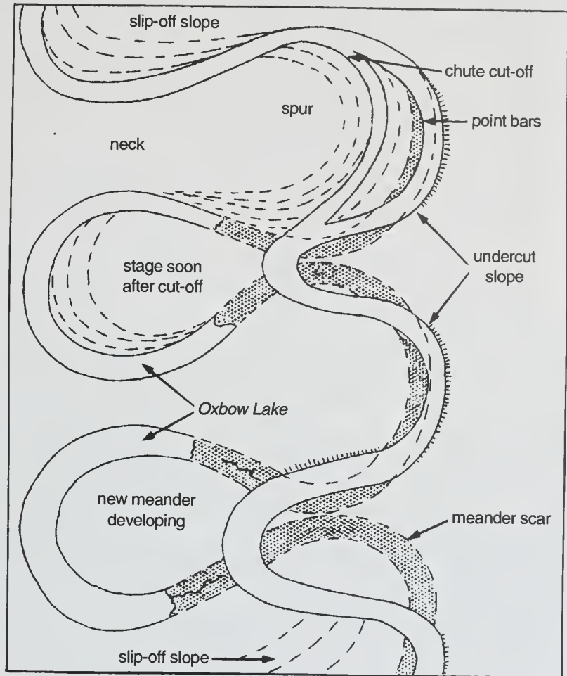
Figure 21 Floodplain features. Water flowing through a meander curve is forced against the outside bank (called the cutbank). As the cutbank is eroded back, the channel migrates in this direction leaving a "slip-off" slope on the inside of the curve. Deposition of material may occur on the slip-off slope in crescent-shaped forms that, when incorporated into the floodplain, become floodplain scrolls. Meanders move across the valley and also downstream. Abandoned meanders generally leave evidence of their existence in the form of meander scars. The area within a meander curve is called a neck. At times of high water, the river may cut off the meander through the neck, leaving a meander core or abandoned meander. If water is left in the cut-off meander, it is called an oxbow lake. When the river cuts through channel bars or point bars, which form on the slip-off slope, a chute cut-off is formed.
