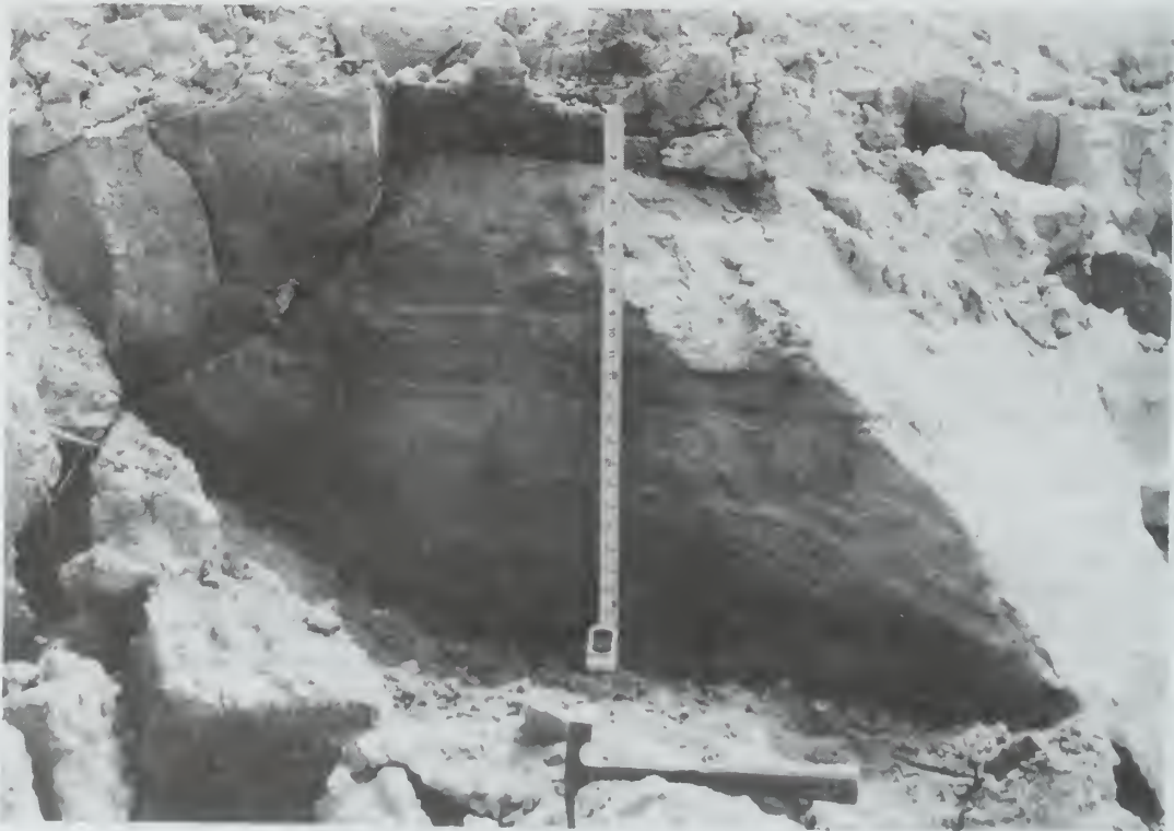
Figure 17 Sand lens with cross bedding in Lake Ancona sediments.
