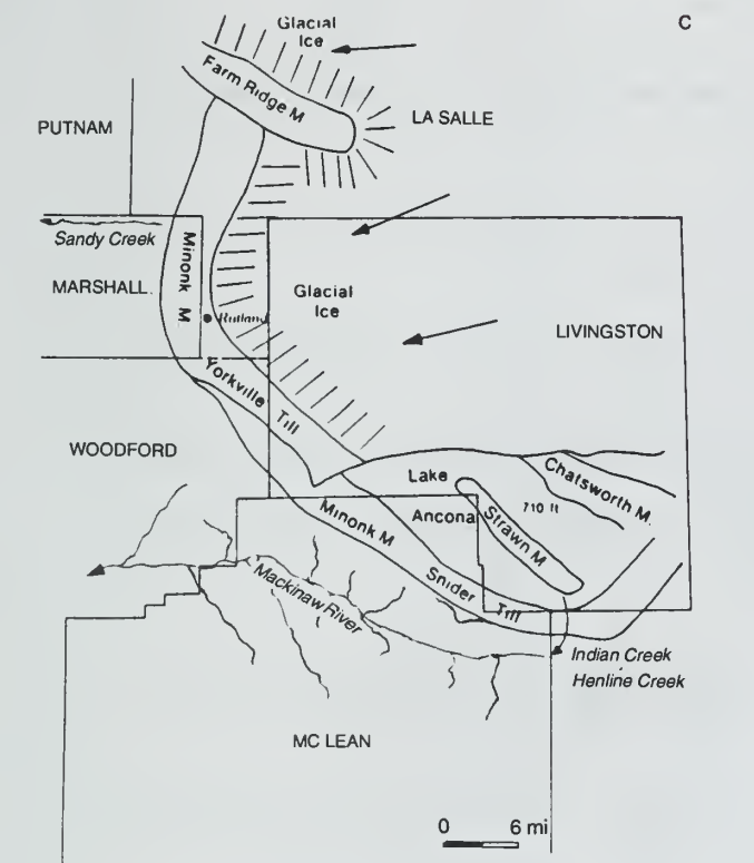
Figure 18 Evolution of Lake Ancona.
