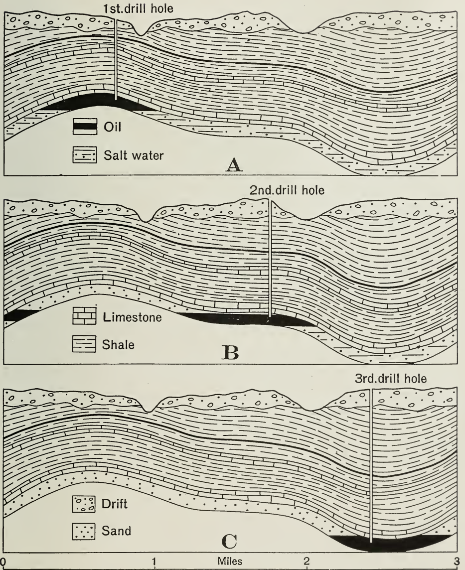
Diagram showing conditions governing oil accumulation
