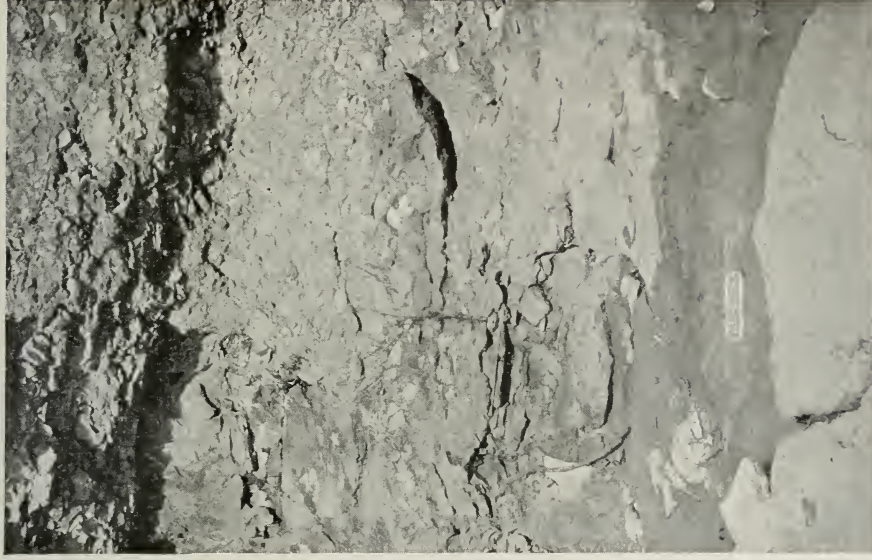
B. Brecciated St. Louis limestone northwest of St. Patrick, Missouri. (See page 43.)
