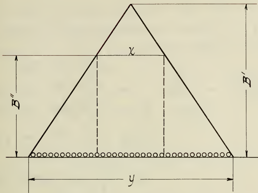
DISTRIBUTED WINDING
