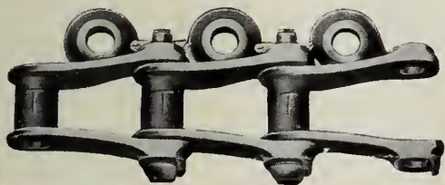
Coke Machine Chain.
