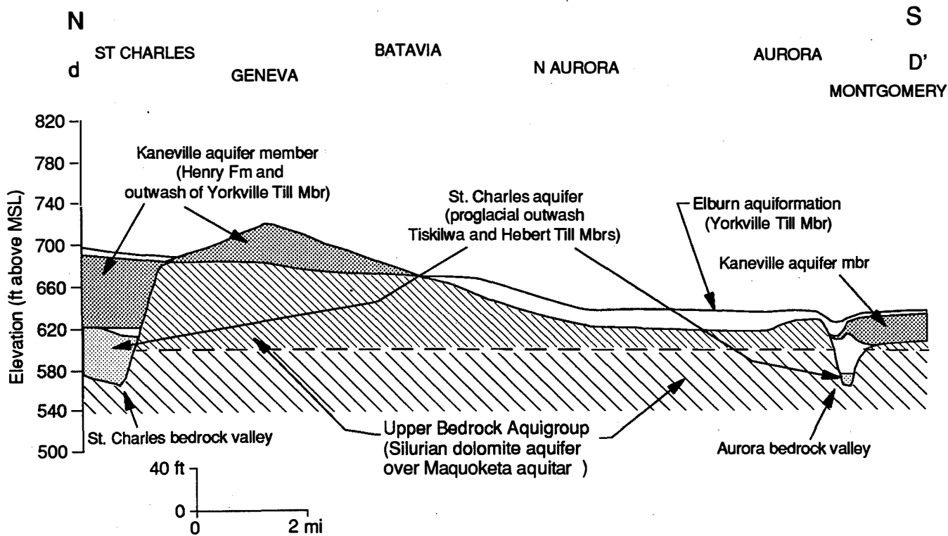
Figure 7d Longitudinal cross section of the Fox River valley from north of Carpentersville to south of Montgomery.
