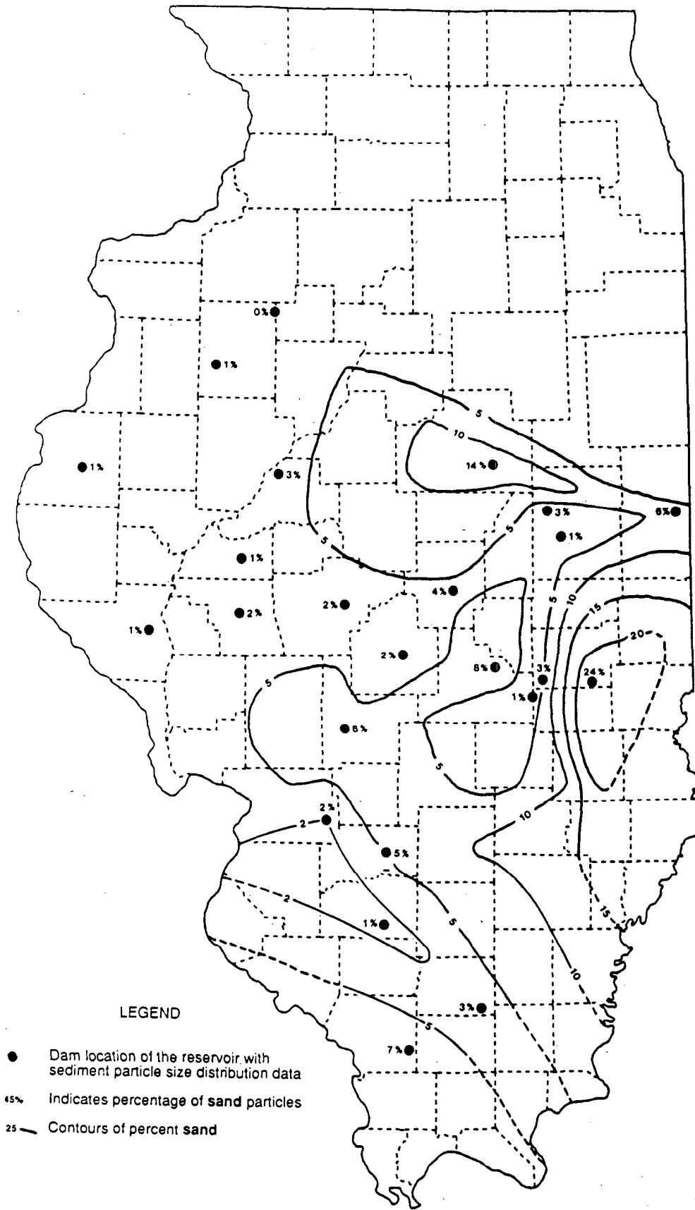
Figure 4. Locations of reservoirs for which sediment particle size analyses have been conducted, and contour map for percent sand distribution
