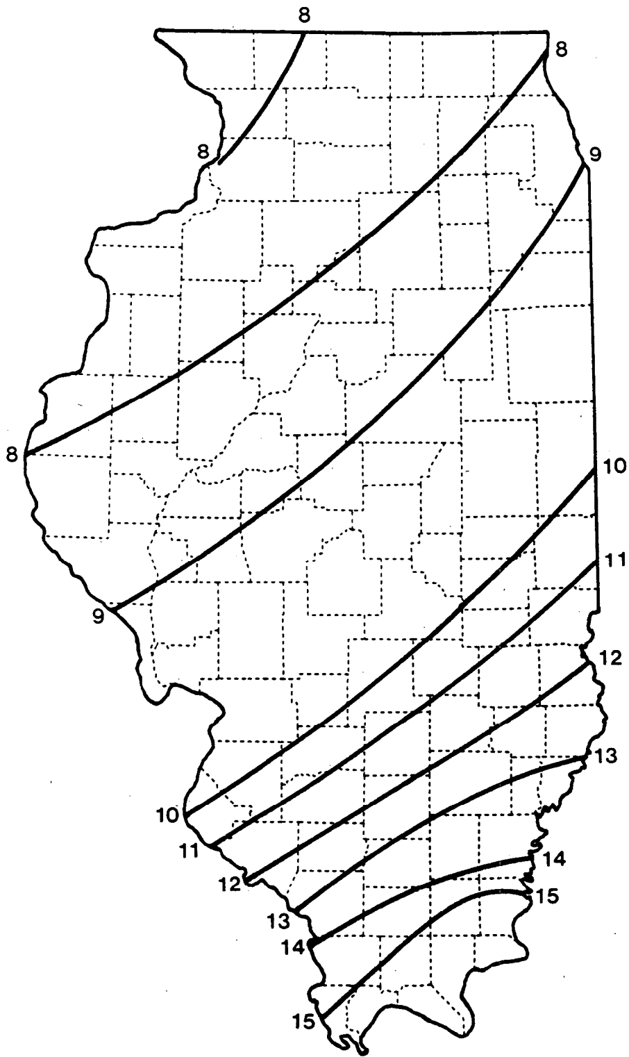
Figure 3. Average annual runoff for Illinois in inches per square mile (from UMRBC, 1970)
