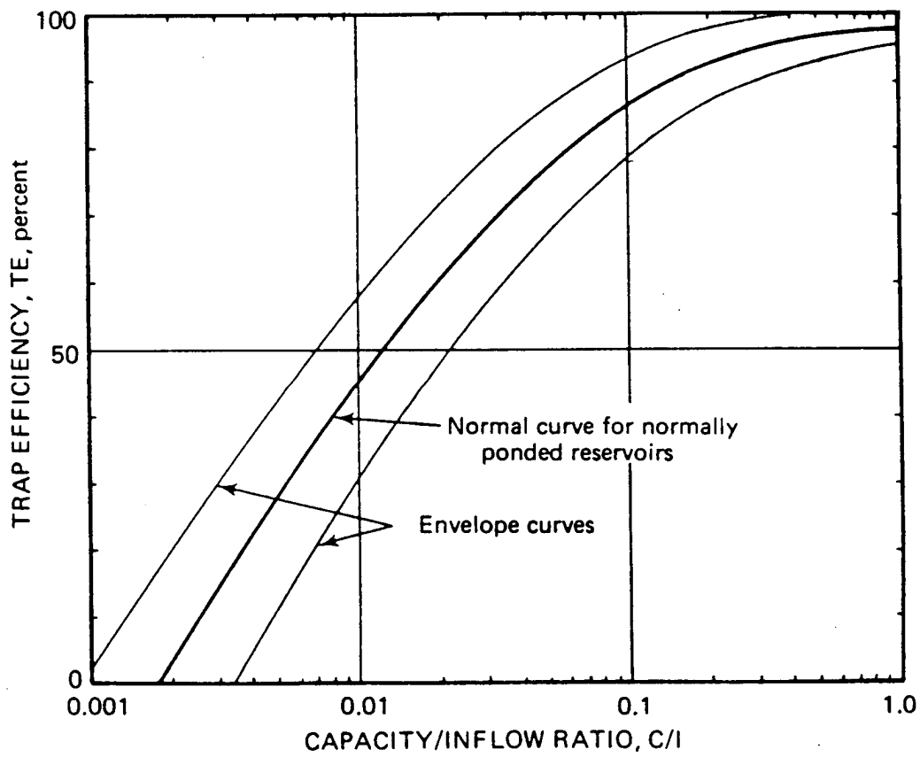
Figure 2. Brune's curve (from Brune, 1953)
